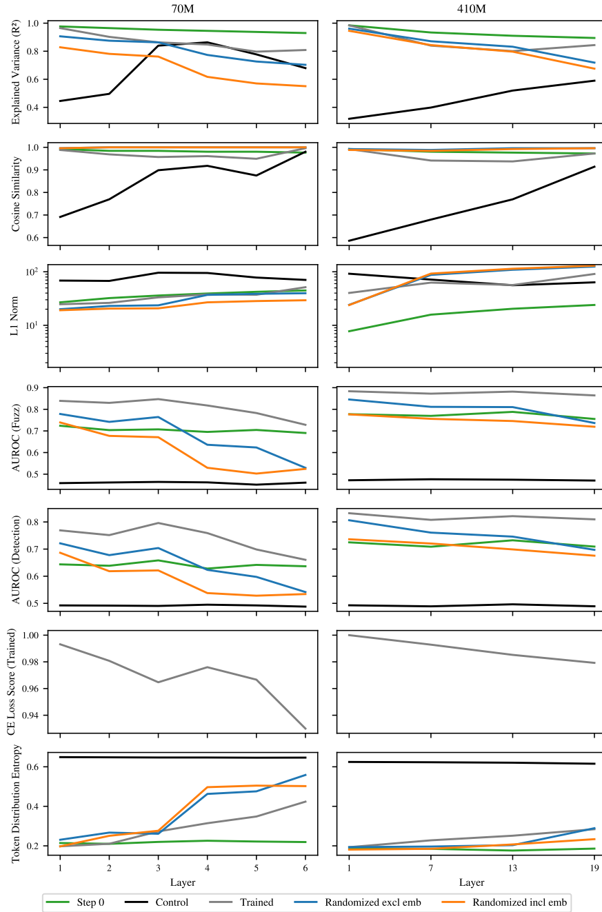
Figure 15: Evaluation metrics for SAEs trained on one billion tokens for the Pythia-70m and 410m models. These panels correspond directly to the matching columns of Figure 2, which reports the same metrics at 100M tokens; the behavior is qualitatively identical, establishing that the ten-fold increase in training data leaves the conclusions intact.
