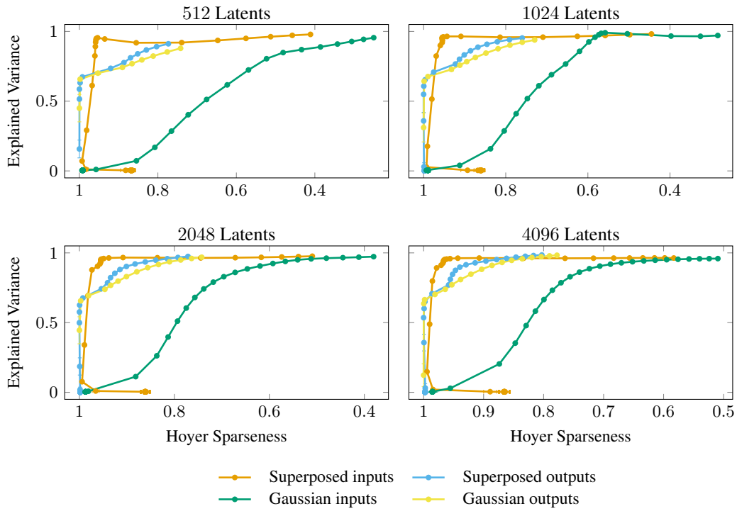
Figure 25: Pareto frontiers of explained variance against sparsity, here measured by the Hoyer sparseness, for toy datasets generated to exhibit superposition, for Gaussian controls matched in mean and variance, and for the corresponding outputs when each is passed through a randomly initialized two-layer MLP. The same ordering of the frontiers holds under this fourth measure, so the conclusion does not depend on the particular sparsity metric.
