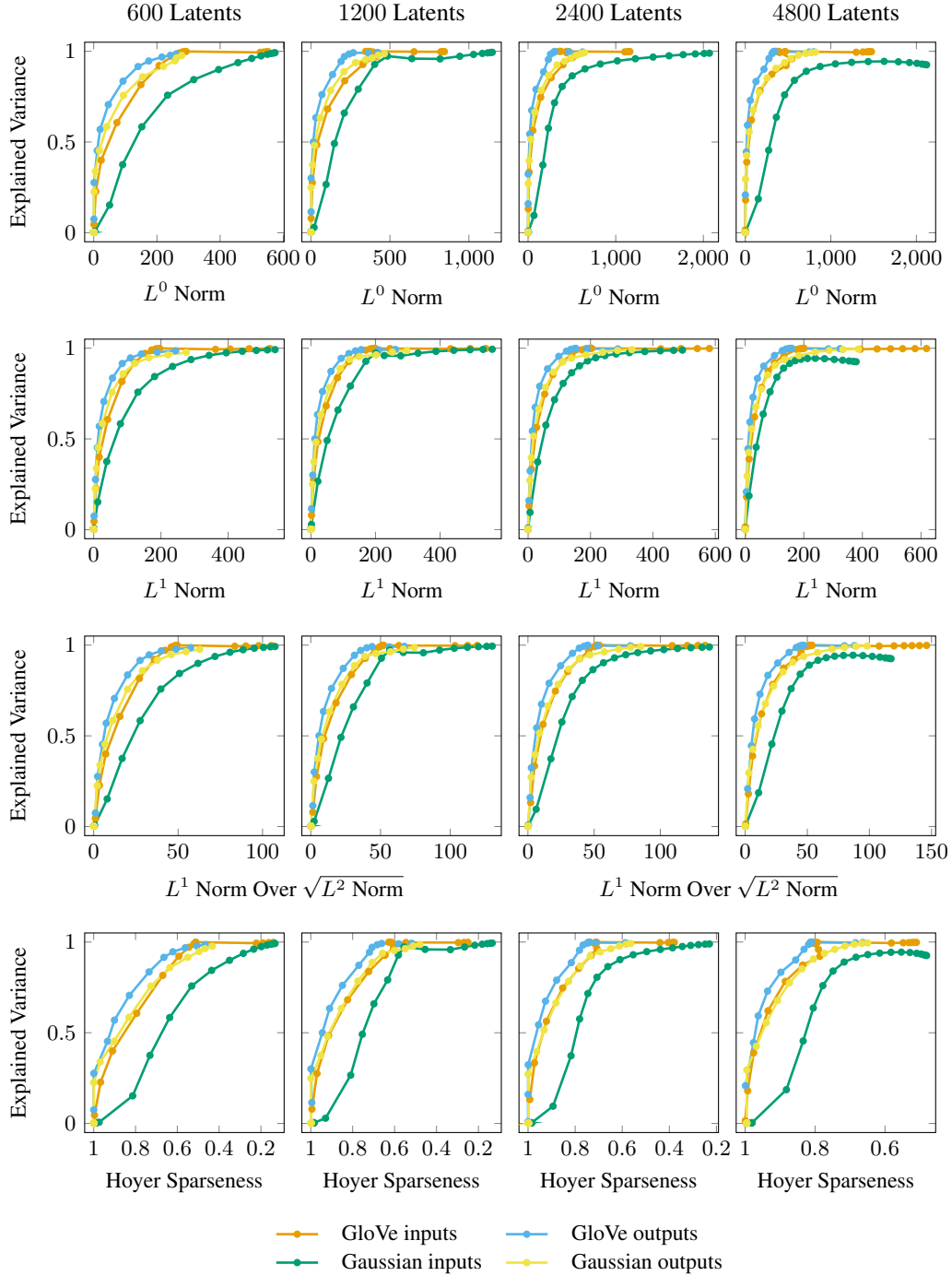
Figure 29: Pareto frontiers of explained variance against several sparsity measures for 300-dimensional GloVe word embeddings, for Gaussian controls matched in mean and variance, and for the corresponding outputs when each is passed through a randomly initialized two-layer MLP. The 300-dimensional case is the one summarized in the main text (Figure 5b); the effect holds across every embedding dimension we examine.
