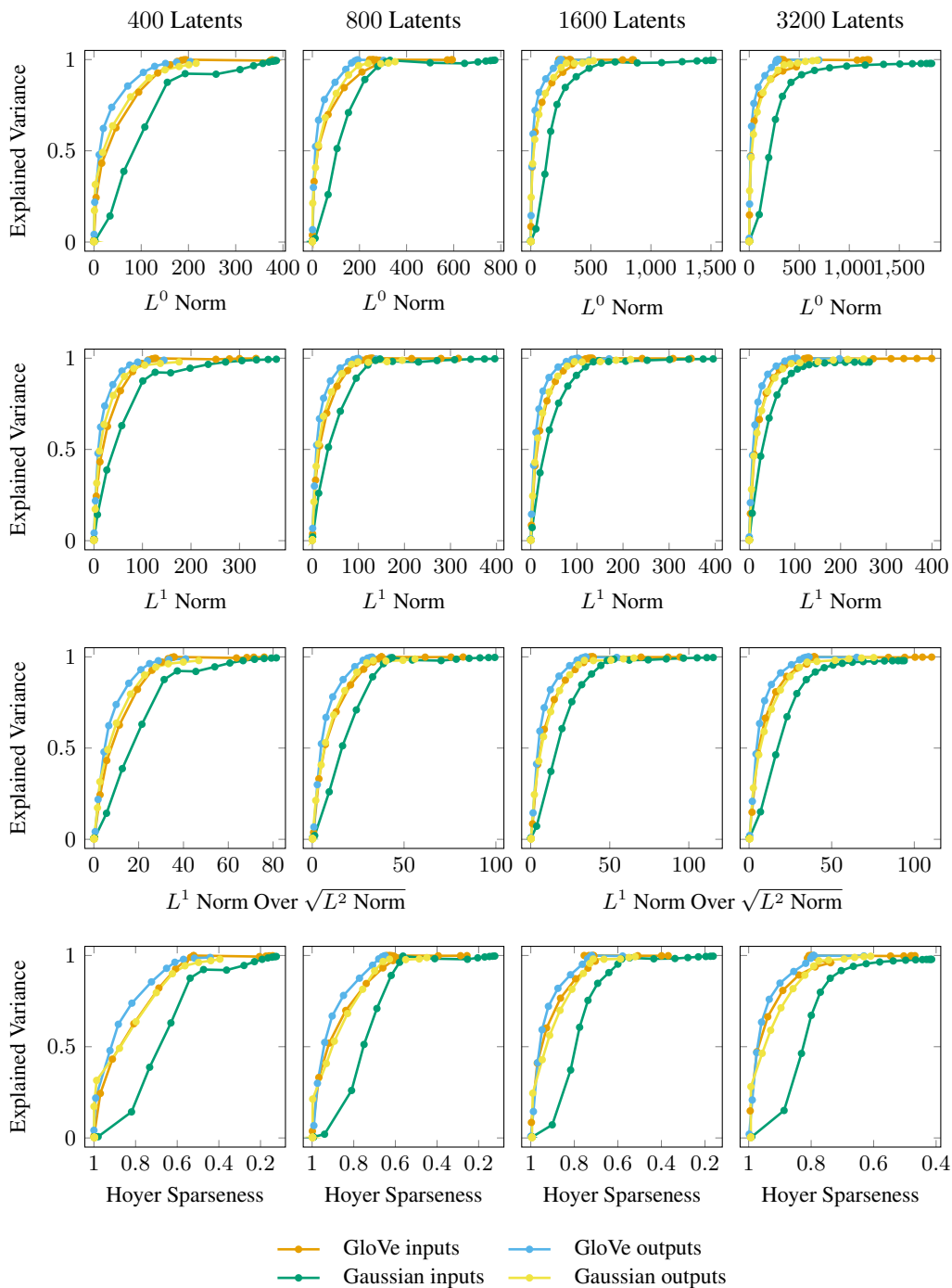
Figure 28: Pareto frontiers of explained variance against several sparsity measures for 200-dimensional GloVe word embeddings, for Gaussian controls matched in mean and variance, and for the corresponding outputs when each is passed through a randomly initialized two-layer MLP. The sparsification effect remains evident at 200 dimensions.
