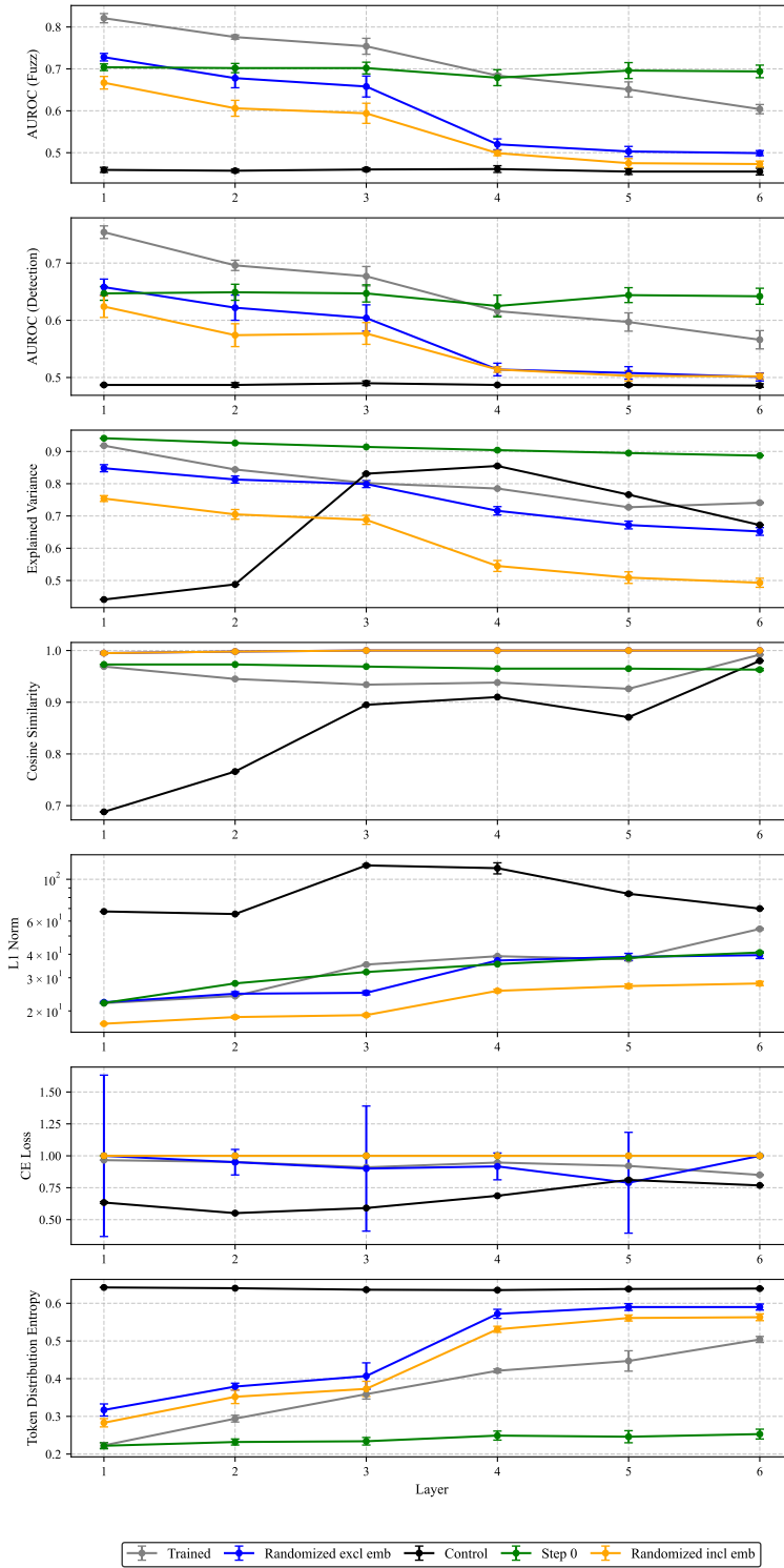
Figure 17: Uncertainty in the Pythia-70m evaluation metrics, computed across five random seeds. The variant orderings established in the main text persist once seed-to-seed variability is accounted for; the reported effects therefore exceed the sampling noise.
