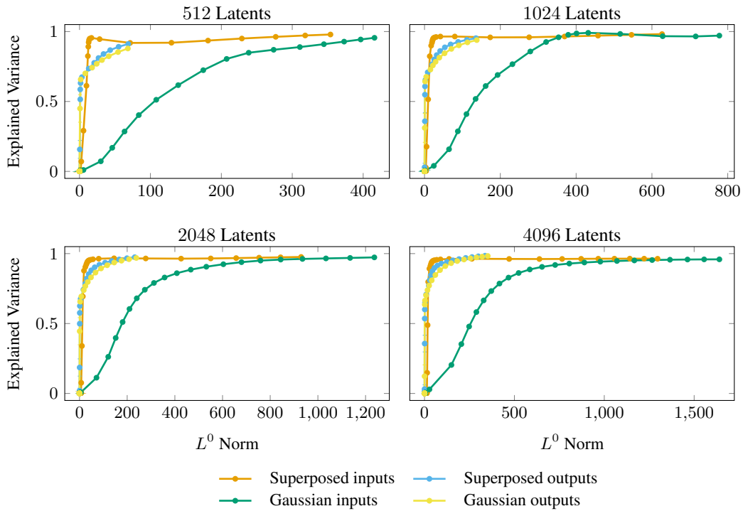
Figure 22: Pareto frontiers of explained variance against sparsity, here measured by the L^0 norm, for toy datasets generated to exhibit superposition, for Gaussian controls matched in mean and variance, and for the corresponding outputs when each is passed through a randomly initialized two-layer MLP. The random MLP shifts the frontier toward greater sparsity under this measure as well.
