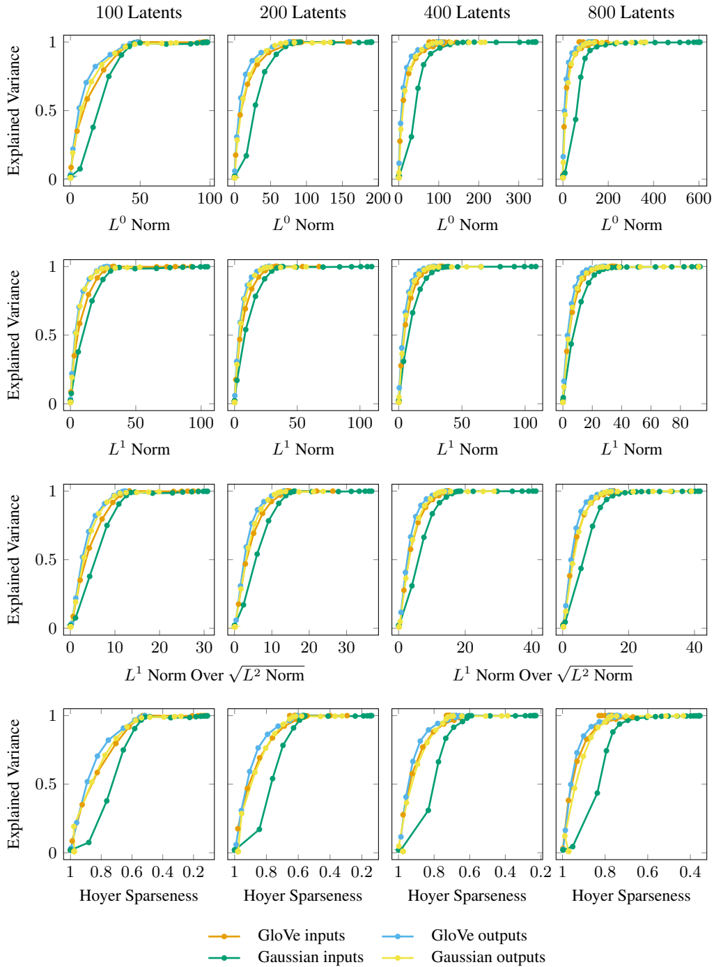
Figure 26: Pareto frontiers of explained variance against several sparsity measures for 50-dimensional GloVe word vectors, for Gaussian controls matched in mean and variance, and for the corresponding outputs when each is passed through a randomly initialized two-layer MLP. Passing the embeddings through the random MLP again increases their apparent sparsity.
