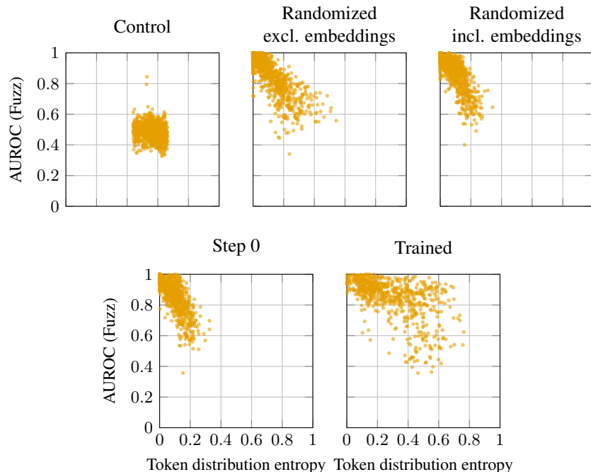
Figure 20: Per-latent token-distribution entropy against ‘fuzzing’ AUROC (auto-interpretability score) for SAEs trained on multiple layers of Pythia-6.9b. Each point is a single latent drawn from the same sample used to compute the aggregate metrics of Figures 1 and 2. Disaggregating to the latent level exposes structure that the aggregate scores conceal: the trained and randomized variants occupy visibly different regions of the entropy–AUROC plane even where their aggregate scores coincide.
