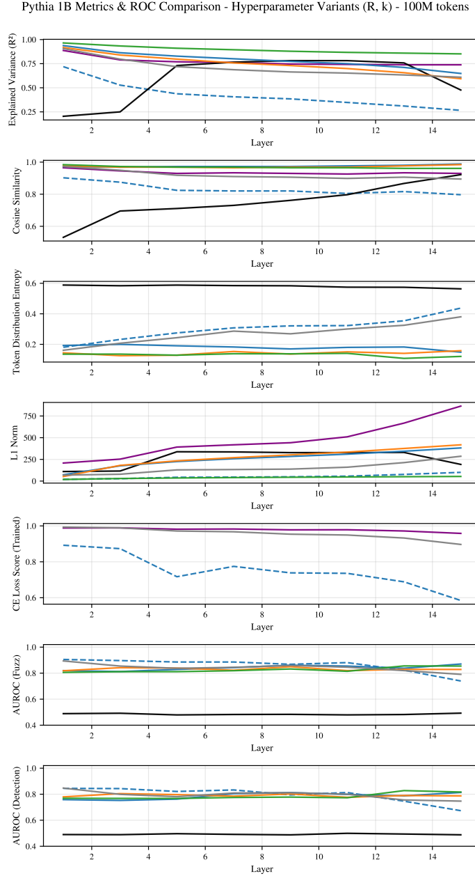
Figure 19: Evaluation metrics for SAEs trained on Pythia-1b under varying hyperparameters, alongside the main results from Figure 2. SAEs with a very small expansion factor R = 2 and sparsity k = 4 are clearly separated from our default configuration by explained variance and CE loss score. Even under this deliberately degraded configuration, their auto-interpretability scores remain close to those of the default-hyperparameter SAEs on both trained and randomized models—further evidence that the trained-versus-randomized similarity is a property of the auto-interpretability metric itself rather than an artifact of the hyperparameter choice.
