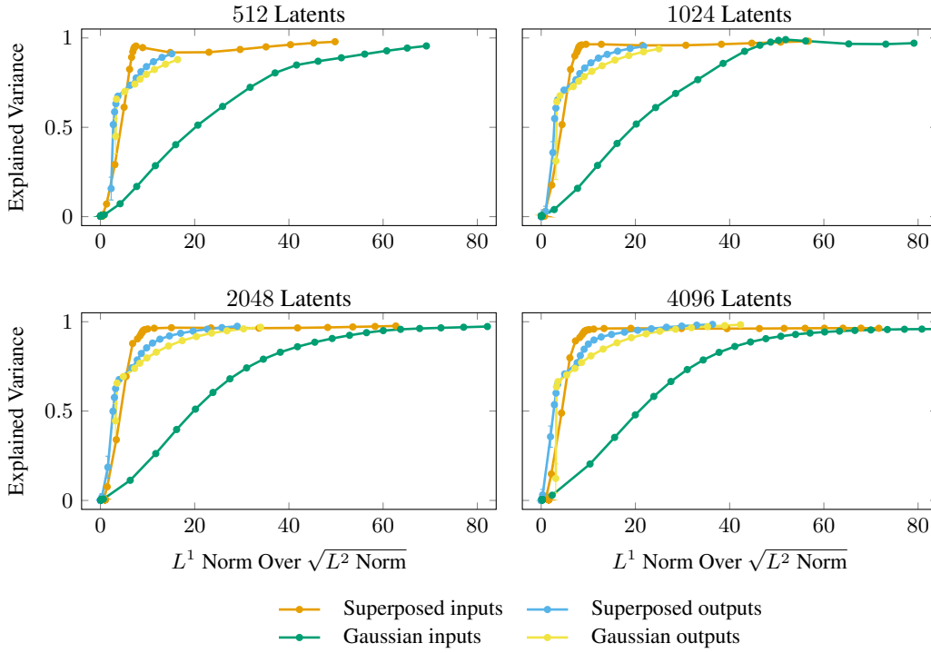
Figure 24: Pareto frontiers of explained variance against sparsity, here measured by the L^1 norm divided by the square root of the L^2 norm, for toy datasets generated to exhibit superposition, for Gaussian controls matched in mean and variance, and for the corresponding outputs when each is passed through a randomly initialized two-layer MLP. This is the scale-invariant sparsity measure reported in the main text (Figure 5a).
