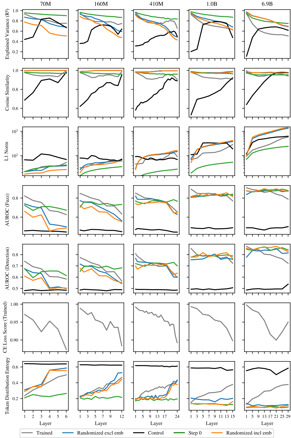
Figure 2: SAE metrics across Pythia model sizes (70M to 6.9B parameters). The contribution highlighted by this comparison is that trained and randomized variants often follow similar trends across scale, while the control is more clearly separated. Larger models show more consistent behavior across layers, and all non-control variants can achieve comparable metric values despite different initialization histories.
