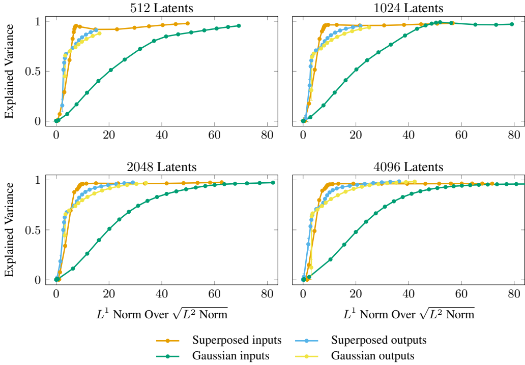
Figure 24: Toy-model Pareto frontiers of explained variance against the L^1 norm over the square root of the L^2 norm. This sparsity measure shows how synthetic superposed data, matched Gaussian controls, and random-MLP outputs compare.
