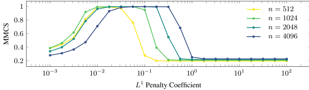
Figure 4: Ground-truth recovery check for the toy-model contribution. The plot shows mean max cosine similarity (MMCS) between standard-SAE decoder weight vectors and data-generating features as the L^1 penalty coefficient varies, following Sharkey et al. (2022). The ‘Goldilocks zone’ confirms that SAEs can nearly recover the data-generating features when enough latents are available.
