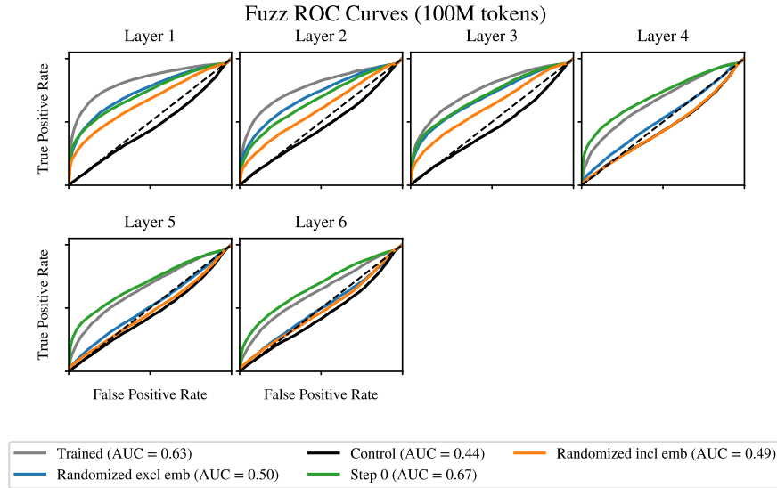
Figure 6: Pythia-70m ‘fuzzing’ auto-interpretability over 100 SAE latents. This appendix panel supports the main contribution by showing how trained and randomized variants compare across layers, including the overall degradation in performance as layer index increases.
