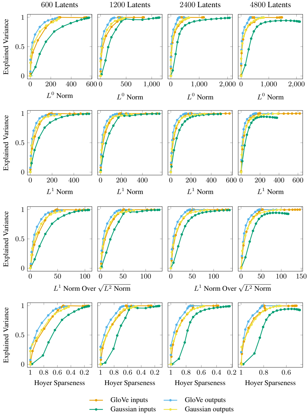
Figure 29: Language-vector superposition check for 300-dimensional GloVe word embeddings. Pareto frontiers compare embeddings, matched Gaussian controls, and outputs after a randomly initialized two-layer MLP.
