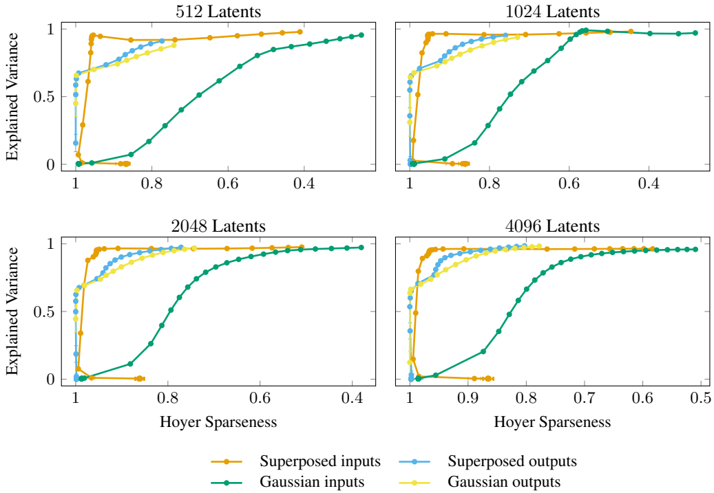
Figure 25: Toy-model Pareto frontiers of explained variance against Hoyer sparseness. The comparison again separates synthetic superposed data, matched Gaussian controls, and outputs from a randomly initialized two-layer MLP.
