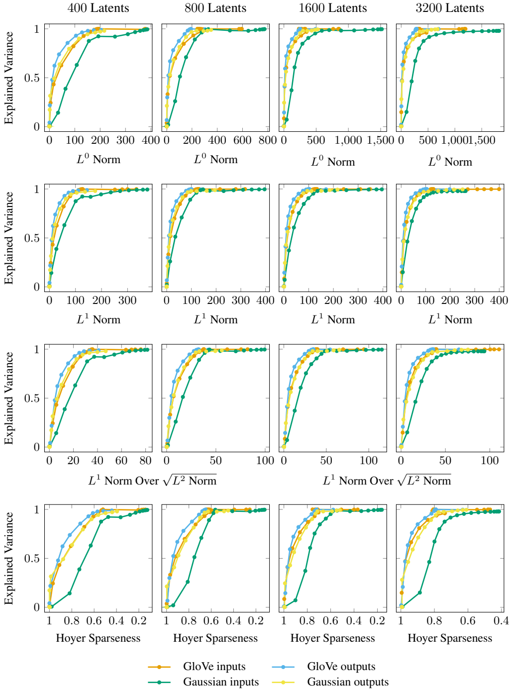
Figure 28: Language-vector superposition check for 200-dimensional GloVe word embeddings. Pareto frontiers compare embeddings, matched Gaussian controls, and outputs after a randomly initialized two-layer MLP.
