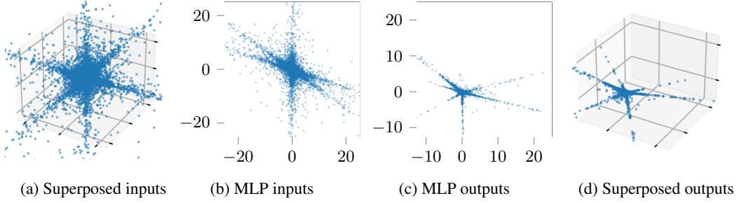
Figure 3: Illustrating mechanism one: a randomly initialized network preserves (and appears to sharpen) superposition in its input. We draw 10K samples of n_s = 3 sparse input features from a Lomax distribution with shape \alpha = 1 and scale \lambda = 1 , project them to n_d = 2 dense input features by an i.i.d. standard normal matrix, pass the result through a two-layer ReLU MLP with hidden size 4n_d , and recover n_s = 3 sparse outputs via the inverse of that projection matrix. The superposed structure survives the nonlinearity, foreshadowing the amplification we test next.
