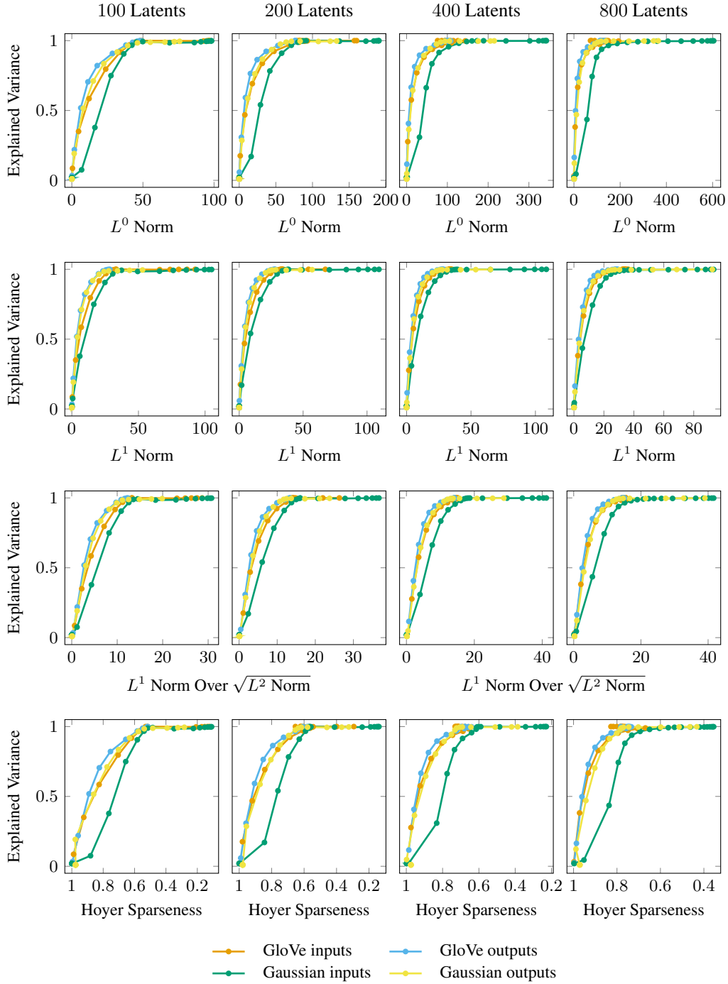
Figure 26: The embedding-superposition result at 50 dimensions. Pareto frontiers of explained variance against sparsity measures for 50-dimensional GloVe word vectors, Gaussian controls with matched mean and variance, and the corresponding outputs after a randomly initialized two-layer MLP.
