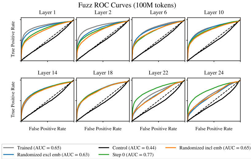
Figure 10: ‘Fuzzing’ auto-interpretability ROC curves for Pythia-410m over 100 SAE latents. The variants perform similarly and degrade overall with layer index; here, too, the auto-interpretability scores fail to distinguish trained from randomized models – our central finding.
