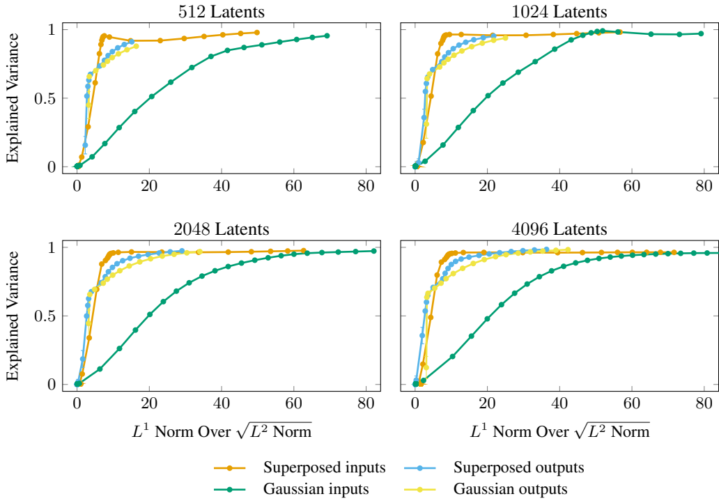
Figure 24: And under the L^1/\sqrt{L^2} sparsity measure used in the main text. Pareto frontiers of explained variance against the L^1 norm over the square root of the L^2 norm for toy datasets generated to exhibit superposition, Gaussian controls with matched mean and variance, and the corresponding outputs after a randomly initialized two-layer MLP.
