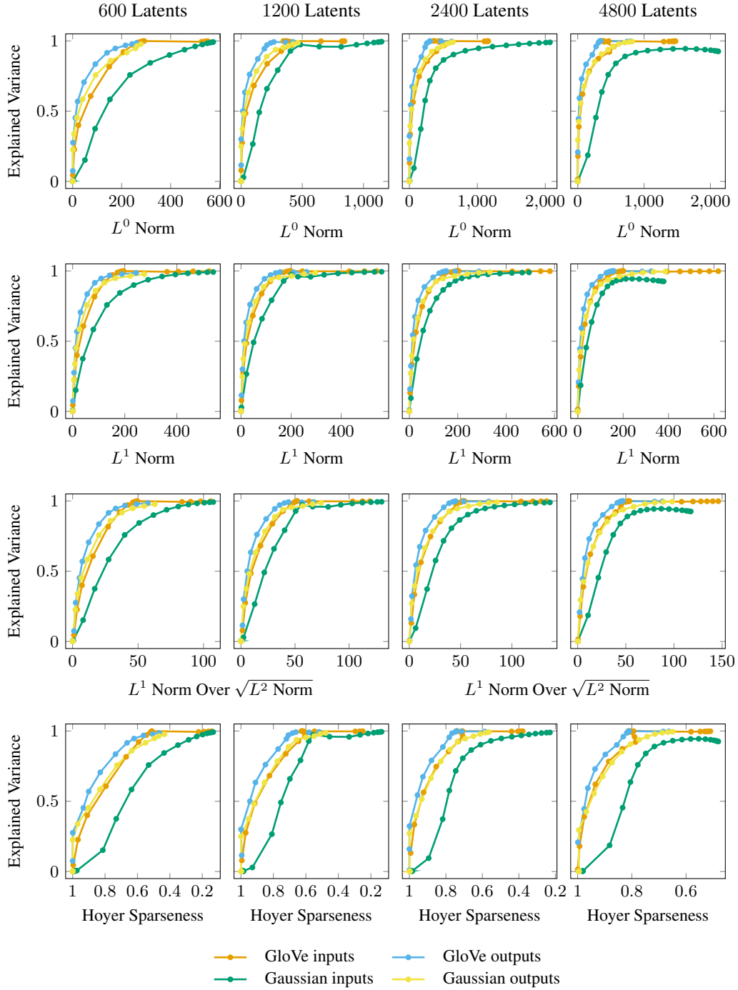
Figure 29: And at 300 dimensions, matching the main-text panel. Pareto frontiers of explained variance against sparsity measures for 300-dimensional GloVe word embeddings, Gaussian controls with matched mean and variance, and the corresponding outputs after a randomly initialized two-layer MLP.
