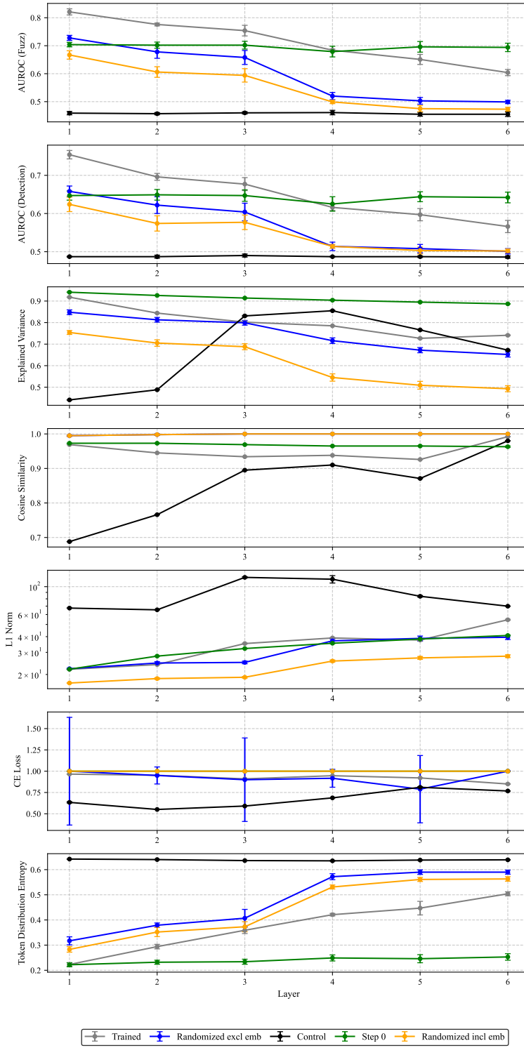
Figure 17: Uncertainty in the Pythia-70m metrics across five random seeds; the variability is small relative to the trained-vs-randomized gaps we report, so our central finding is robust to seed choice.
