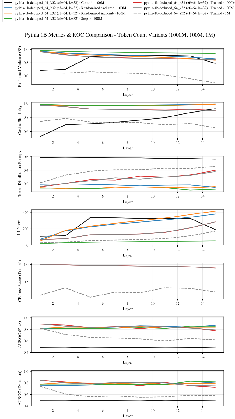
Figure 16: At the opposite extreme, severe under-training degrades reconstruction but not our qualitative story: evaluation metrics for SAEs trained on 1M and 1B tokens for Pythia-1b. Explained variance and CE loss score are much lower for the 1M model, confirming it is under-trained; average auto-interpretability scores are slightly lower at the earliest layers and decline sharply with layer. The trends in auto-interpretability and token-distribution entropy with layer index remain consistent with the other SAEs.
