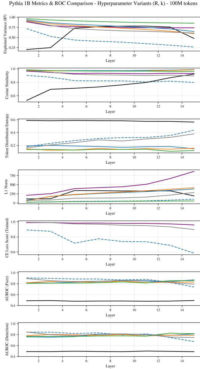
Figure 19: Hyperparameter comparison for Pythia-1b SAEs, including the default setting from Figure 2. A very small SAE ( R = 2, k = 4 ) is clearly worse on explained variance and CE loss score, but its auto-interpretability scores remain close to those of default-hyperparameter SAEs trained on either trained or randomized models.
