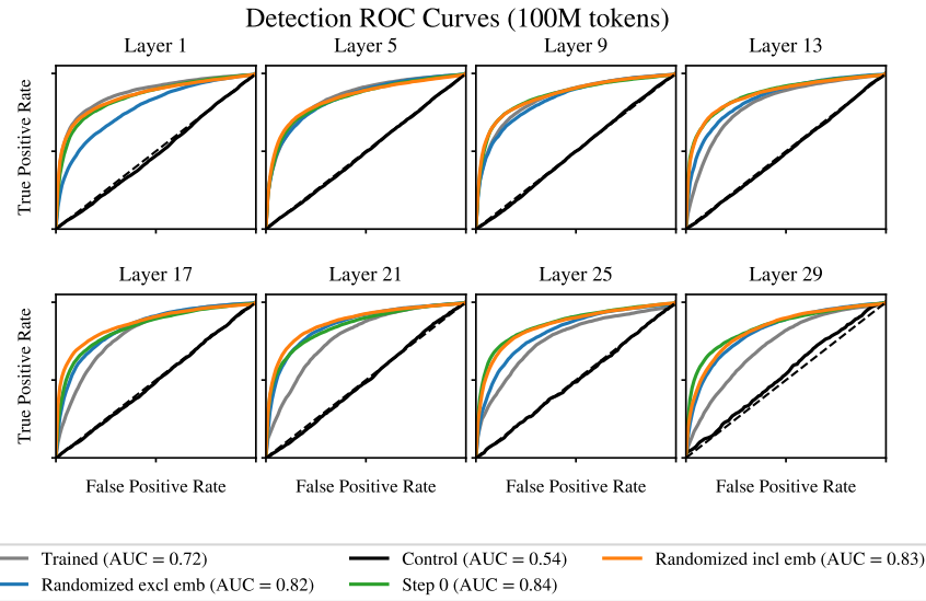
Figure 14: Layer-wise ‘detection’ AUROC for Pythia-6.9b using 100 sampled SAE latents per variant. As in the ‘fuzzing’ results, trained and randomized variants occupy similar score ranges.
