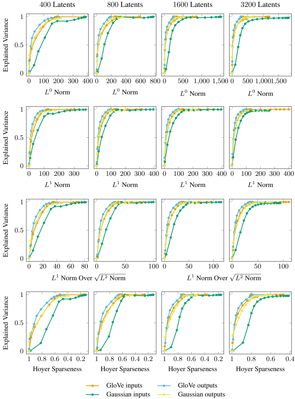
Figure 28: Pareto-frontier comparison for 200-dimensional GloVe word embeddings, matched Gaussian controls, and their random-MLP outputs. The curves make the input-control and output-control sparsity margins directly comparable.
