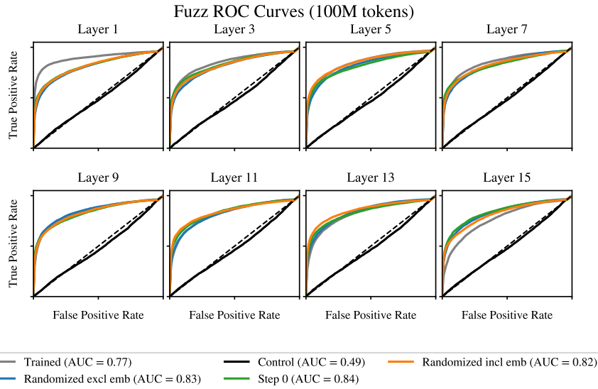
Figure 12: Layer-wise ‘fuzzing’ AUROC for Pythia-1b using 100 sampled SAE latents per variant. The trained and randomized curves remain close, and unlike smaller models there is no clear overall degradation with layer index.
