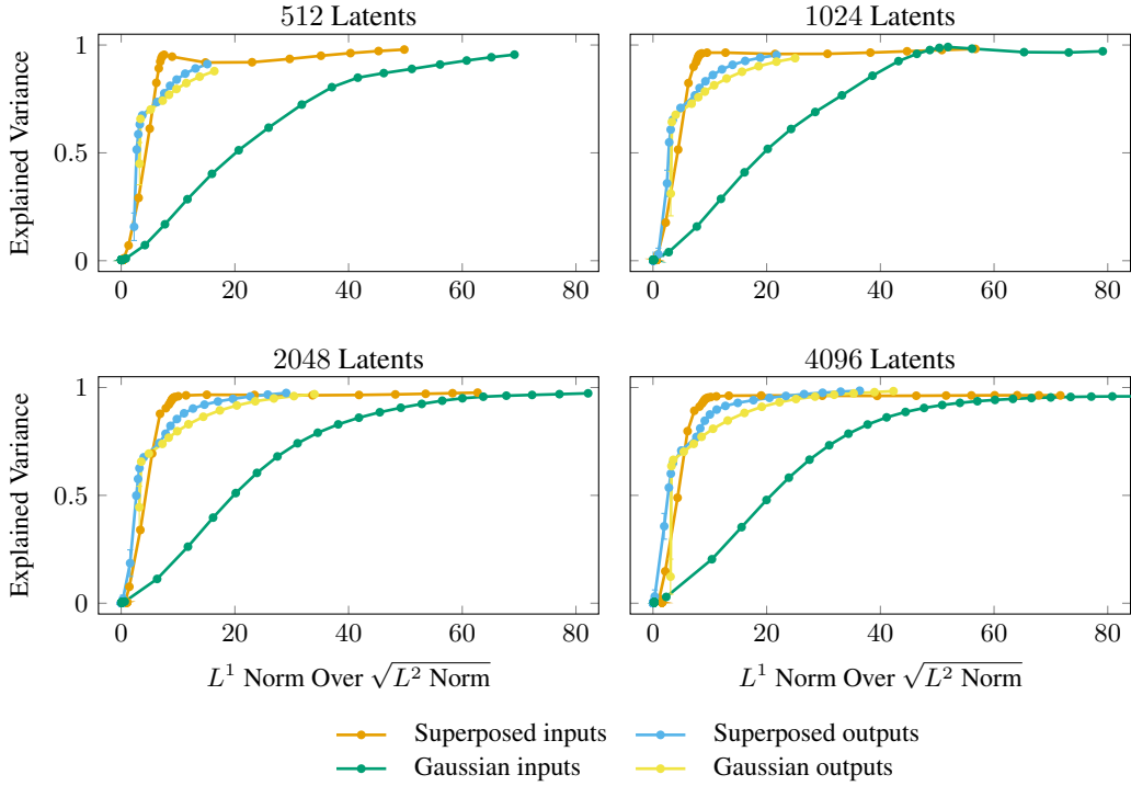
Figure 24: Toy-data Pareto frontiers comparing explained variance with L^1/\sqrt{L^2} sparsity for superposed inputs, matched Gaussian controls, and the corresponding random-MLP outputs. The frontier gaps summarize the empirical sparsity advantage of each condition.
