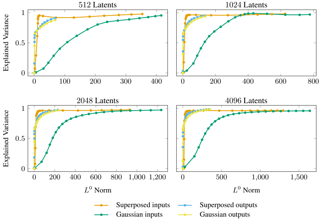
Figure 22: Toy-data Pareto frontiers comparing explained variance with L^0 sparsity for superposed inputs, matched Gaussian controls, and the corresponding random-MLP outputs. The plot exposes sparsity margins at matched reconstruction quality.
