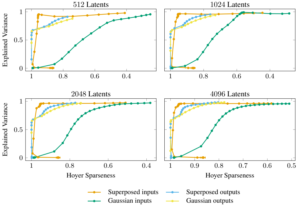
Figure 25: Toy-data Pareto frontiers comparing explained variance with Hoyer sparseness for superposed inputs, matched Gaussian controls, and the corresponding random-MLP outputs. This alternative sparsity metric checks that the qualitative frontier pattern is not metric-specific.
