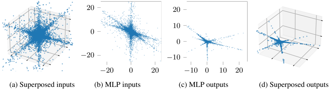
Figure 3: Illustrative comparison of sparse inputs, dense projections, and outputs from a randomly initialized neural network. We sample 10K points with n_s = 3 sparse input features from a Lomax distribution with shape \alpha = 1 and scale \lambda = 1 , then project them to n_d = 2 dense input features using an i.i.d. standard normal matrix. Passing the dense inputs through a two-layer ReLU MLP with hidden size 4n_d and mapping back with the inverse projection preserves the visible sparse structure, providing a qualitative example of how random networks can maintain or sharpen superposition.
