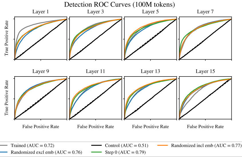
Figure 13: Layer-wise ‘detection’ AUROC for Pythia-1b using 100 sampled SAE latents per variant. The comparison again shows small trained–randomized margins without a clear layer-wise quality decline.
