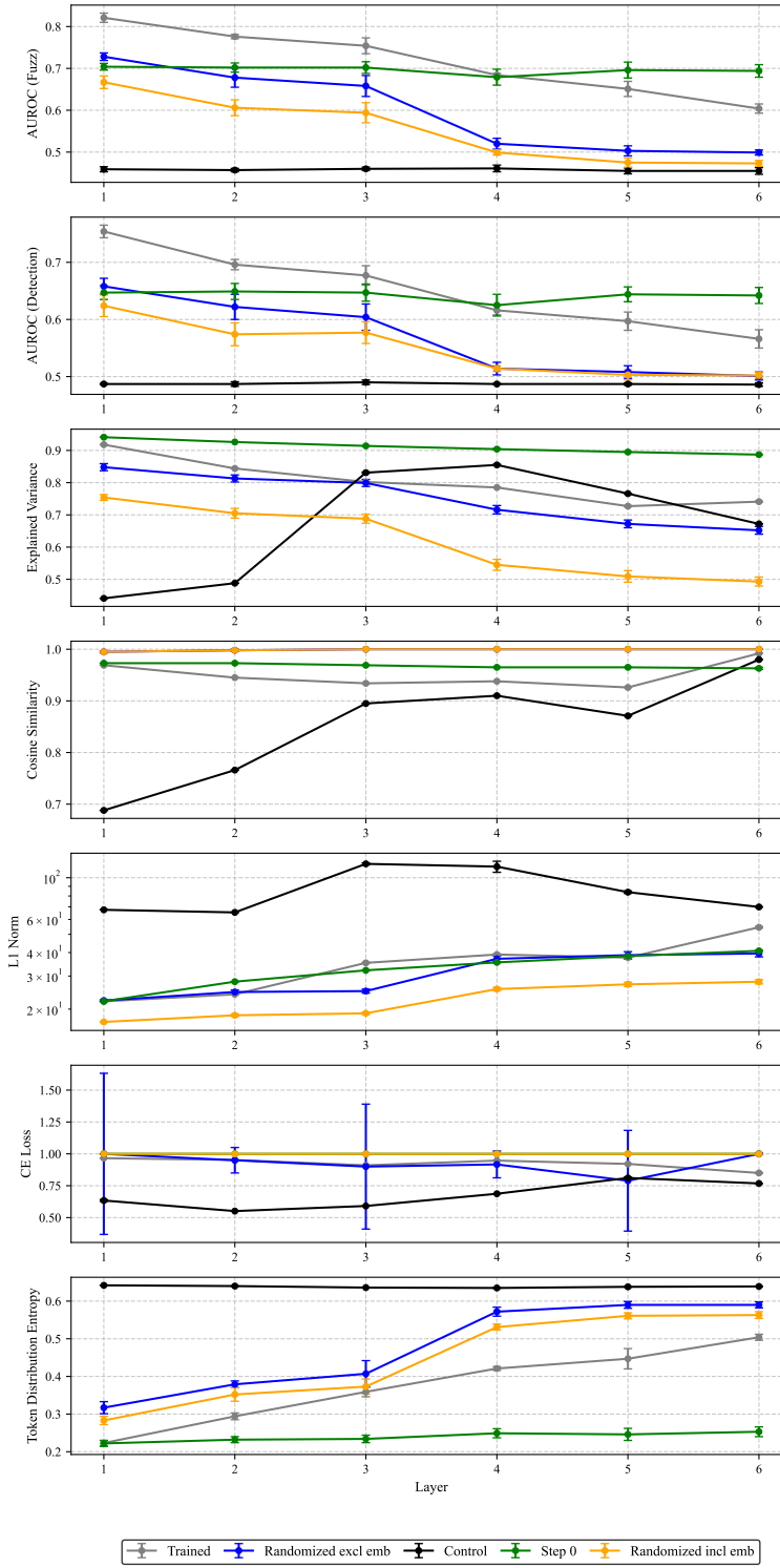
Figure 17: Uncertainty estimates for Pythia-70m metrics computed over five random seeds, showing the stability of the trained, randomized, and control comparisons.
