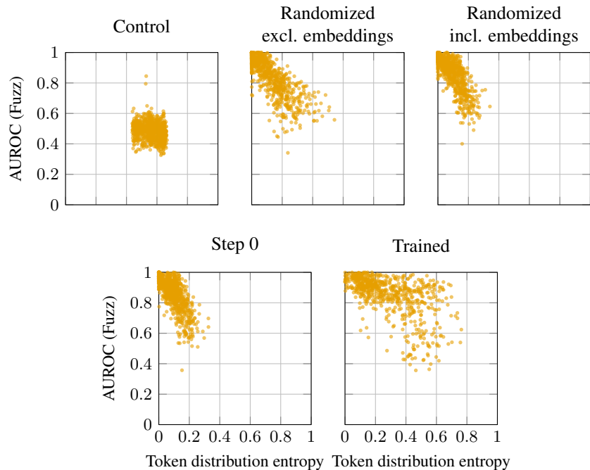
Figure 20: Per-latent token-distribution entropy versus ‘fuzzing’ AUROC for SAEs across multiple layers of Pythia-6.9b. Each point is a single latent, drawn from the same sample used for the aggregate metrics in Figures 1 and 2. Whereas the aggregate scores gave near-identical numbers across variants, the joint entropy–AUROC distribution pulls the variants apart: only the trained variant populates the high-entropy, high-AUROC region.
