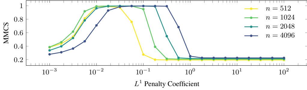
Figure 4: Mean max cosine similarity (MMCS) between the SAE’s learned features (decoder weight vectors) and the data-generating features, as a function of the L^1 penalty coefficient in the training loss, following Sharkey et al. (2022). Across an intermediate ‘Goldilocks zone’ of penalty coefficients, MMCS approaches its ceiling—i.e., the SAE recovers the data-generating features almost perfectly—provided there are enough latents to represent them.
