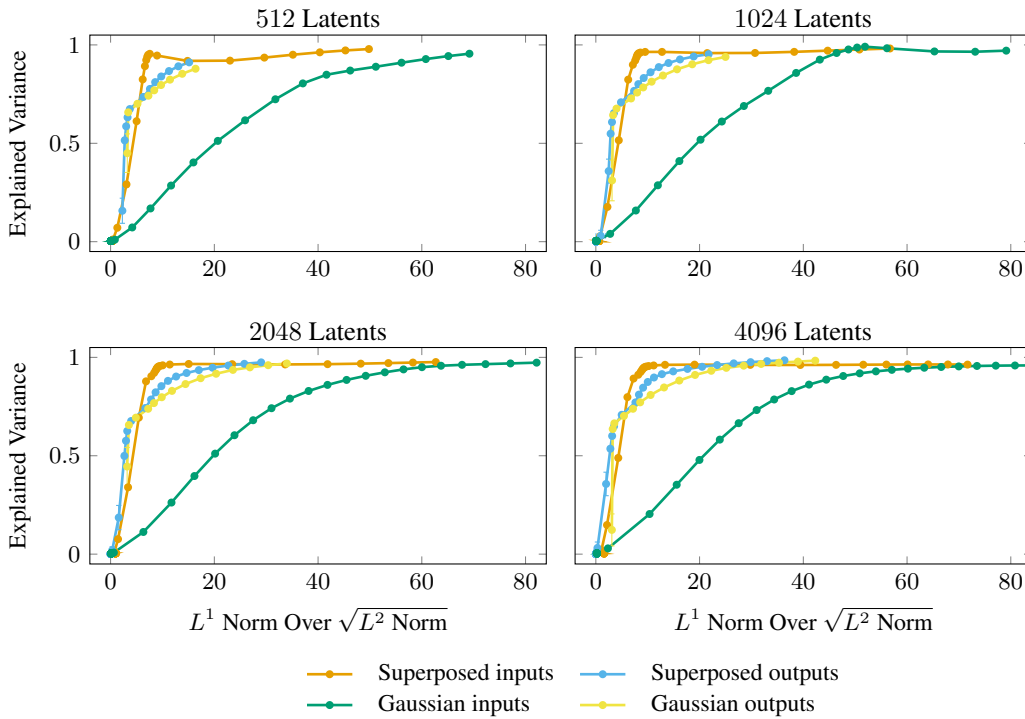
Figure 24: Explained-variance-vs- L^1/\sqrt{L^2} (sparsity) Pareto frontiers comparing toy datasets generated to exhibit superposition, matched Gaussian controls with the same mean and variance, and the corresponding outputs after a randomly initialized two-layer MLP. This is the full-page version of the comparison summarized in Figure 5a, again showing a wide input-side gap that all but disappears at the output.
