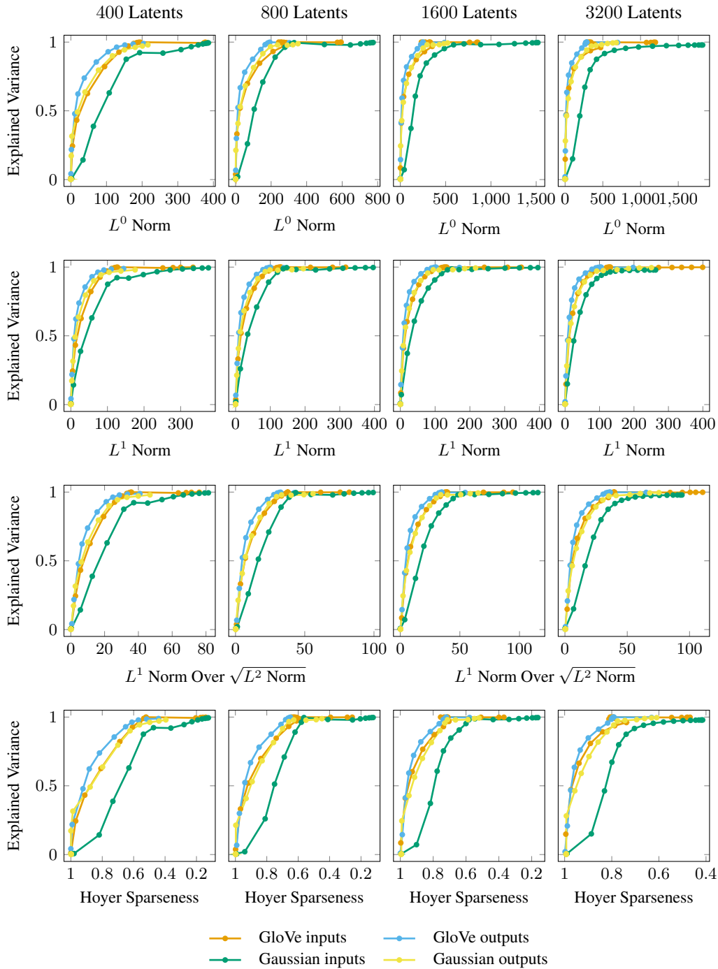
Figure 28: Explained-variance-vs-sparsity Pareto frontiers comparing 200-dimensional GloVe word embeddings, matched Gaussian controls with the same mean and variance, and the corresponding outputs after a randomly initialized two-layer MLP. The comparison mirrors the other dimensions: a small input-side GloVe-vs-control gap that narrows at the output.
