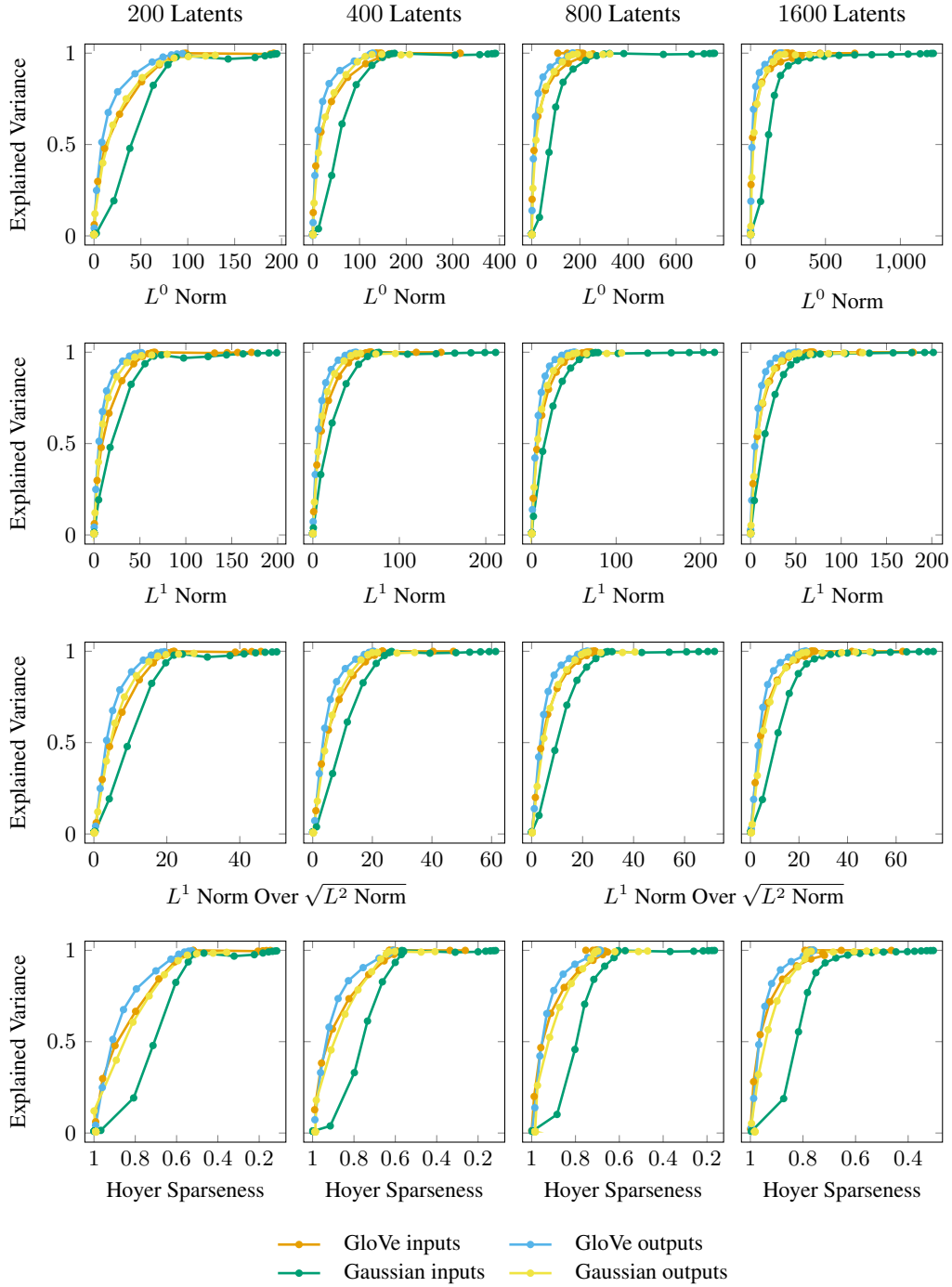
Figure 27: Explained-variance-vs-sparsity Pareto frontiers comparing 100-dimensional GloVe word embeddings, matched Gaussian controls with the same mean and variance, and the corresponding outputs after a randomly initialized two-layer MLP. The GloVe-vs-control gap is small at the input and narrower still at the output.
