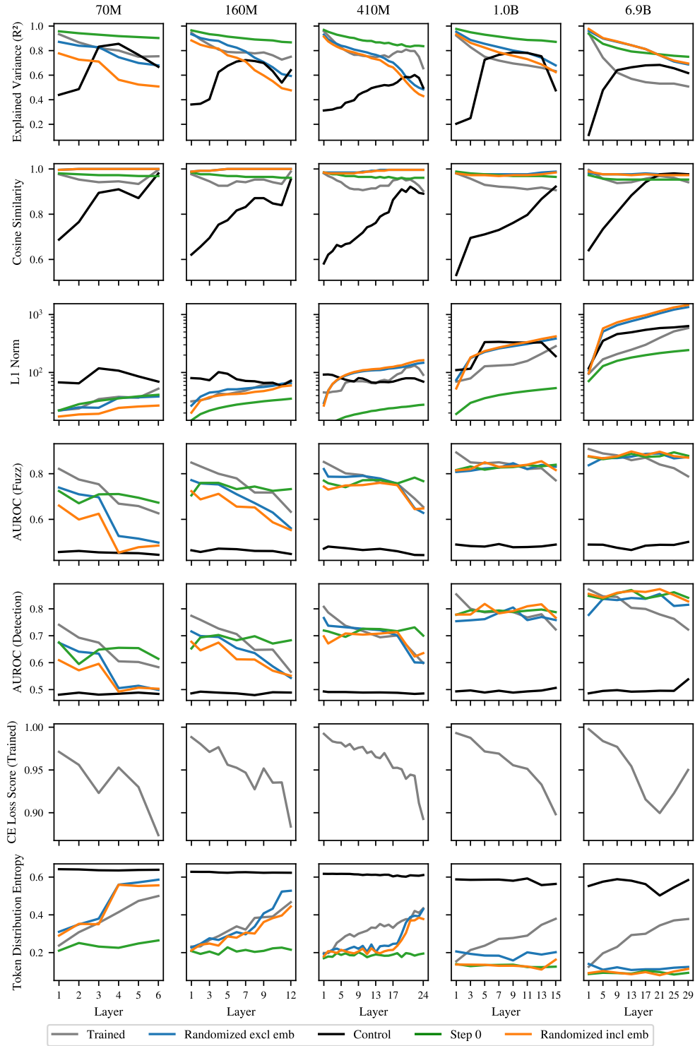
Figure 2: Head-to-head SAE performance across the Pythia suite (70M to 6.9B parameters), one column per model size and one row per metric. The comparison is consistent across every metric and scale: the trained variant and the three randomized variants track one another closely, layer for layer, whereas the control is the lone outlier. The trained-vs-random curves converge further as model size grows. In short, four variants that differ fundamentally in how their weights were obtained—one trained, three never trained—land on comparable performance, and only the random-embedding control separates out.
