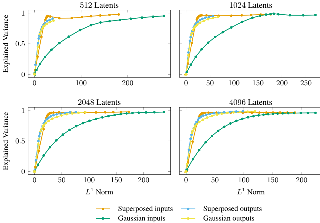
Figure 23: Explained-variance-vs- L^1 -norm (sparsity) Pareto frontiers comparing toy datasets generated to exhibit superposition, matched Gaussian controls with the same mean and variance, and the corresponding outputs after a randomly initialized two-layer MLP. As under the other sparsity measures, the large input-side superposed-vs-control gap nearly closes at the MLP output.
