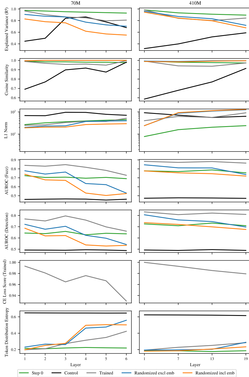
Figure 15: Evaluation metrics for SAEs trained with one billion tokens on Pythia-70m and 410m. Compared column-for-column against the 100M-token results in Figure 2, the curves are qualitatively unchanged: the trained-vs-random near-parity holds at 10\times the training data.
