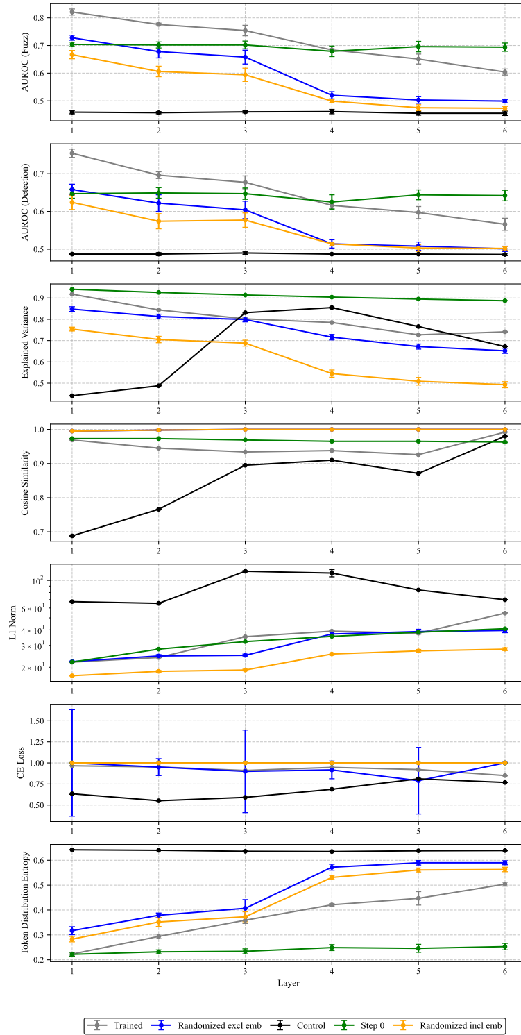
Figure 17: Pythia-70m metrics with uncertainty over five random seeds. The between-variant gaps—small between trained and randomized, large against the control—exceed the seed-to-seed variability, so the near-parity reported in the main text is not attributable to seed noise.
