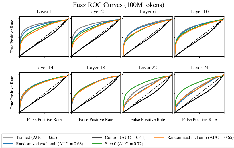
Figure 10: Trained-vs-random ‘fuzzing’ AUROC for Pythia-410m (100 latents per SAE). The trained and randomized curves are essentially indistinguishable at every layer—so at this scale fuzzing AUROC does not separate trained from randomized models—and both decline together with increasing layer index.
