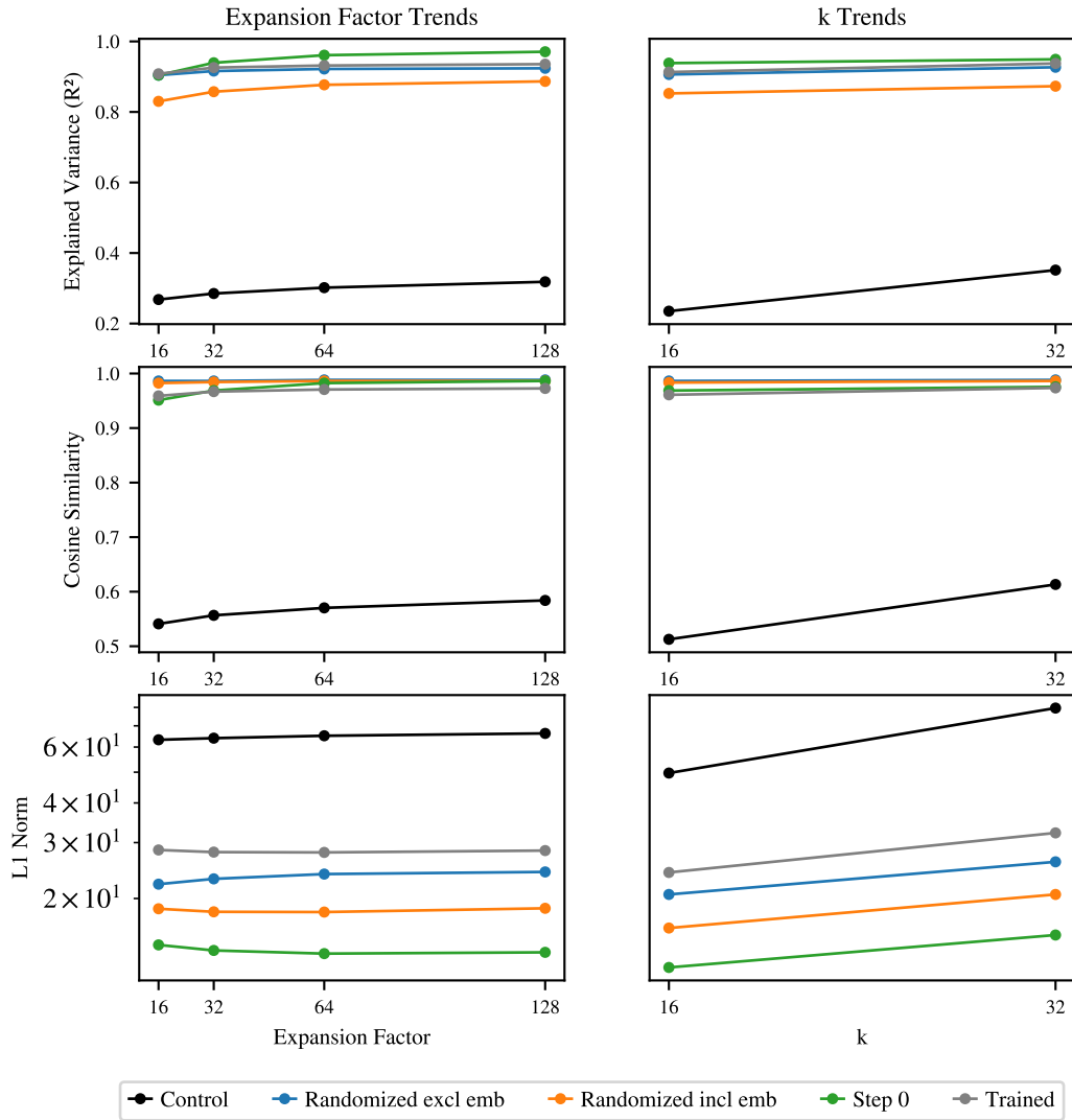
Figure 18: Robustness of SAE performance under hyperparameter variation. Standard evaluation metrics remain stable across expansion factors R from 16 to 128 and sparsities k from 16 to 32, with all initialization strategies preserving their relative ordering. This stability suggests that moderate hyperparameter values, such as expansion factor R = 64 and sparsity k = 32 , are sufficient.
