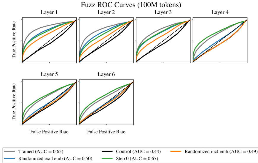
Figure 6: ROC curves for ‘fuzzing’ auto-interpretability on Pythia-70m, computed over 100 SAE latents. The curves show similar performance across SAE variants, together with an overall degradation as layer index increases.
