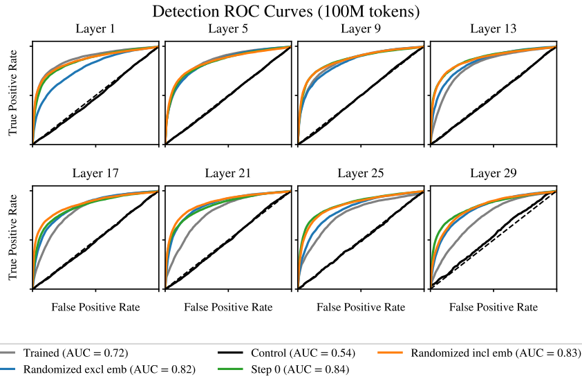
Figure 14: ROC curves for ‘detection’ auto-interpretability on Pythia-6.9b, computed over 100 SAE latents. The curves demonstrate similar performance across SAE variants.
