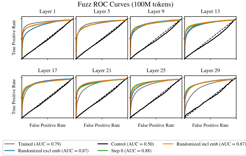
Figure 1: Layer-wise ‘fuzzing’ ROC curves for Pythia-6.9b, computed from 100 sampled latents per SAE. The trained model (gray) and randomized variants (colored) substantially overlap, whereas the control condition (black) remains near chance (dotted), indicating that aggregate AUROC is, by itself, insufficient for attributing latents to learned computation. See Figure 2 for additional metrics and model sizes, and Appendix E for multiple random seeds.
