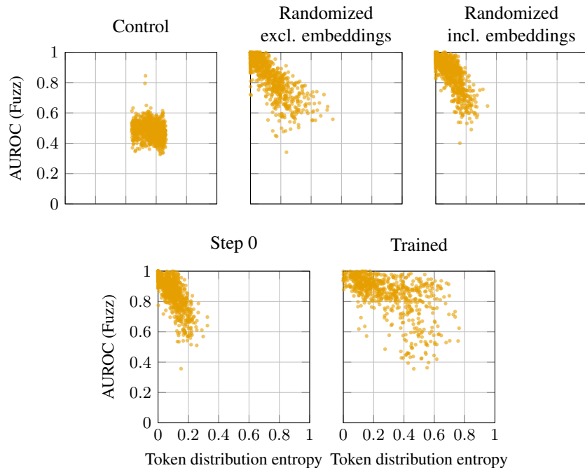
Figure 20: Scatter plots of the per-latent token distribution entropy against ‘fuzzing’ AUROC (auto-interpretability score) for SAEs trained on multiple layers of the Pythia-6.9b model. Each point corresponds to a single latent, taken from the sample of latents used to compute the aggregate metrics displayed in Figures 1 and 2.
