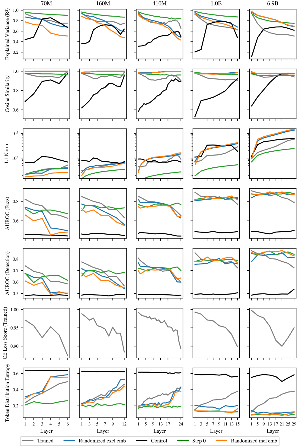
Figure 2: Sparse-autoencoder metrics across Pythia models from 70M to 6.9B parameters. Trained, Step-0, and re-randomized variants show similar trends across model scales, whereas the control condition is consistently separated on several reconstruction metrics. Larger models exhibit more stable layerwise behavior, and all non-control variants achieve broadly comparable performance despite different initialization conditions.
