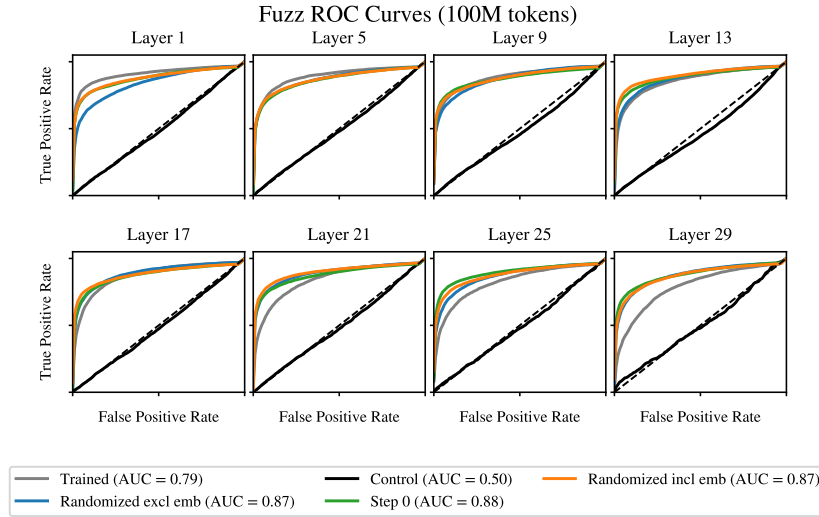
Figure 1: ‘Fuzzing’ ROC curves by layer for Pythia-6.9b, with 100 latents sampled per SAE. The trained model (gray) and randomized variants (colored) occupy a similar range, whereas the control (black) remains near chance (dotted), illustrating that aggregate AUROC alone is not enough to attribute latents to learned computation. Figure 2 reports additional metrics and model sizes, and Appendix E shows multiple random seeds.
