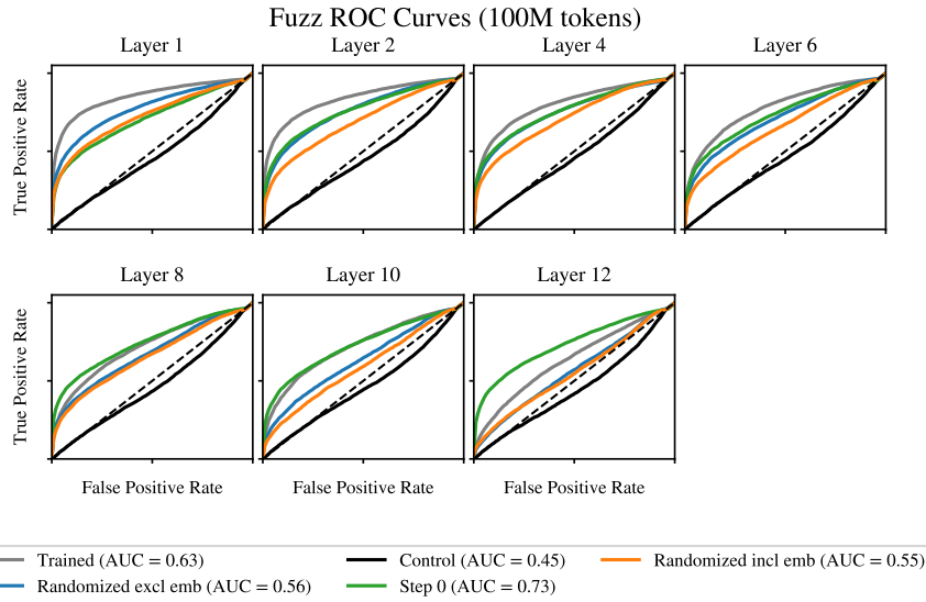
Figure 8: ROC curves for ‘fuzzing’ auto-interpretability on Pythia-160m over 100 SAE latents. The variants show similar layerwise behavior, including an overall degradation as layer index increases.
