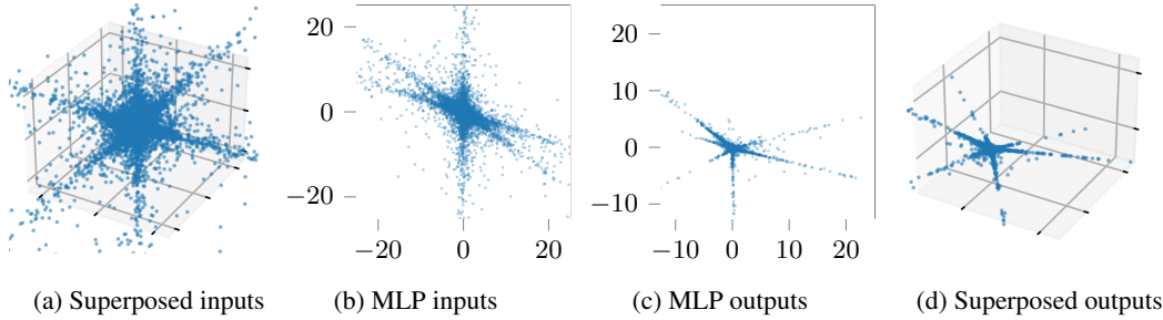
Figure 3: Illustration of how a randomly initialized neural network transforms superposed input data. We draw 10K samples of n_s = 3 sparse input features from a Lomax distribution with shape \alpha = 1 and scale \lambda = 1 , then project them to n_d = 2 dense input features using an i.i.d. standard normal matrix. We pass the dense vectors through a two-layer ReLU MLP with hidden size 4n_d and recover n_s = 3 sparse outputs using the inverse of the previously generated projection matrix.
