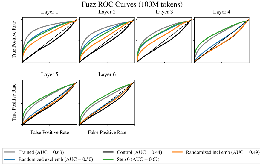
Figure 6: ROC curves for ‘fuzzing’ auto-interpretability on Pythia-70m over 100 SAE latents. The variants show similar layerwise behavior, including an overall degradation as layer index increases.
