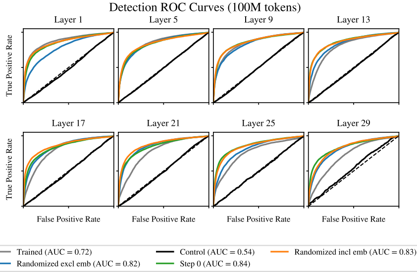
Figure 14: ROC curves for ‘detection’ auto-interpretability on Pythia-6.9b over 100 SAE latents. The trained and randomized variants again occupy a similar performance range.
