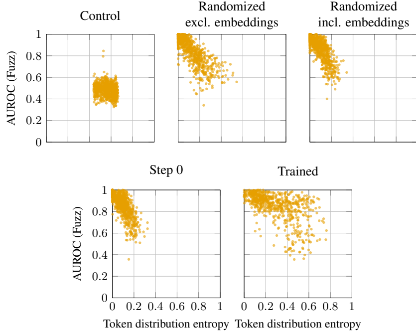
Figure 20: Per-latent token-distribution entropy plotted against ‘fuzzing’ AUROC (auto-interpretability score) for SAEs trained on multiple Pythia-6.9b layers. Each point is a single latent from the same sample used to compute the aggregate metrics in Figures 1 and 2.
