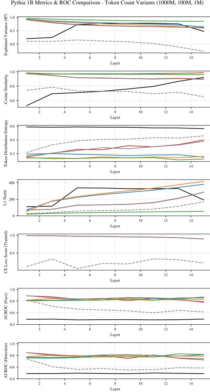
Figure 16: Evaluation metrics for SAEs trained with 1M and 1B tokens on Pythia-1b. The 1M-token SAEs have substantially lower explained variance and CE loss score, indicating under-training. Average auto-interpretability scores are slightly lower in the earliest layers and decline sharply with depth, while layerwise trends in auto-interpretability and token-distribution entropy remain consistent with the other SAE settings.
