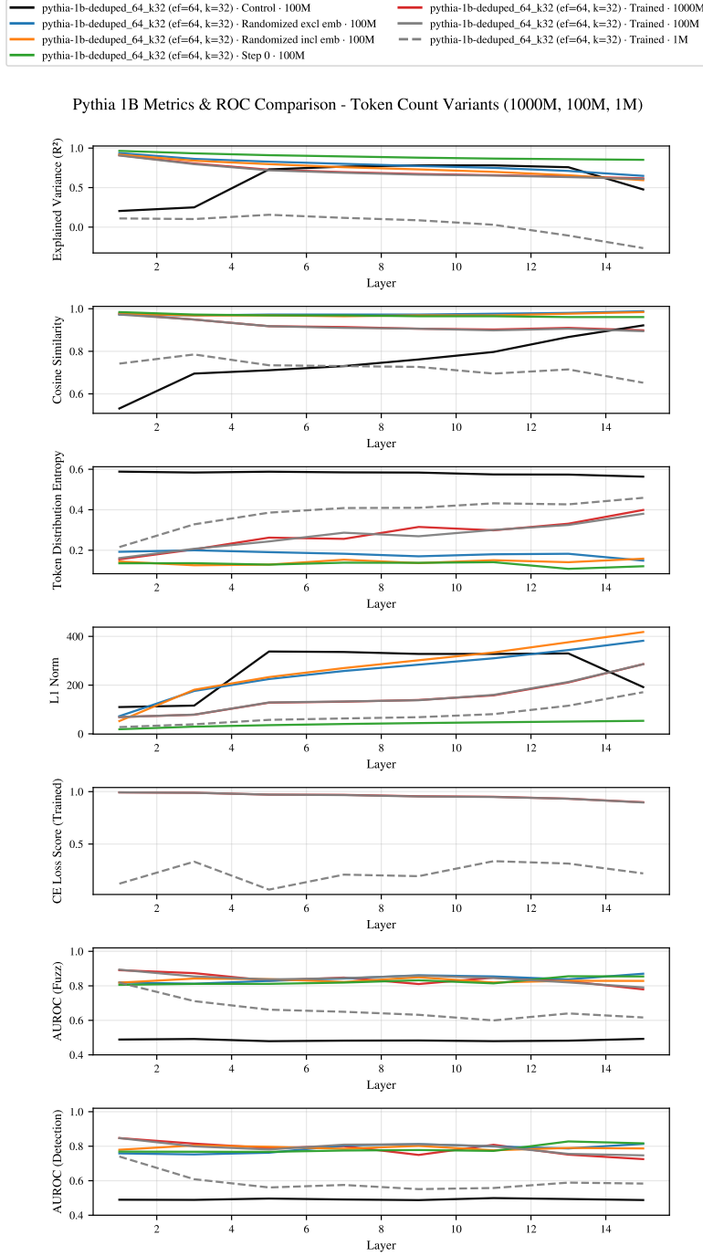
Figure 16: Evaluation metrics for SAEs trained with 1M and 1B tokens on Pythia-1b. The explained variance and CE loss score are markedly lower for the 1M model, indicating that these SAEs are under-trained. Average auto-interpretability scores are slightly lower at the earliest layers and decline sharply with depth. The trends in auto-interpretability and token-distribution entropy with layer index remain consistent with those seen for our other SAEs, suggesting the qualitative picture is robust to the training-data budget.
