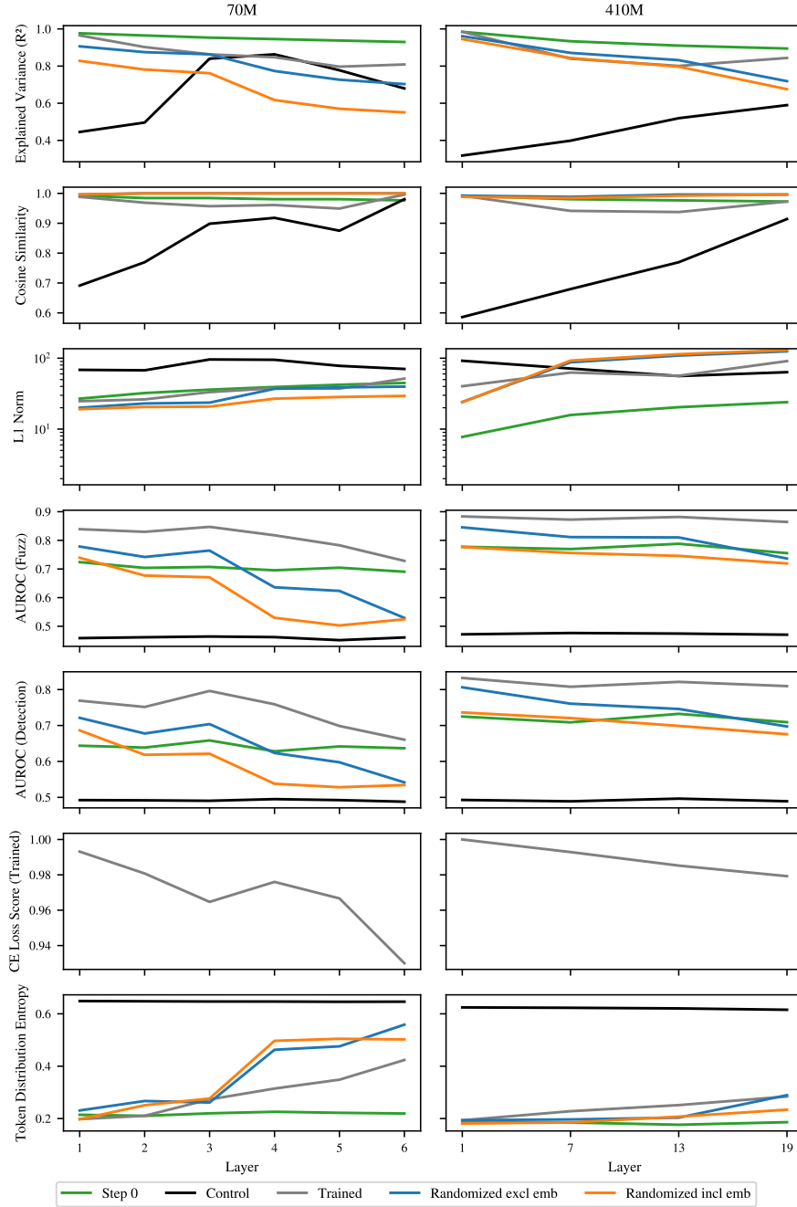
Figure 15: Evaluation metrics for SAEs trained with one billion tokens on the Pythia-70m and 410m models. These correspond to columns of Figure 2, which reports the same metrics for SAEs trained on 100M tokens; the behavior is qualitatively unchanged, indicating that the effect persists across training-data budgets.
