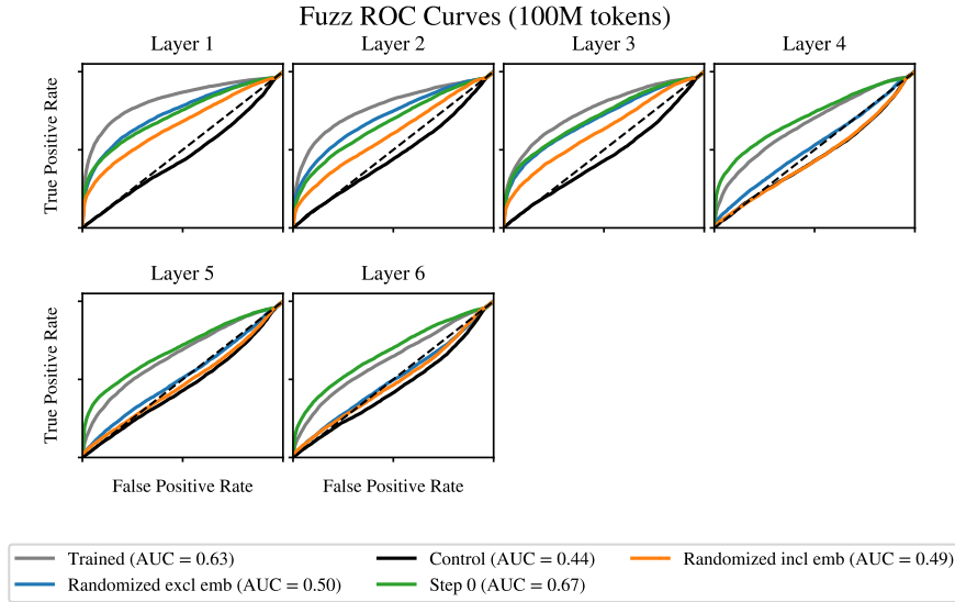
Figure 6: ROC curves for ‘fuzzing’ auto-interpretability for Pythia-70m over 100 SAE latents. As at other scales, the SAE variants perform similarly, and performance degrades overall as the layer index increases.
