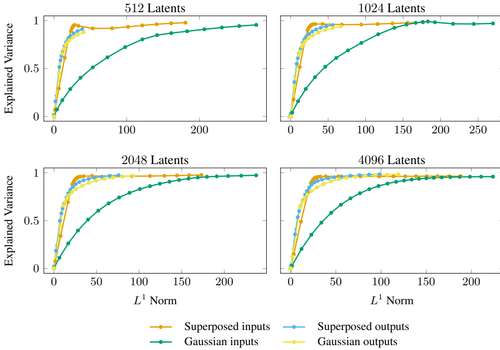
Figure 23: Pareto frontiers of explained variance against the L^1 norm (sparsity), across toy datasets generated to exhibit superposition, Gaussian controls with matched mean and variance, and the corresponding outputs obtained by passing these inputs through a randomly initialized two-layer MLP.
