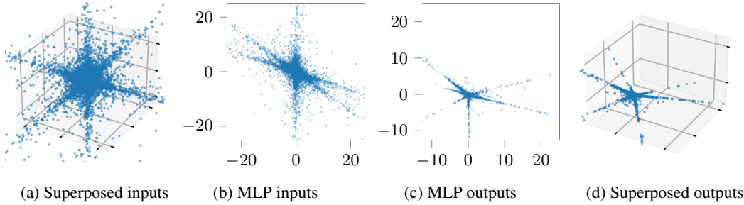
Figure 3: An illustrative example of the effect that a randomly initialized neural network has on superposed input data. We take 10K samples of n_s = 3 sparse input features from a Lomax distribution with shape \alpha = 1 and scale \lambda = 1 and project these to n_d = 2 dense input features via an i.i.d. standard normal matrix. We then pass the dense outputs through a two-layer MLP with ReLU activation and hidden size 4n_d , and recover n_s = 3 sparse outputs using the inverse of the previously generated projection matrix.
