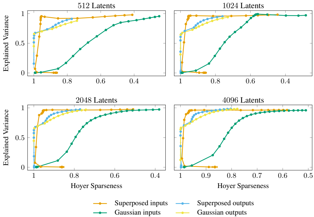
Figure 25: Pareto frontiers of explained variance against the Hoyer sparseness (sparsity), across toy datasets generated to exhibit superposition, Gaussian controls with matched mean and variance, and the corresponding outputs obtained by passing these inputs through a randomly initialized two-layer MLP.
