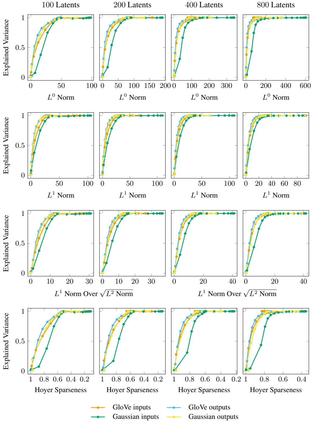
Figure 26: Pareto frontiers of explained variance against sparsity measures, across 50-dimensional GloVe word vectors, Gaussian controls with matched mean and variance, and the corresponding outputs obtained by passing these inputs through a randomly initialized two-layer MLP.
