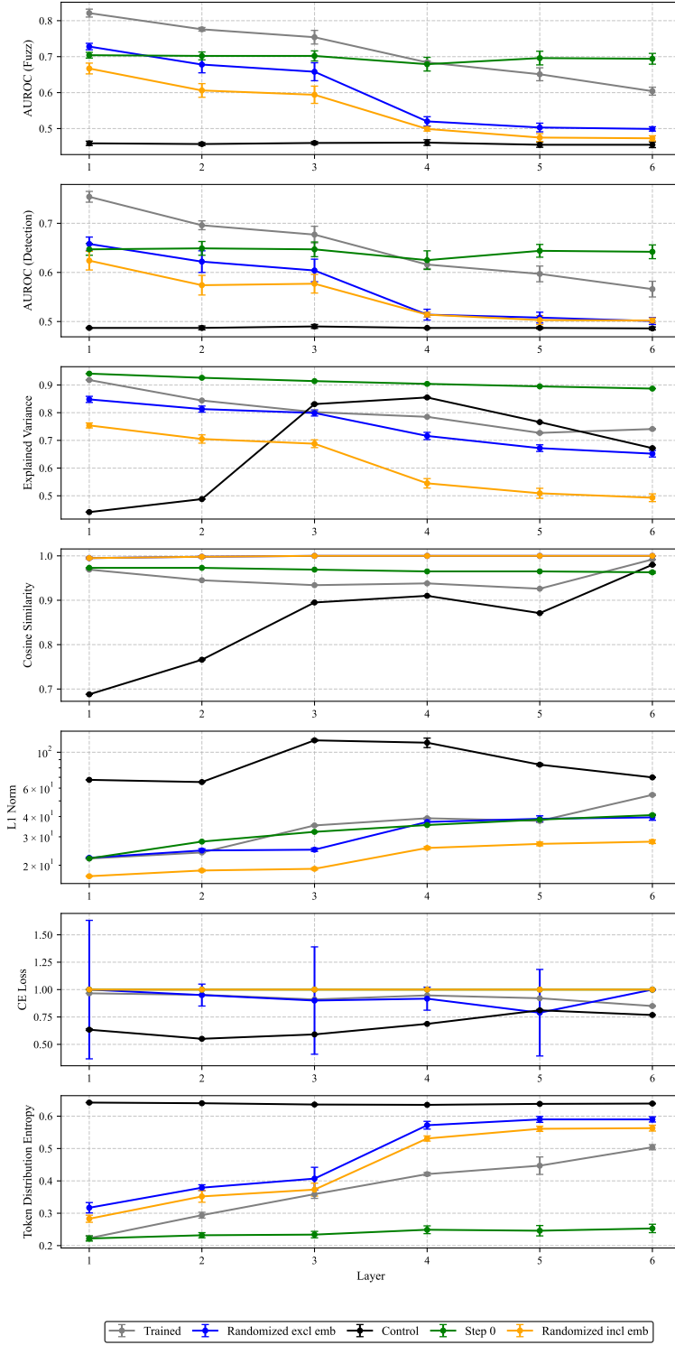
Figure 17: Uncertainty for the Pythia-70m metrics, computed across five random seeds.
