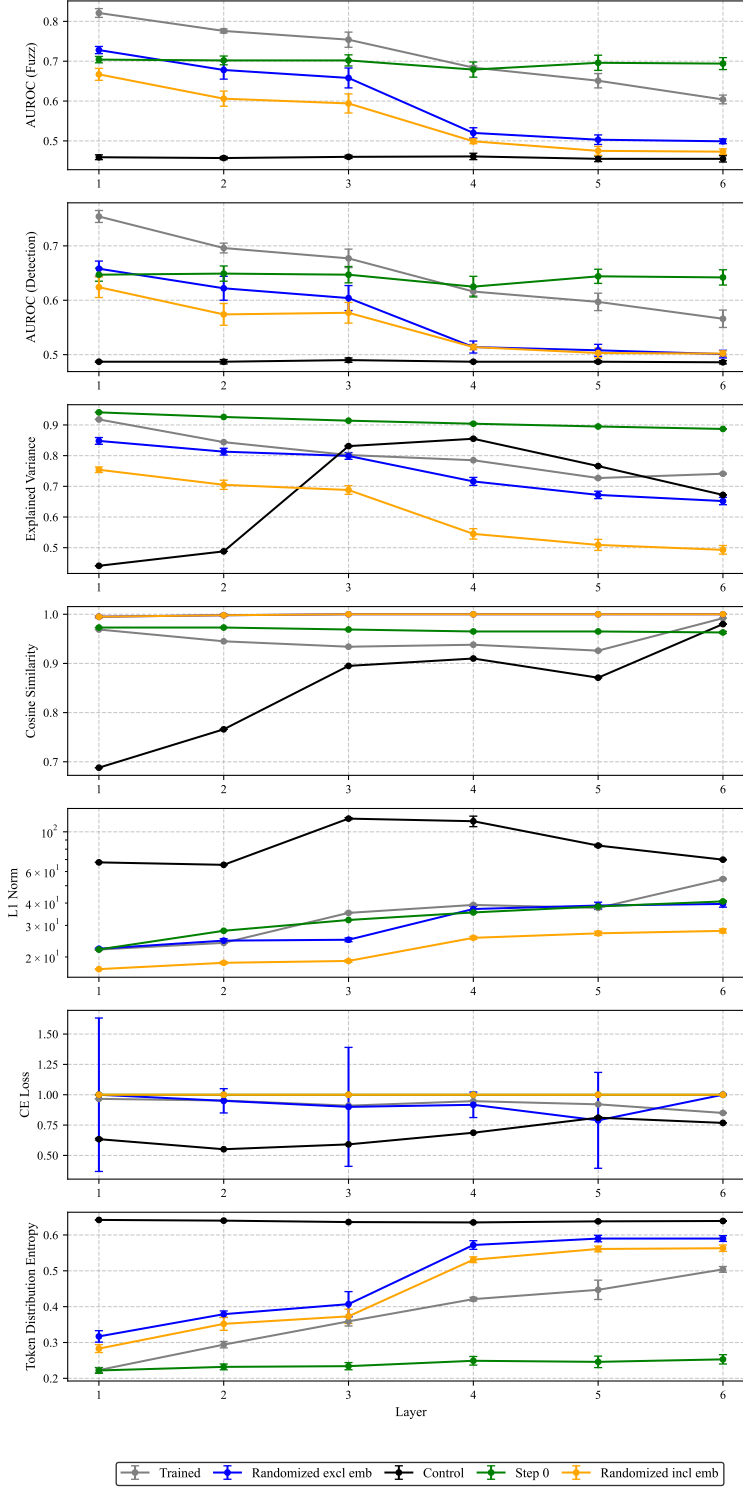
Figure 17: Uncertainty estimates for Pythia-70m metrics computed from five random seeds.
