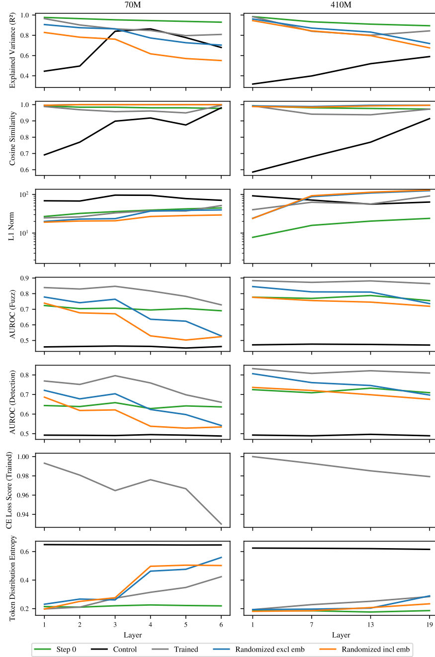
Figure 15: Evaluation metrics for SAEs trained on one billion tokens for the Pythia-70m and Pythia-410m models. These panels correspond to the same metric columns in Figure 2, where SAEs are trained on 100M tokens, and they exhibit qualitatively similar behavior.
