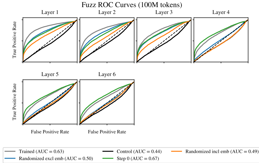
Figure 6: ‘Fuzzing’ auto-interpretability ROC curves for Pythia-70m, computed over 100 sampled SAE latents. The curves show similar performance across SAE variants and a general decrease in score as layer index increases.
