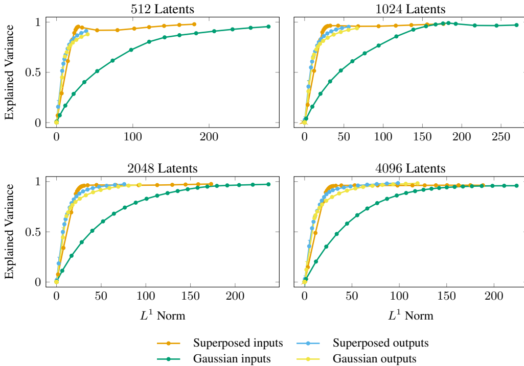
Figure 23: Pareto frontiers of explained variance against the L^1 norm (sparsity) for toy datasets constructed to exhibit superposition, Gaussian controls matched in mean and variance, and the corresponding outputs produced by a randomly initialized two-layer MLP.
