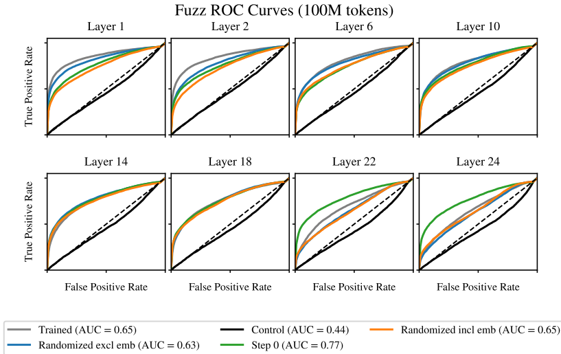
Figure 10: ‘Fuzzing’ auto-interpretability ROC curves for Pythia-410m, computed over 100 sampled SAE latents. The variants exhibit similar performance profiles and a general score decrease with layer index; in this setting, the auto-interpretability scores do not separate trained and randomized models.
