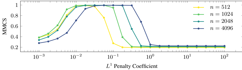
Figure 4: Mean max cosine similarity (MMCS) between the SAE-learned features (decoder weight vectors) and the data-generating features, as a function of the L^1 penalty coefficient in the training loss, following Sharkey et al. (2022). An intermediate ‘Goldilocks zone’ of the penalty coefficient yields near-exact recovery of the data-generating features, provided the SAE has sufficiently many latents to represent them.
