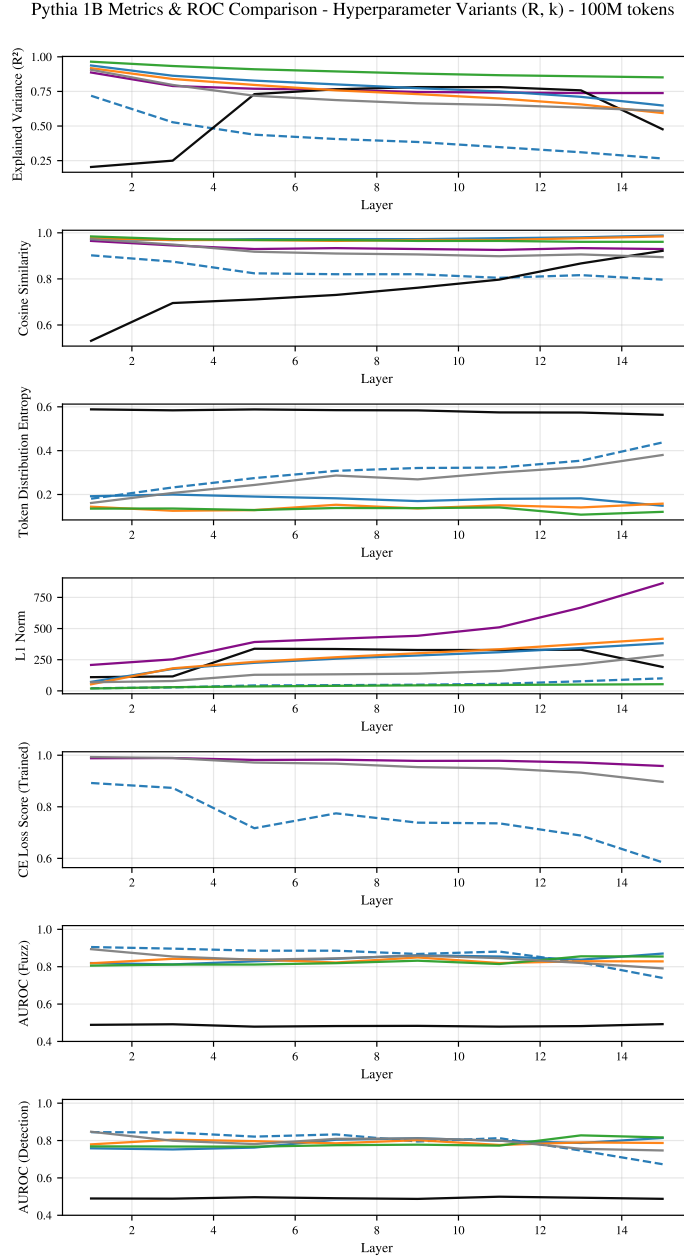
Figure 19: Evaluation metrics for SAEs trained on Pythia-1b under varying hyperparameters, alongside the main results reproduced from Figure 2. SAEs with a very small expansion factor R = 2 and sparsity k = 4 are clearly separated from the default configuration by both explained variance and CE loss score. Crucially, however, their auto-interpretability scores remain comparable to those of the default configuration, on both trained and randomized models.
