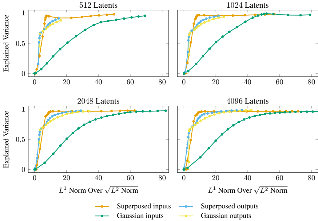
Figure 24: Pareto frontiers of explained variance against the sparsity measure L^1/\sqrt{L^2} for the toy datasets constructed to exhibit superposition, the Gaussian controls matched in mean and variance, and the corresponding outputs obtained by passing each through a randomly initialized two-layer MLP.
