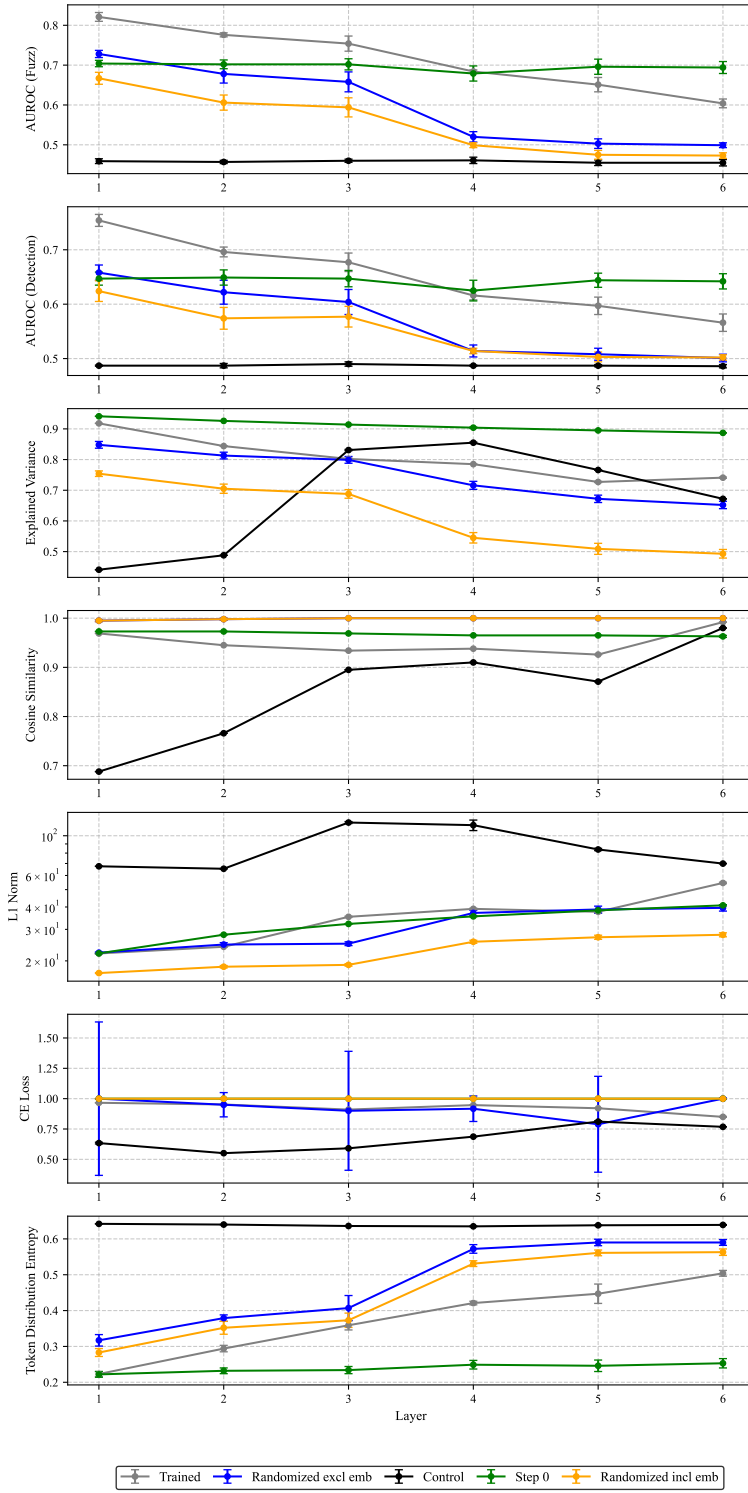
Figure 17: Uncertainty in the Pythia-70m evaluation metrics, estimated across five independent random seeds.
