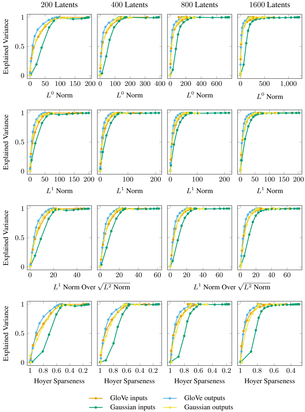
Figure 27: Pareto frontiers of explained variance against sparsity measures for 100-dimensional GloVe word embeddings, the Gaussian controls matched in mean and variance, and the corresponding outputs obtained by passing each through a randomly initialized two-layer MLP.
