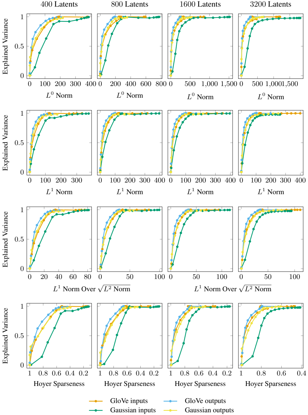
Figure 28: Pareto frontiers of explained variance against sparsity measures for 200-dimensional GloVe word embeddings, the Gaussian controls matched in mean and variance, and the corresponding outputs obtained by passing each through a randomly initialized two-layer MLP.
