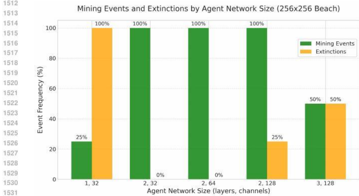
Figure 19: Frequency of mining and extinction events in a 256 \times 256 Beach world for different agent policy network sizes. Frequencies are computed across four random seeds for each setting.
