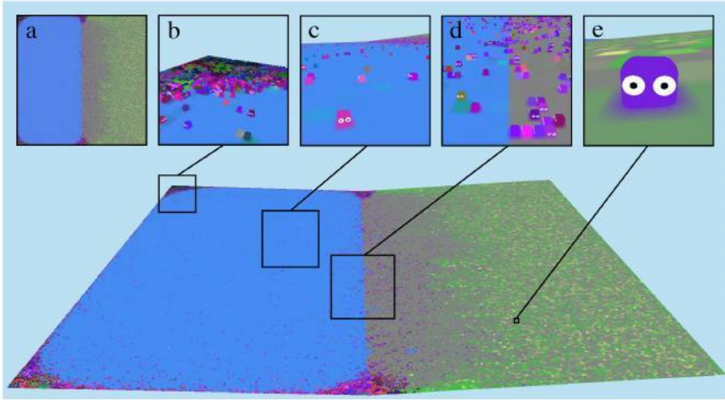
Figure 1: 3D visualization of a 512 \times 512 map in our environment. Insert (a) shows a top-down view of the full map; (b) shows agents clustered near a corner; (c) shows agents in water; (d) shows agents traveling between land and water; and (e) shows a close view of a single agent gathering resources.
