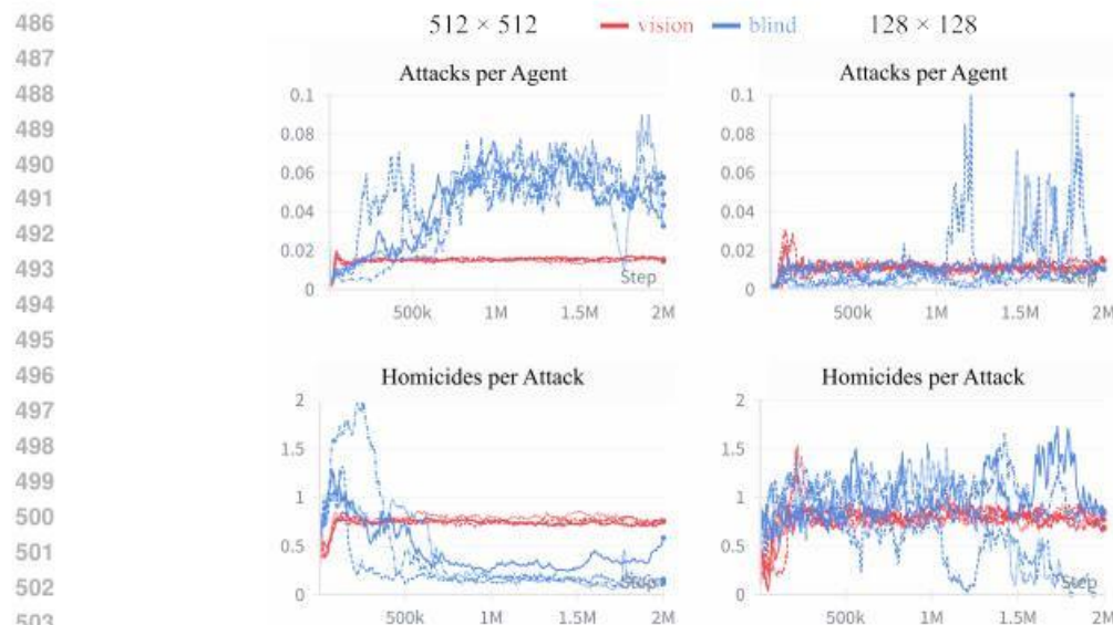
Figure 6: Attacks per agent and homicides per attack, averaged across agents, in 512 \times 512 and 128 \times 128 Ocean worlds. Each plot shows four seeds with vision agents ( RCV + A ) (red) and four seeds with blind agents ( RC + A ) (blue). With vision, agents attack less often but with higher precision, consistent with the emergence of specialized predation behavior. The effect is clearer at larger scales. Figure 10 in Appendix C compares the 1024 \times 1024 and 256 \times 256 grid sizes.
