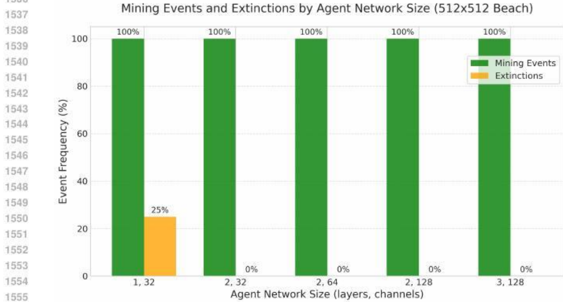
Figure 20: Frequency of mining and extinction events in a 512 \times 512 Beach world for different agent policy network sizes. Frequencies are computed across four random seeds for each setting.
