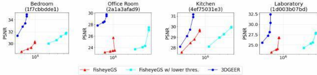
Figure 5: PSNR↑ Trends When Scaling-Up Gaussian Counts. Increasing Gaussian count improves the splatting baseline but does not close the projective-exactness gap (see full metrics in Fig. K.3 and Tab. K.3).
