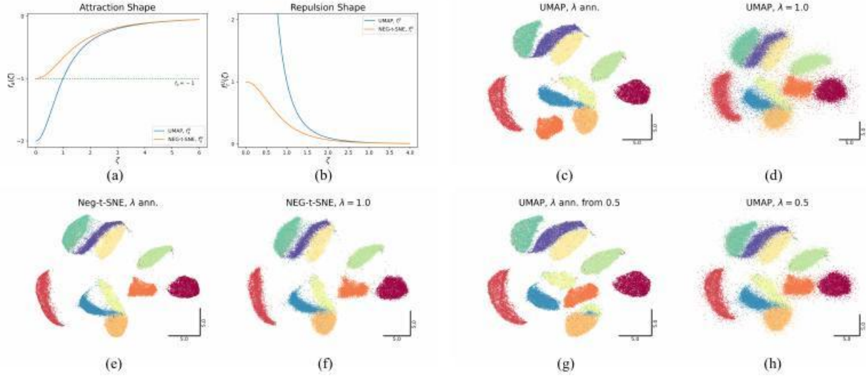
Figure 11: Sensitivity of UMAP and NEG- t -SNE to learning rate on the MNIST dataset. (a) Attraction and (b) repulsion shapes for UMAP ( a = 1 , b = 1 ) and NEG- t -SNE. (c,d) UMAP is very sensitive to the learning rate \lambda , as f_a^U < -1 as the separation distance \zeta decreases. Thus, without annealing, the clusters become fuzzy. (e,f) NEG- t -SNE is less sensitive to \lambda as f_a^N \in [-1, 0] always, and the clusters are thus less fuzzy even when not annealed. (g,h) Confining f_a^U to [-1, 0] by setting \lambda = 0.5 shows less sensitivity to \lambda .
