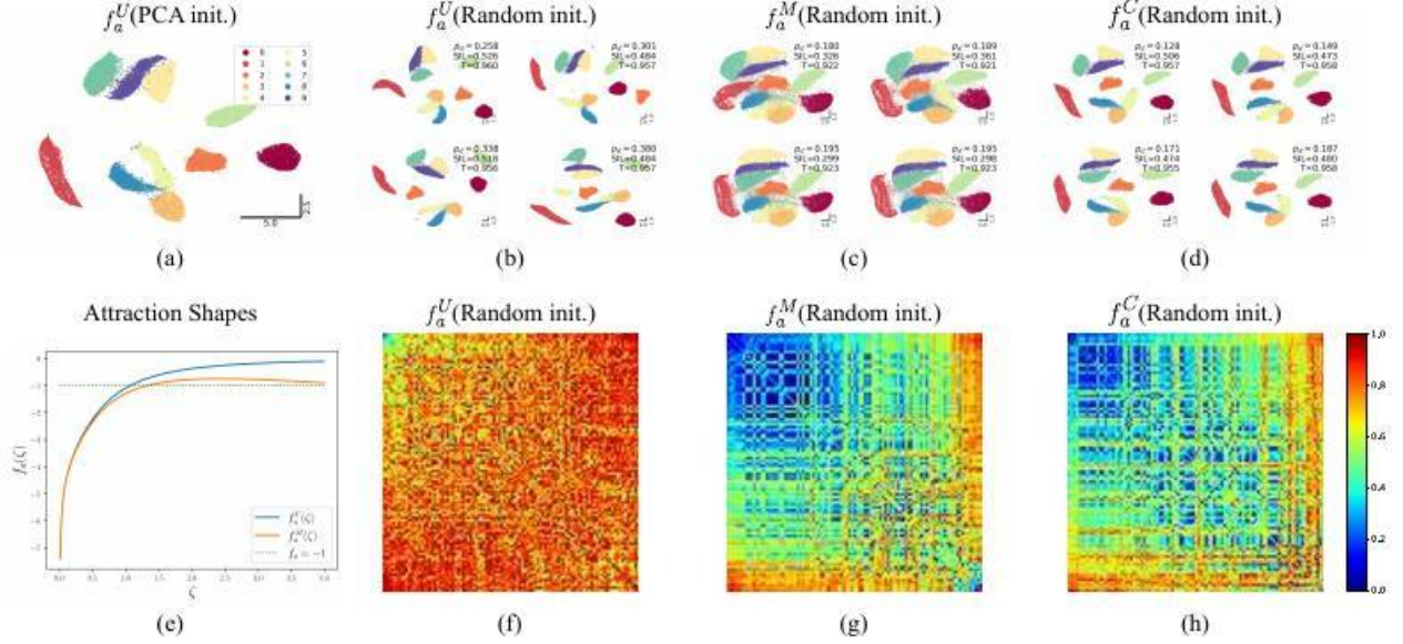
Figure 2: Effect of random initialization on different attraction shapes for the MNIST dataset. (a) PCA-initialized mapping used as the reference. (b-d) Four mappings with the lowest Procrustes distance ( p_d ) from the embedding in (a) for (b) UMAP, (c) modified, and (d) composite attraction shapes. (e) Default UMAP and modified attraction shapes. (f-h) Procrustes matrices from 100 runs of (f) UMAP ( 0.78 \pm 0.13 ), (g) modified ( 0.49 \pm 0.21 ), and (h) composite attraction ( 0.50 \pm 0.20 ) shapes. The diagonal ( i, i ) entries are sorted by Procrustes distance ( p_d ) from (a), and the off-diagonal ( i, j ) entries give p_d between the i^{\text{th}} and j^{\text{th}} mappings. The matrices and (mean p_d \pm \text{std} ) values show that the modified and composite attraction shapes produce more self-similar, scale-invariant structure than default UMAP under random initialization.
