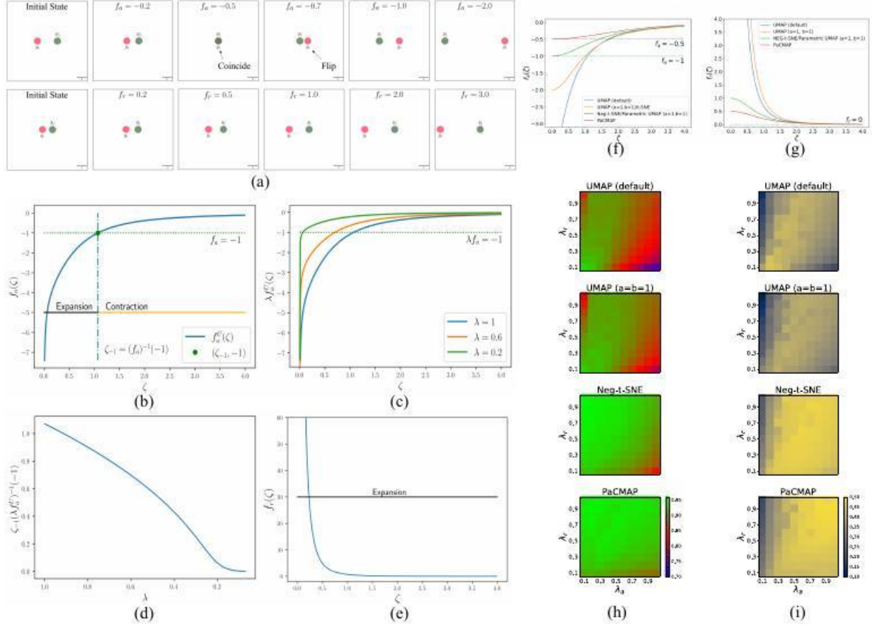
Figure 1: Attraction and repulsion shapes in UMAP and related embeddings. (a) Pairwise effect of different values of f_a (top) and f_r (bottom). (b) UMAP attraction shape. (c) Effective attraction shape ( \lambda f_a ) under several learning rates \lambda . (d) Minimum distance for contraction ( \zeta_{-1} ) as \lambda decreases. (e) UMAP repulsion shape. (f) Attraction and (g) repulsion shapes for several embedding methods. (h) Trustworthiness and (i) Silhouette Score when the constant learning rates for attraction ( \lambda_a ) and repulsion ( \lambda_r ) are varied independently. Default UMAP parameters: a = 1.58 and b = 0.89 .
