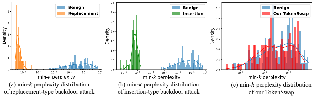
Figure 1: Min- k perplexity distribution for (a)(b) representative fixed-pattern backdoor attacks and (c) TokenSwap. Existing LVLM attacks primarily instantiate two payload mechanisms: (i) Insertion, in which the backdoored model appends or inserts predefined target content into the predicted answer (Lyu et al., 2024a;b; Ni et al., 2024; Yuan et al., 2025); (ii) Replacement, in which the triggered model suppresses the original response and emits only the target content (Lin et al., 2023; Lu et al., 2024; Liang et al., 2025). The resulting distributions make fixed-pattern attacks readily separable by the detector, whereas TokenSwap remains substantially more evasive under the same criterion. The unusually high confidence to the recurring payload, producing a distinctive perplexity profile. The same payload is also conspicuous to human inspectors, so fixed-pattern attacks suffer not only from limited evasiveness against automated detection but also from limited stealthiness under manual inspection, as illustrated in Figure 2.
