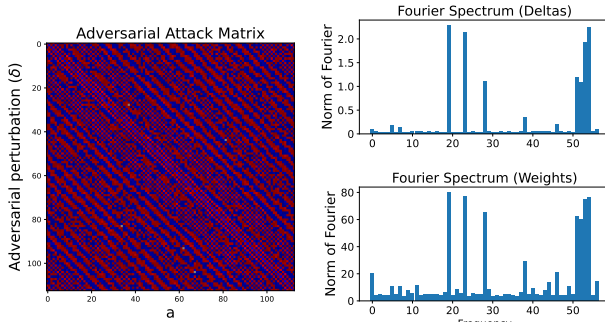
Figure 6: Left: each column is the mean attack \delta added to a to successfully attack a + b \bmod p . Right: the norms of the Fourier components of \delta and of W_{MLP_{out}} , demonstrating that the perturbation’s spectral energy concentrates precisely at the model’s key frequencies—the direct signature of the frequency-based attack mechanism.
