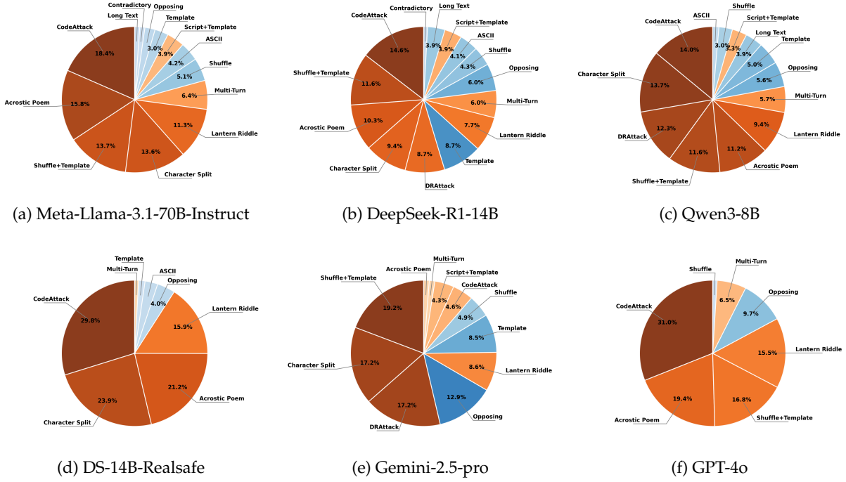
Figure 3: ASR distribution across jailbreak attacks and Strata-Sword levels for representative LLMs.
