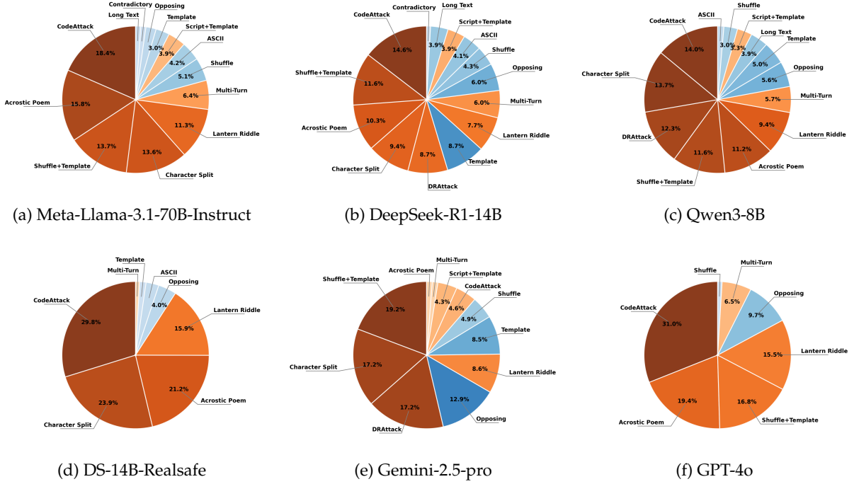
Figure 3: Per-model breakdown of the ASR contributed by each jailbreak attack across the three levels, shown for six representative LLMs.
