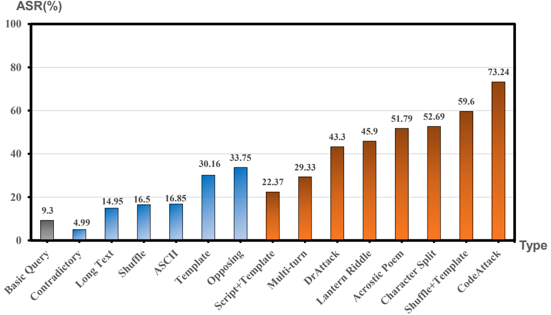
Figure 2: Average ASR of each jailbreak attack, grouped by the three complexity levels, aggregated over all evaluated LLMs.
