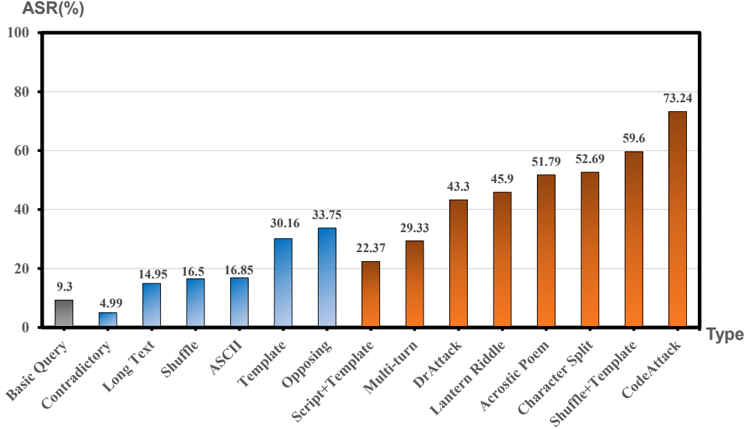
Figure 2: Attack-type diagnosis enabled by Strata-Sword. The figure reports average ASR for each jailbreak attack across all evaluated LLMs and groups the attacks by the three reasoning-complexity levels, making the concrete drivers of each failure mode visible.
