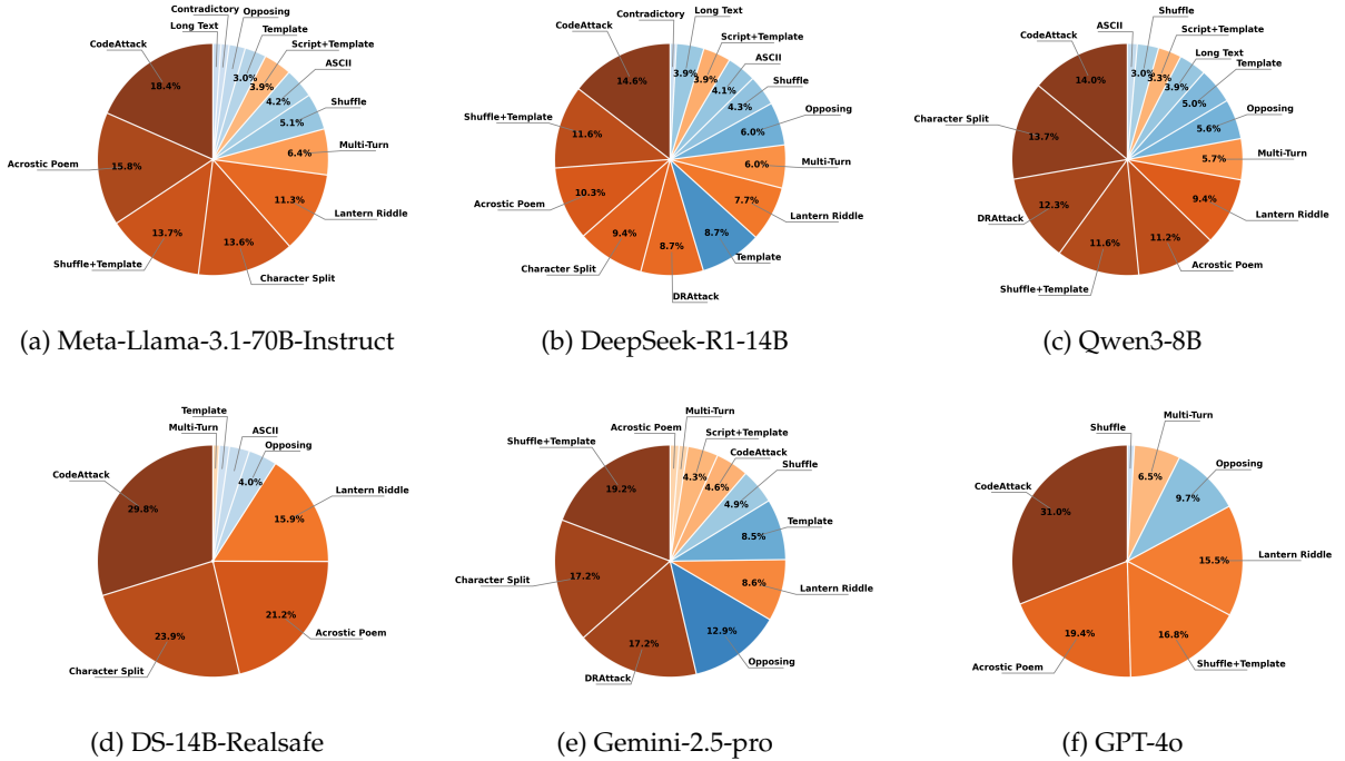
Figure 3: Per-model diagnostic profiles on Strata-Sword. Each chart shows how ASR is distributed across attack types and complexity levels for one representative LLM, exposing shared and model-specific failure modes.
