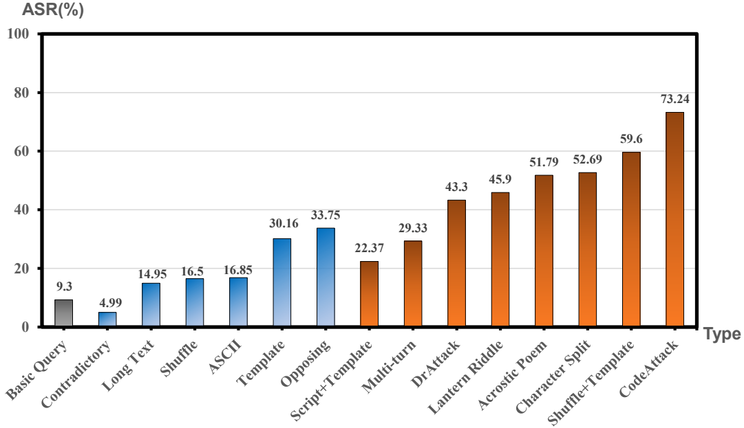
Figure 2: Average ASR of each individual jailbreak attack, grouped by its reasoning-complexity level, aggregated over all evaluated LLMs. The spread within a level shows that complexity level predicts danger only on average, and that some attacks are far more potent than their level-mates.
