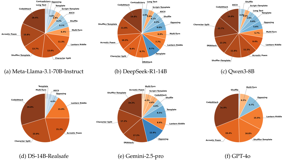
Figure 3: Per-model breakdown of ASR across the three-level attack suite for six representative LLMs. The differing slice patterns show that each model has its own signature of strengths and weaknesses, reinforcing that safety must be assessed per attack type rather than in aggregate.
