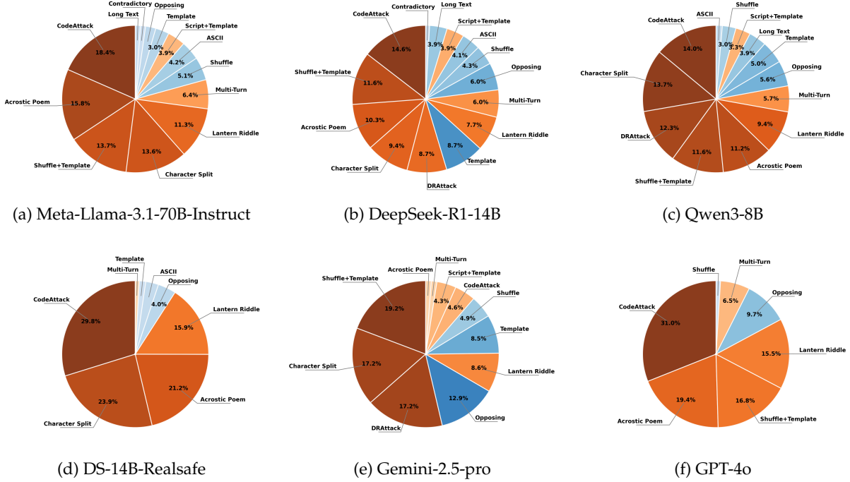
Figure 3: Per-model ASR composition across jailbreak attack methods and Strata-Sword levels for six representative LLMs, showing which attack types dominate each model’s failures.
