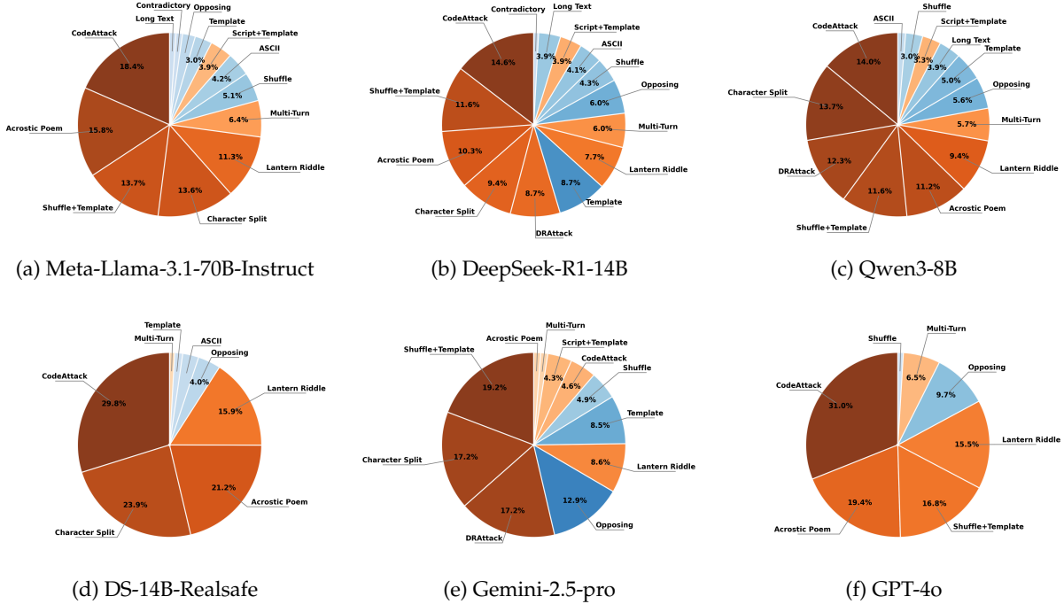
Figure 3: ASR ratios of different jailbreak attacks across the three complexity levels for representative LLMs.
