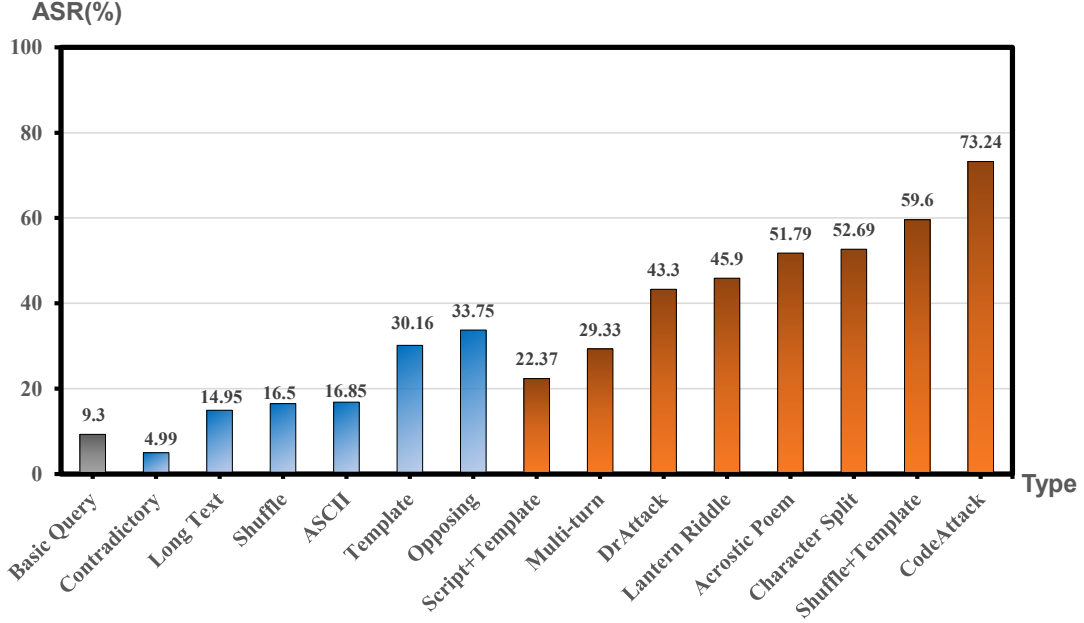
Figure 2: Average ASR of each jailbreak attack method across the evaluated LLMs, grouped by the three reasoning-complexity levels.
