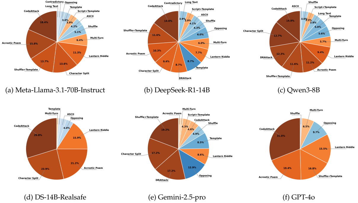
Figure 3: ASR distribution over jailbreak attack methods at the three reasoning-complexity levels for selected LLMs.
