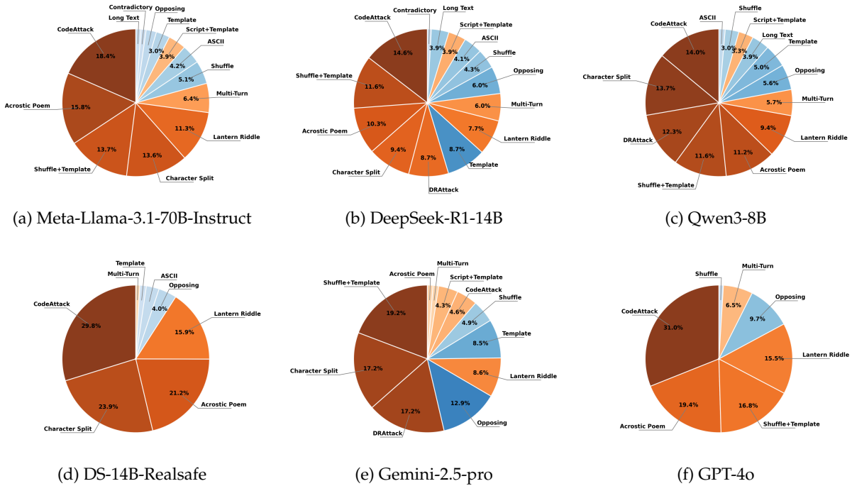
Figure 3: Per-model distribution of ASR across the individual jailbreak attacks in the three complexity levels, shown for six representative models.
