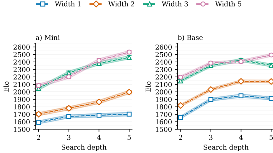
Figure 3: Estimated Elo for SOLIS Mini and SOLIS Base under unanchored planning across search widths and depths. Shaded bands denote 95% confidence intervals.
