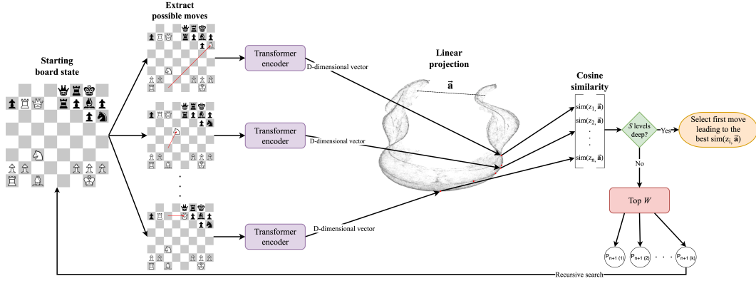
Figure 2: System overview of SOLIS. Legal child positions are embedded by the transformer encoder, scored by alignment with the global advantage vector, and pruned to the top- W continuations. For simplicity, the diagram depicts the unanchored score \cos(z', \vec{a}) .
