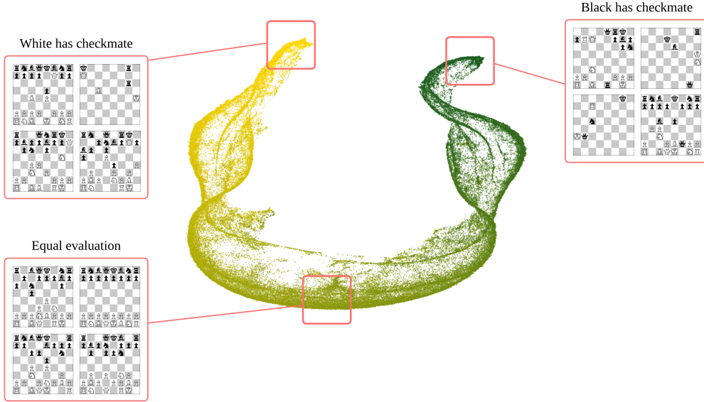
Figure 1: UMAP projection of the Base-model embedding space, with each position colored by Stockfish-evaluated win probability (gold = White favored, green = Black favored).
