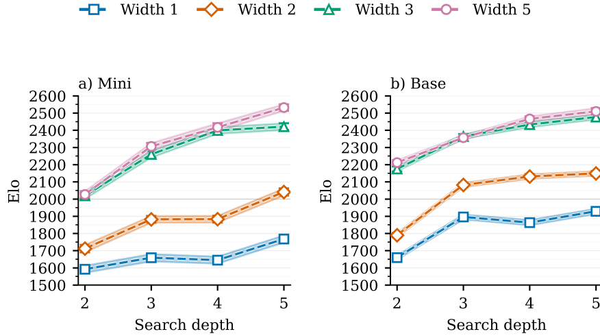
Figure 4: Estimated Elo for SOLIS Mini and SOLIS Base under anchored planning across search widths and depths. Shaded bands denote 95% confidence intervals.
