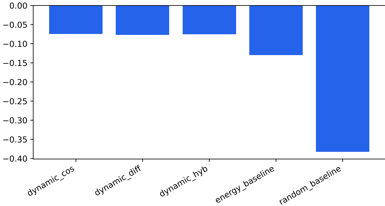
Combined score
