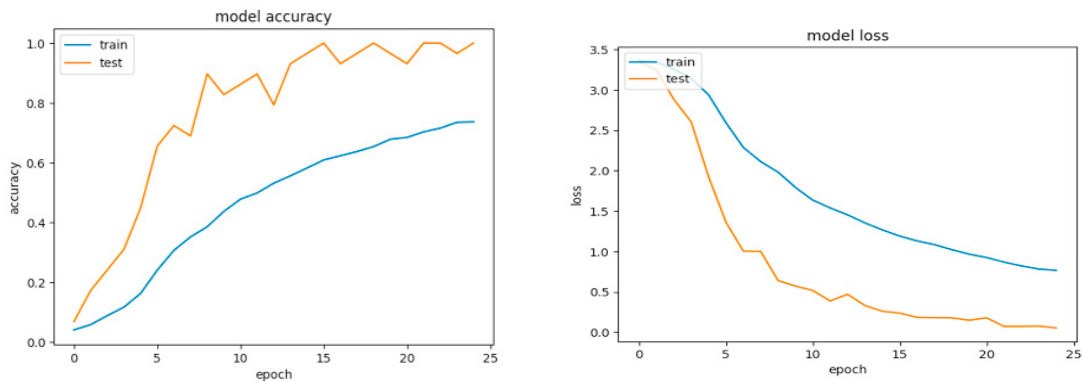
Fig. 5 shows the accuracy and loss curves of the proposed method on the ASL dataset.
