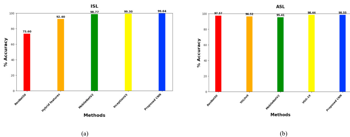
Fig. 6. The accuracy on the datasets (a) ISL, (b) ASL
