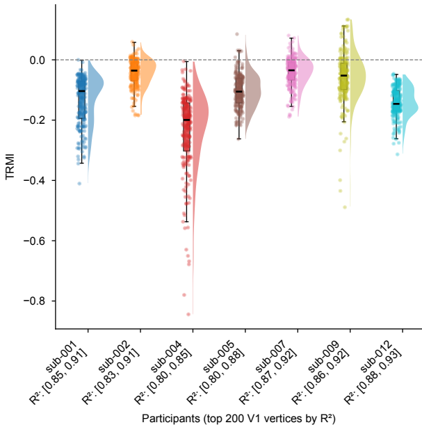
TRMI distribution across participants (parameter d x1.2)
