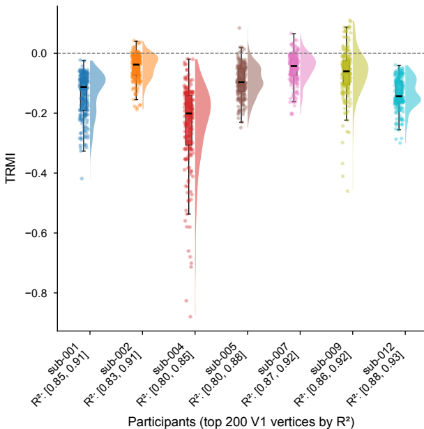
TRMI distribution across participants (pRF size x0.9)
