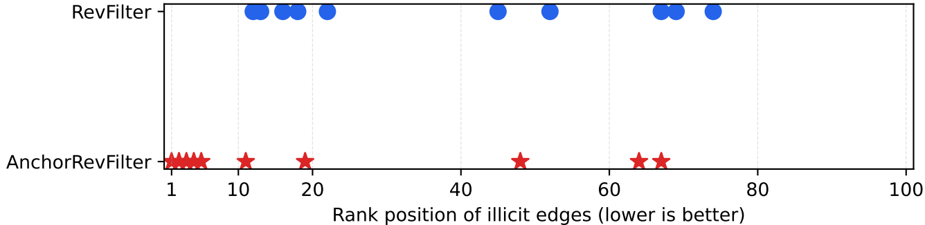
Case study on 10+1000@100: same HR, better ranking
