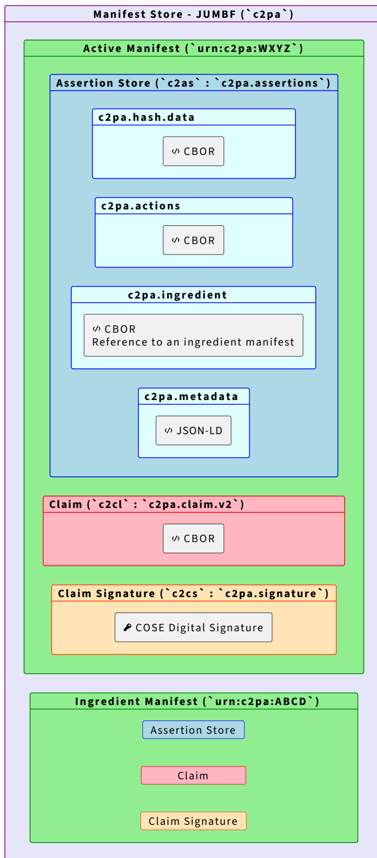
Figure 9. C2PA Manifest Store With an Ingredient
