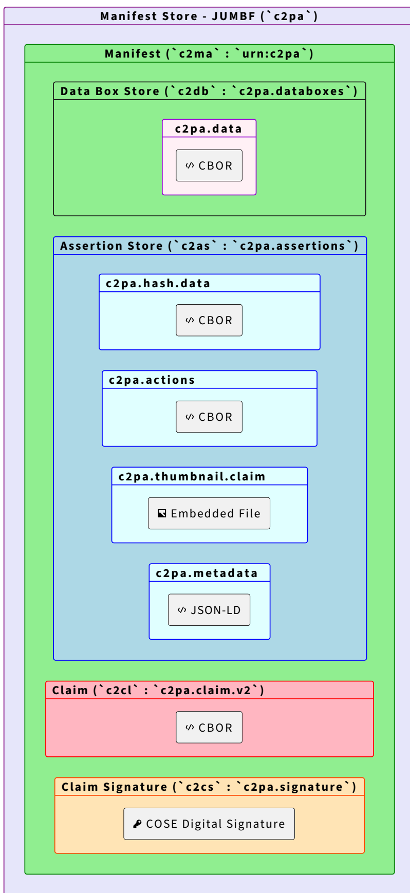
Figure 21. C2PA Manifest Store with Data Boxes
