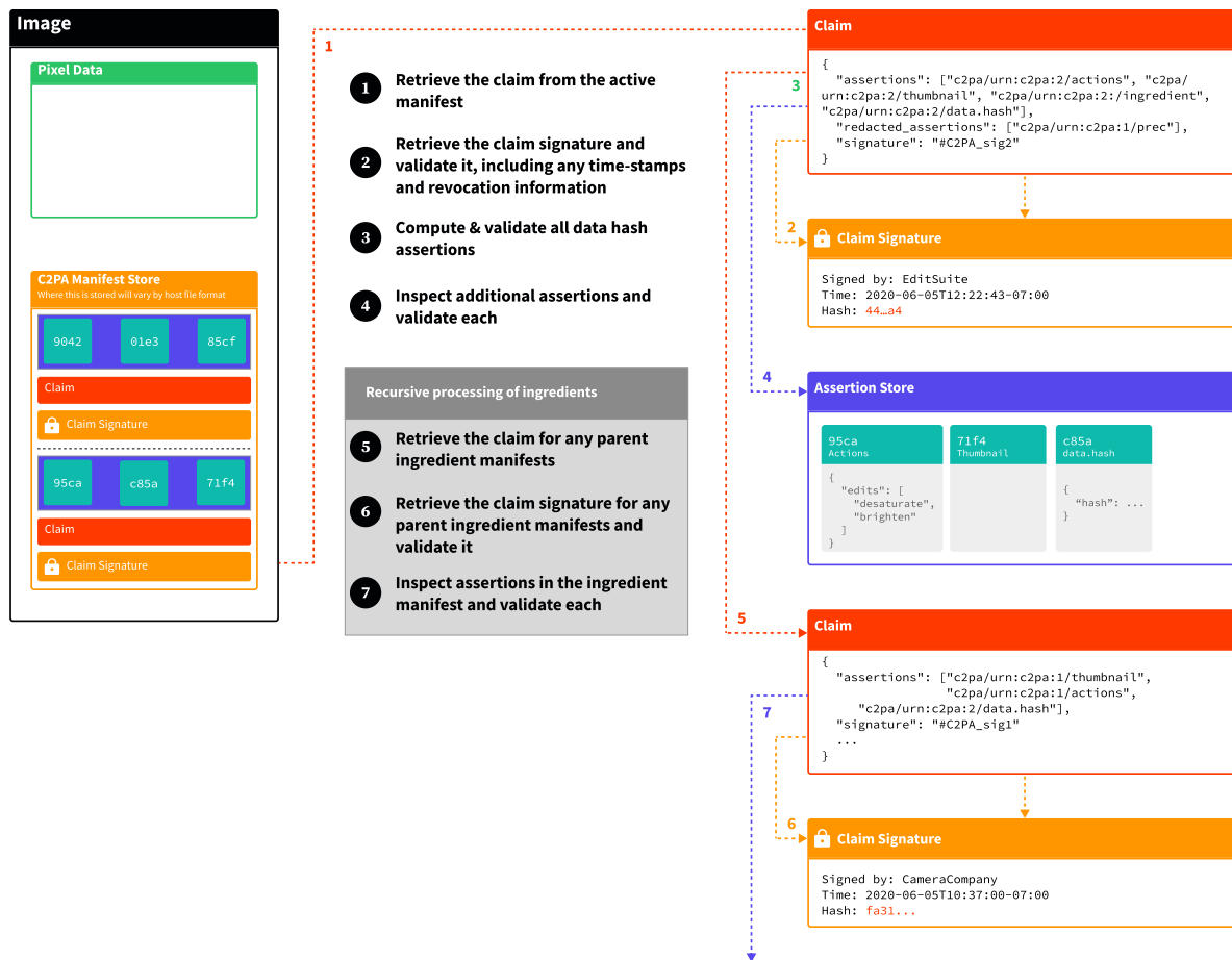
Figure 12. Validating a Claim
