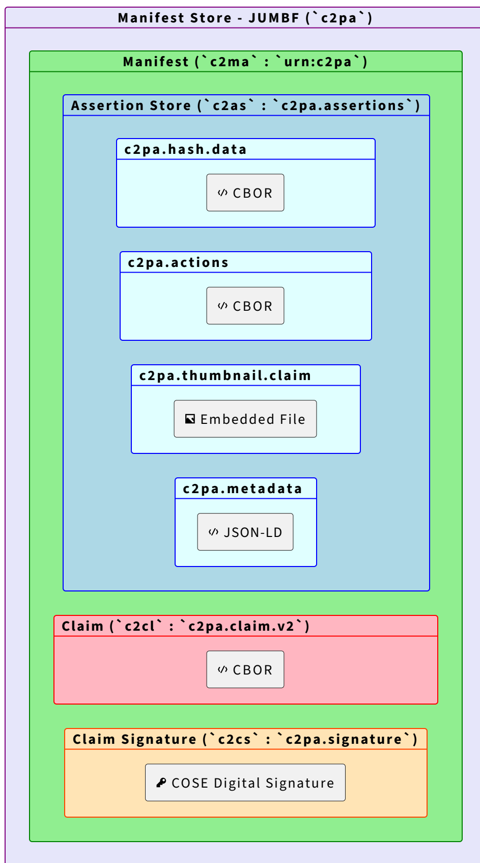
Figure 8. C2PA Manifest Store
