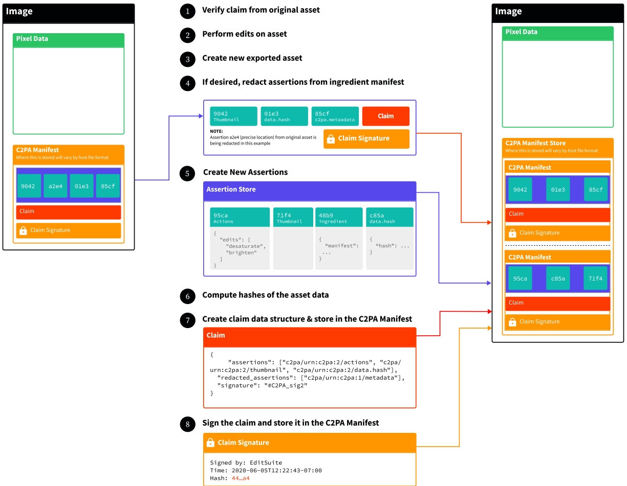
Figure 7. Redacting assertions in a secondary claim
