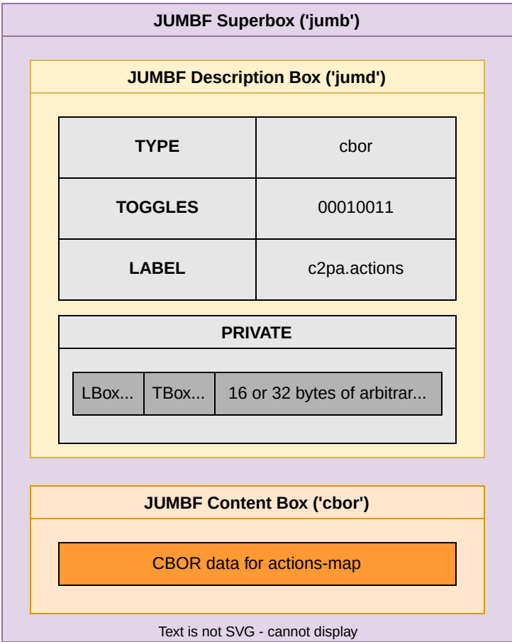
Figure 5. Example c2pa.actions assertion
