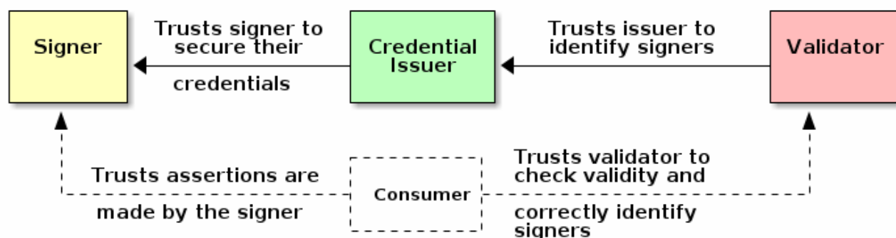
Figure 11. C2PA Trust Model Diagram
