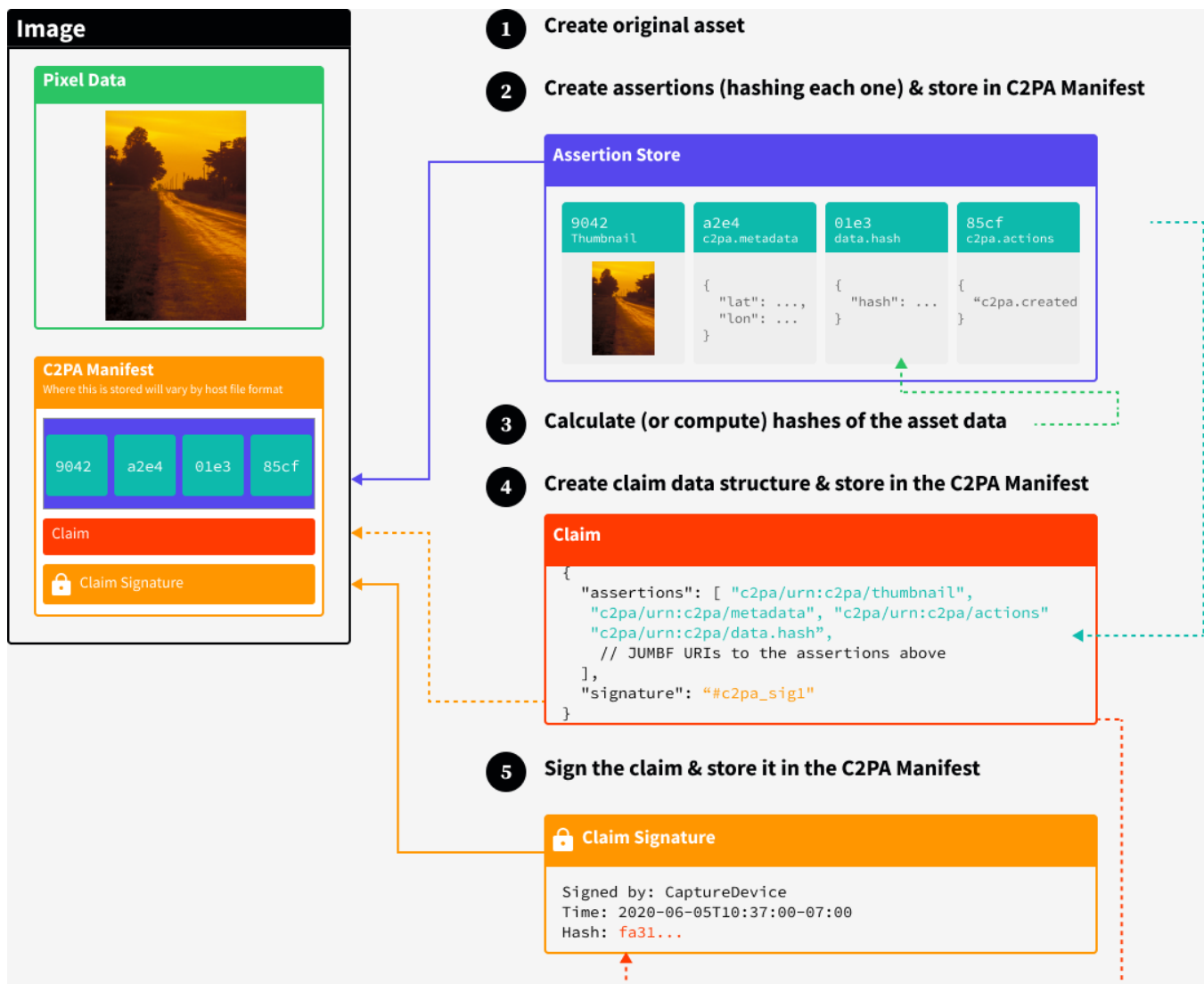
Figure 6. A single claim with assertions
