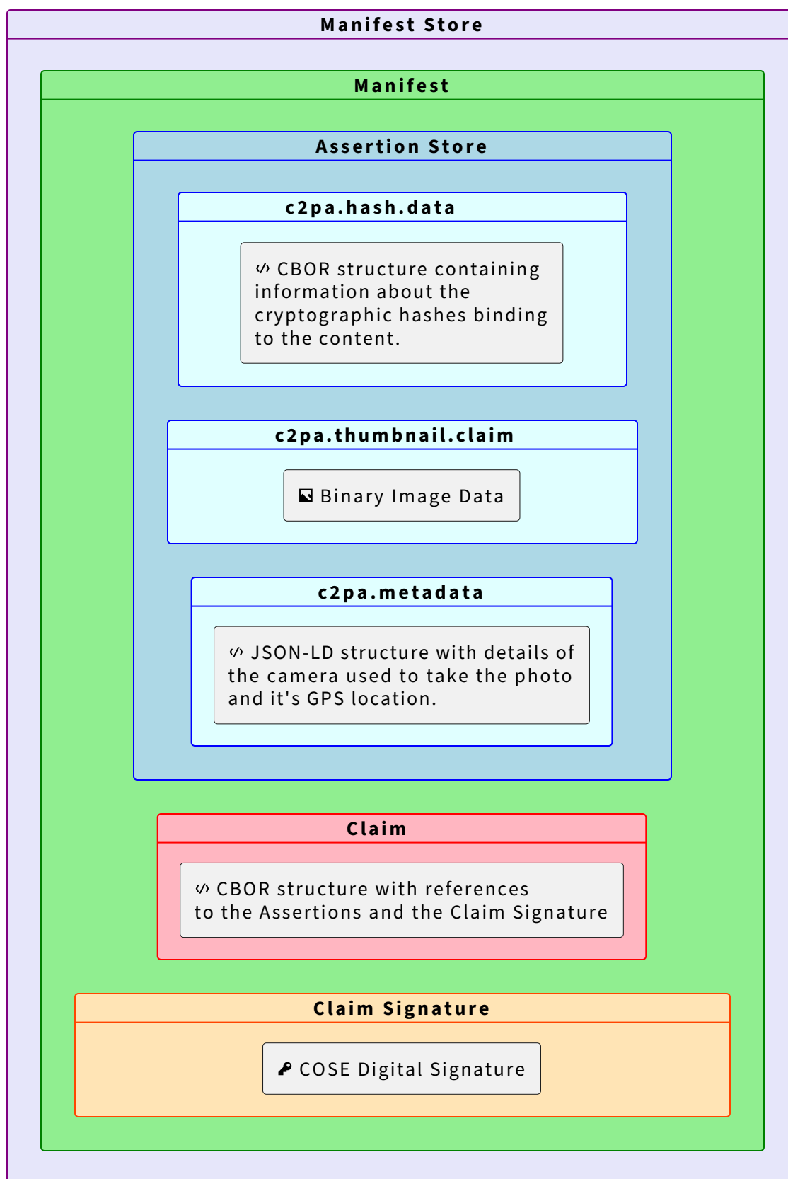
Figure 2. Example C2PA Manifest of a Photograph
