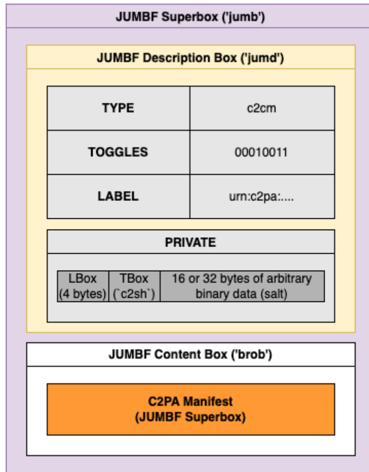
Figure 10. Example of a compressed manifest
