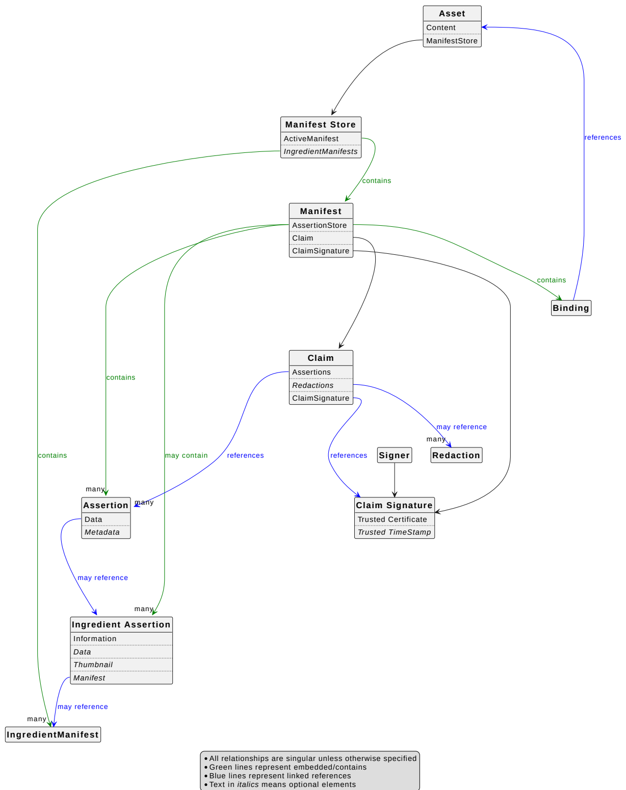
Figure 4. C2PA Entity Diagram
