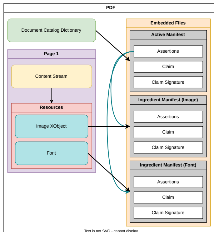
Figure 19. Example of a PDF with multiple ingredient manifests
