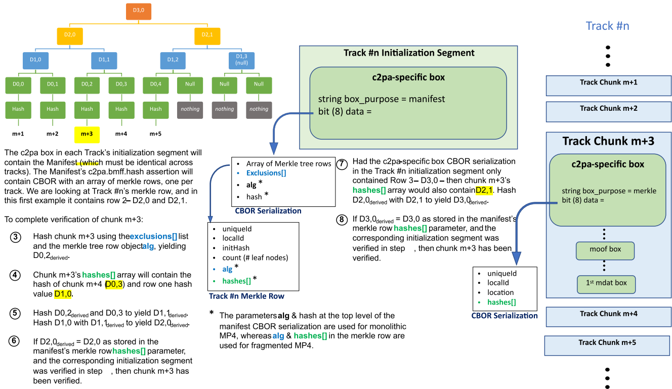
Figure 16. Validating the chunk's data
