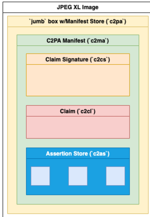
Figure 18. A C2PA Manifest embedded in a JPEG XL image
