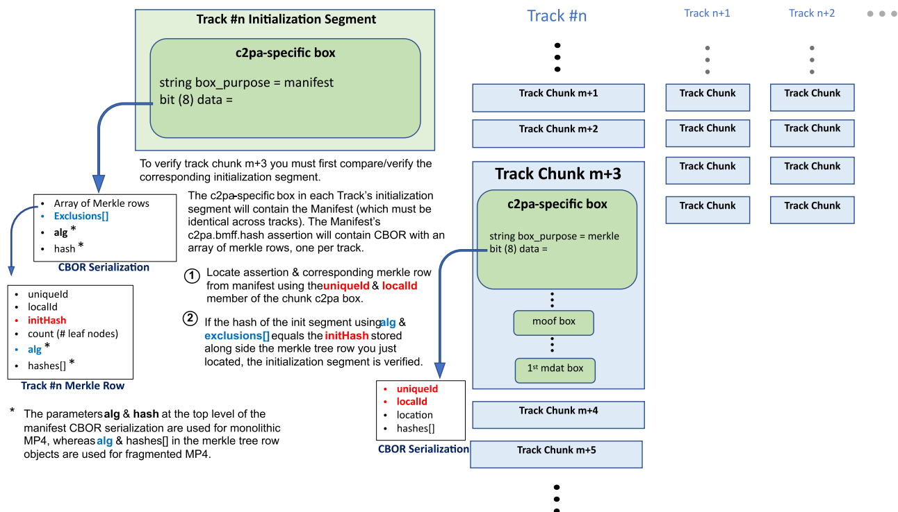
Figure 15. Validating the initialization segment
