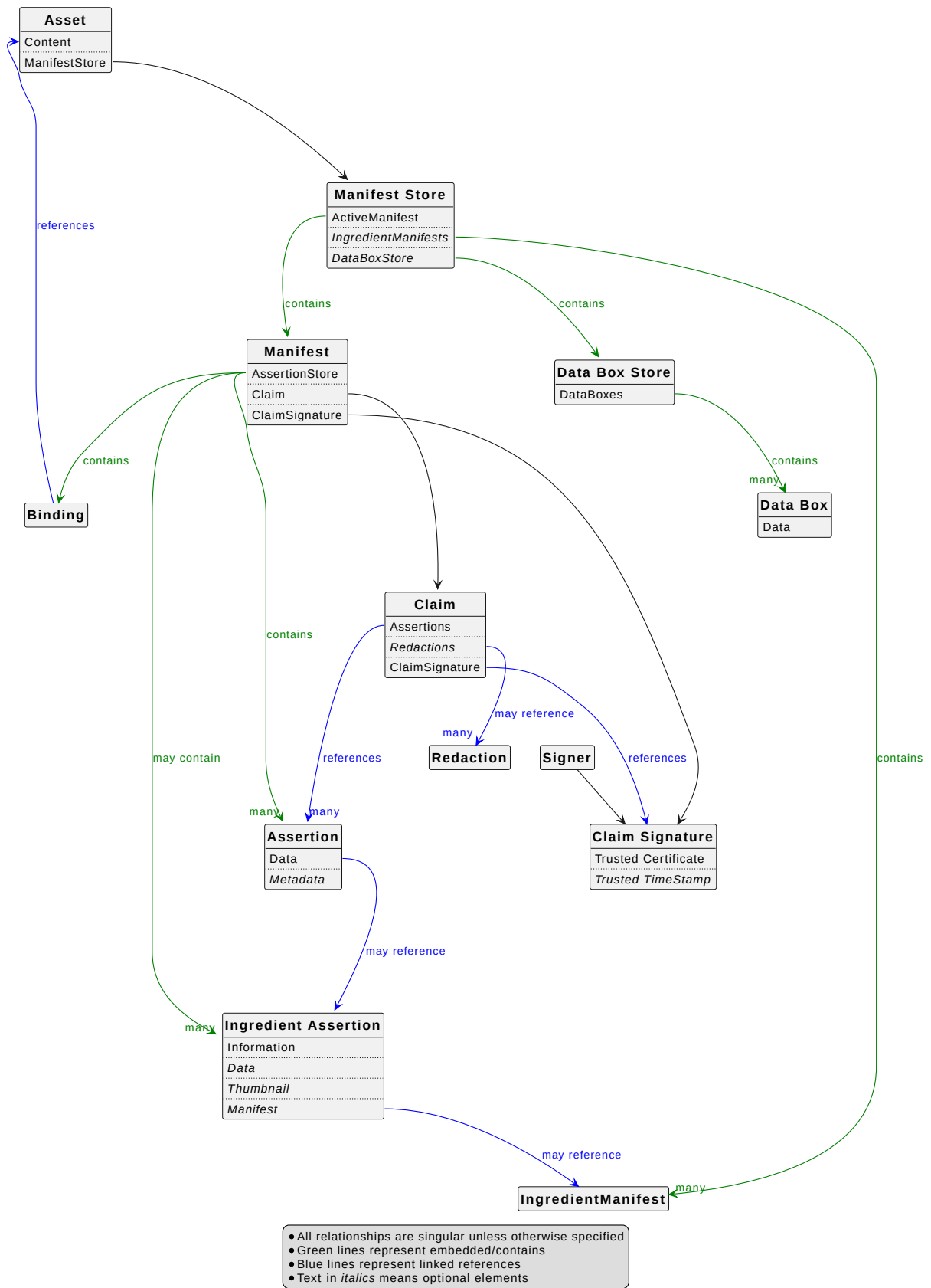
Figure 11. C2PA Entity Diagram
