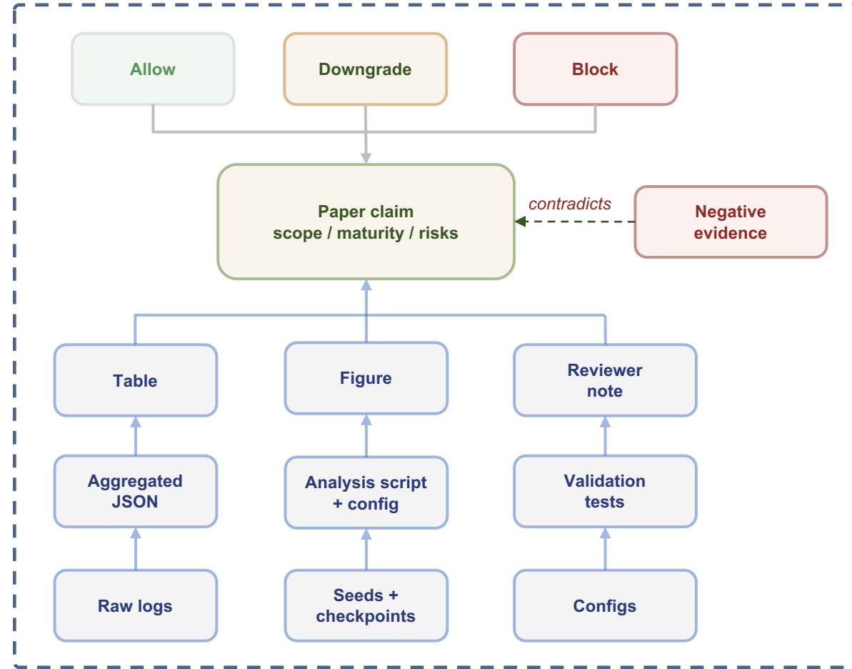
(b) Claim-evidence graph
