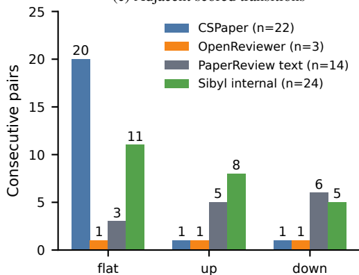
(c) Adjacent scored transitions
