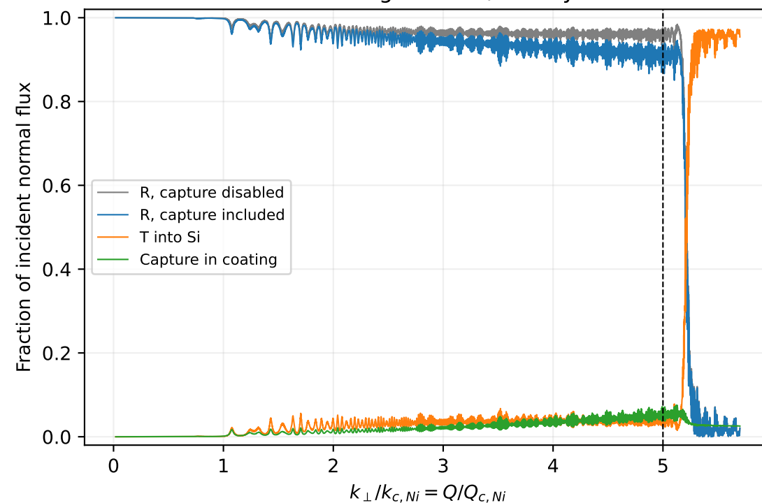
m=5: 1600 graded Ni/Ti bilayers
