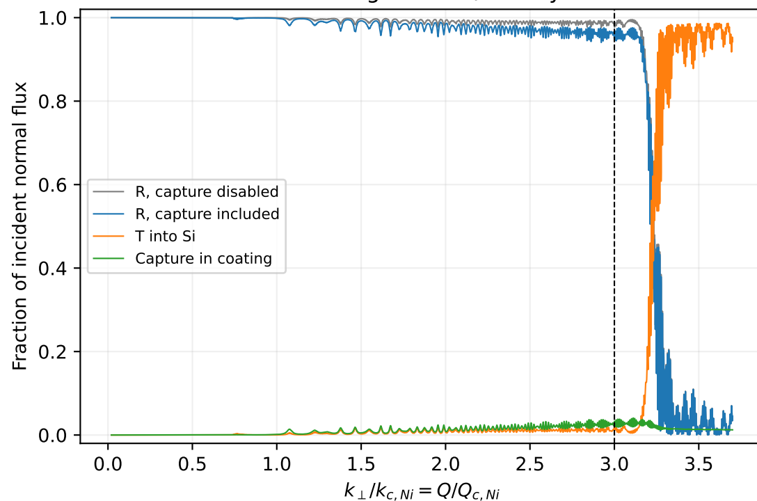
m=3: 300 graded Ni/Ti bilayers
