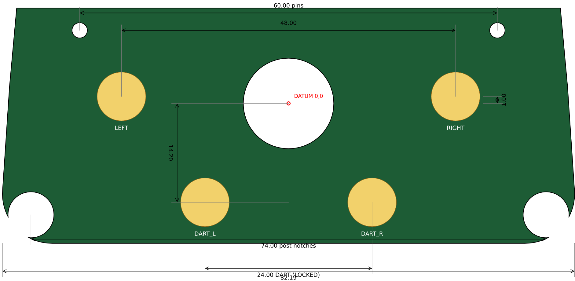
FRONT VIEW (contact side, faces the mat)
