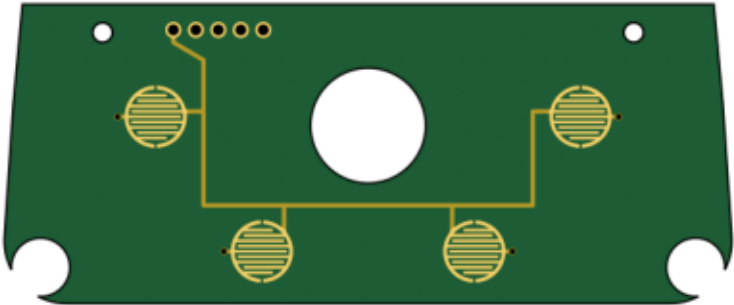
FRONT (contacts, faces the CM1 mat)
