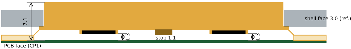
SECTION B-B DART rocker through both pills + centre stop (true scale)
