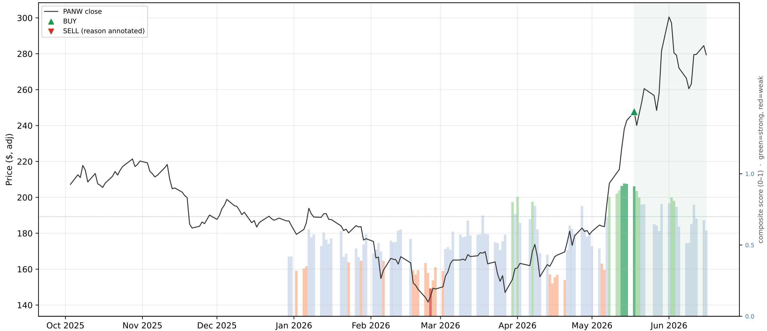
PANW — active +12.8% vs buy & hold +34.9% (active TRAILED hold; 0 round trips)
