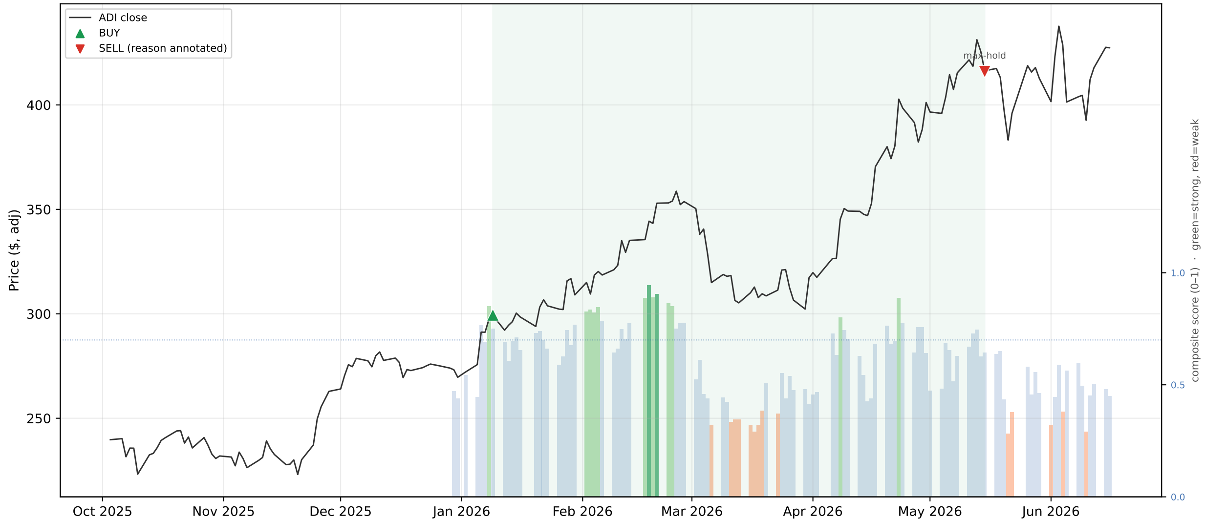
ADI — active +38.9% vs buy & hold +78.3% (active TRAILED hold; 1 round trips)
