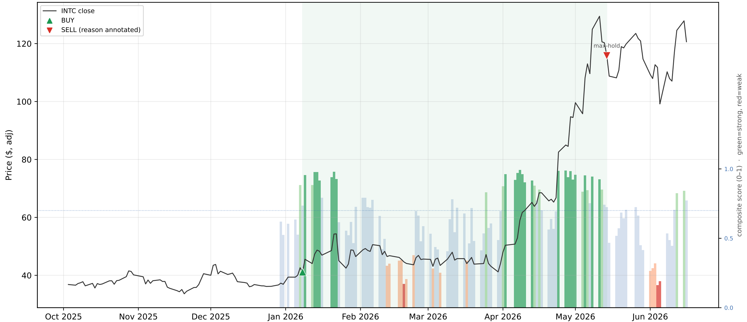
INTC — active +181.4% vs buy & hold +227.5% (active TRAILED hold; 1 round trips)
