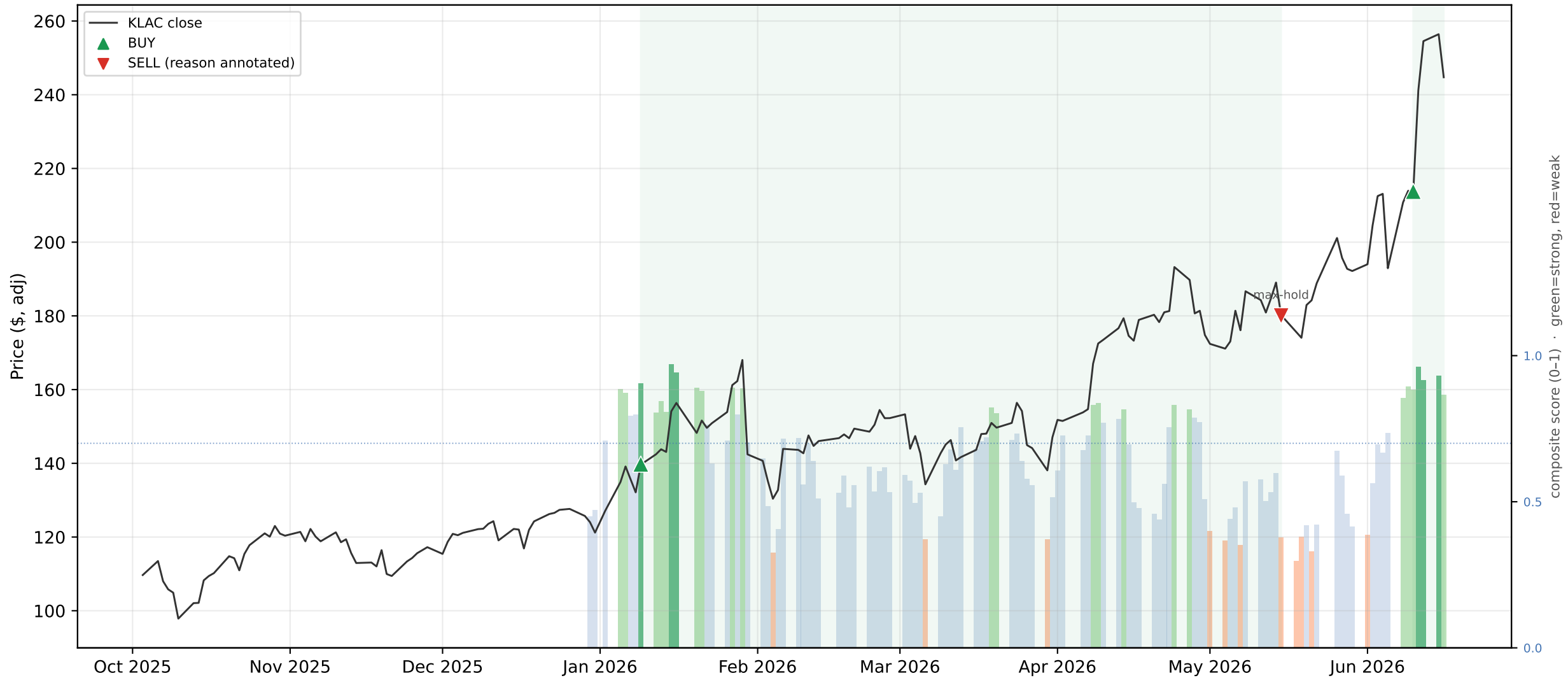
KLAC — active +47.4% vs buy & hold +123.1% (active TRAILED hold; 1 round trips)
