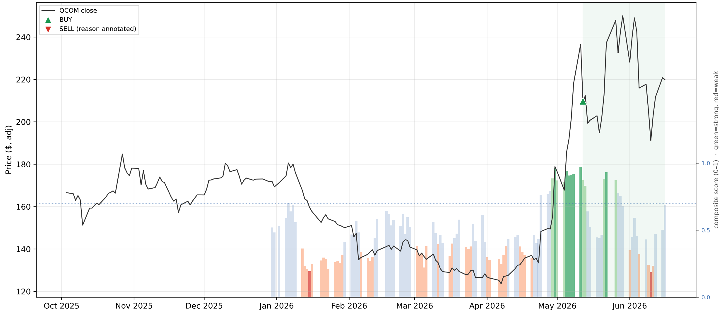
QCOM — active +4.9% vs buy & hold +32.0% (active TRAILED hold; 0 round trips)
