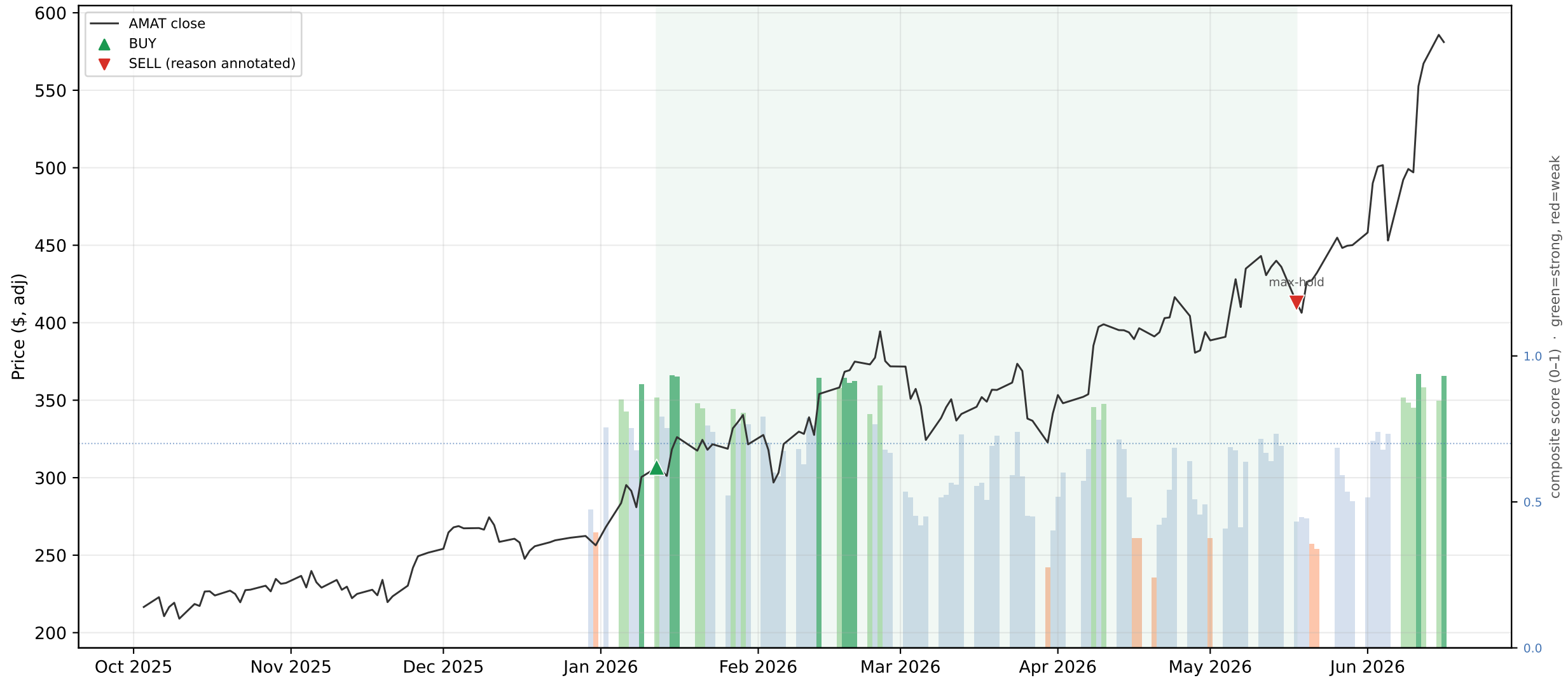
AMAT — active +34.5% vs buy & hold +168.3% (active TRAILED hold; 1 round trips)
