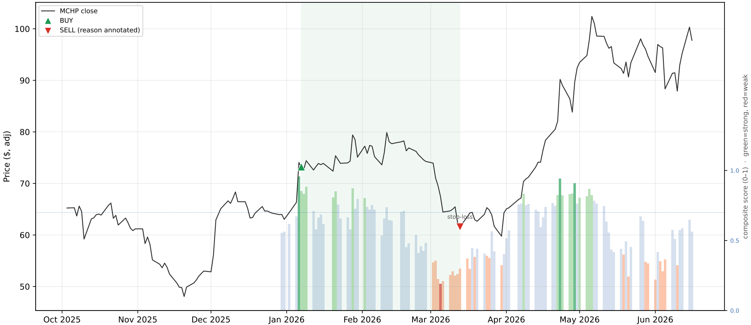
MCHP — active -15.9% vs buy & hold +49.9% (active TRAILED hold; 1 round trips)
