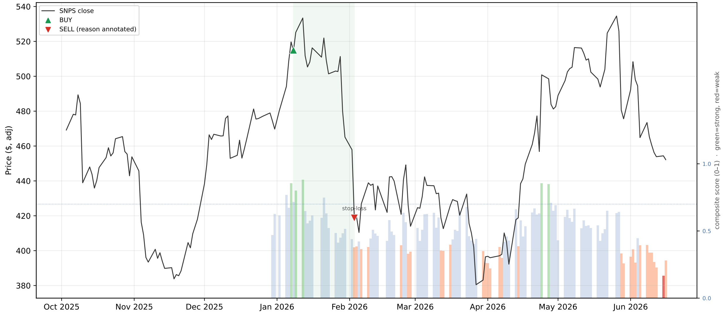
SNPS — active -18.7% vs buy & hold -3.6% (active TRAILED hold; 1 round trips)
