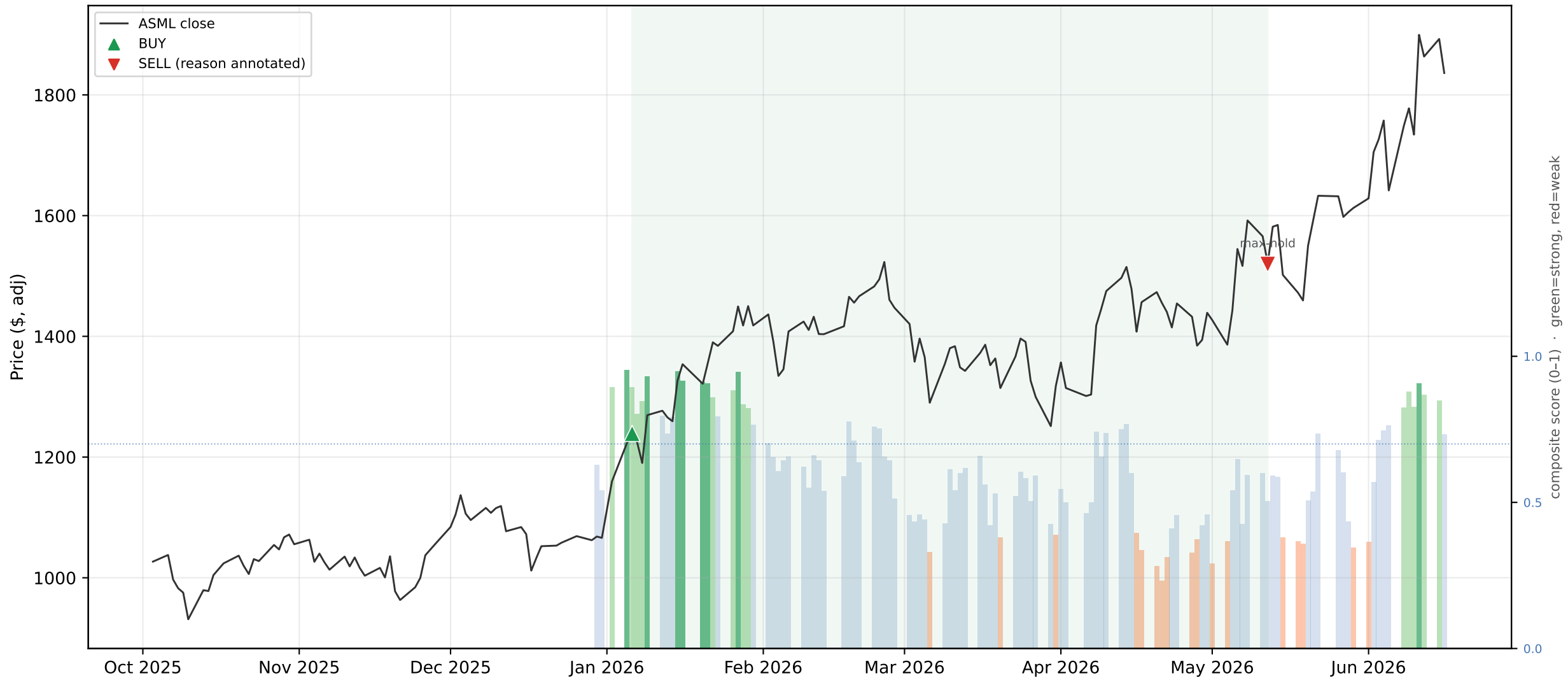
ASML — active +22.6% vs buy & hold +78.8% (active TRAILED hold; 1 round trips)
