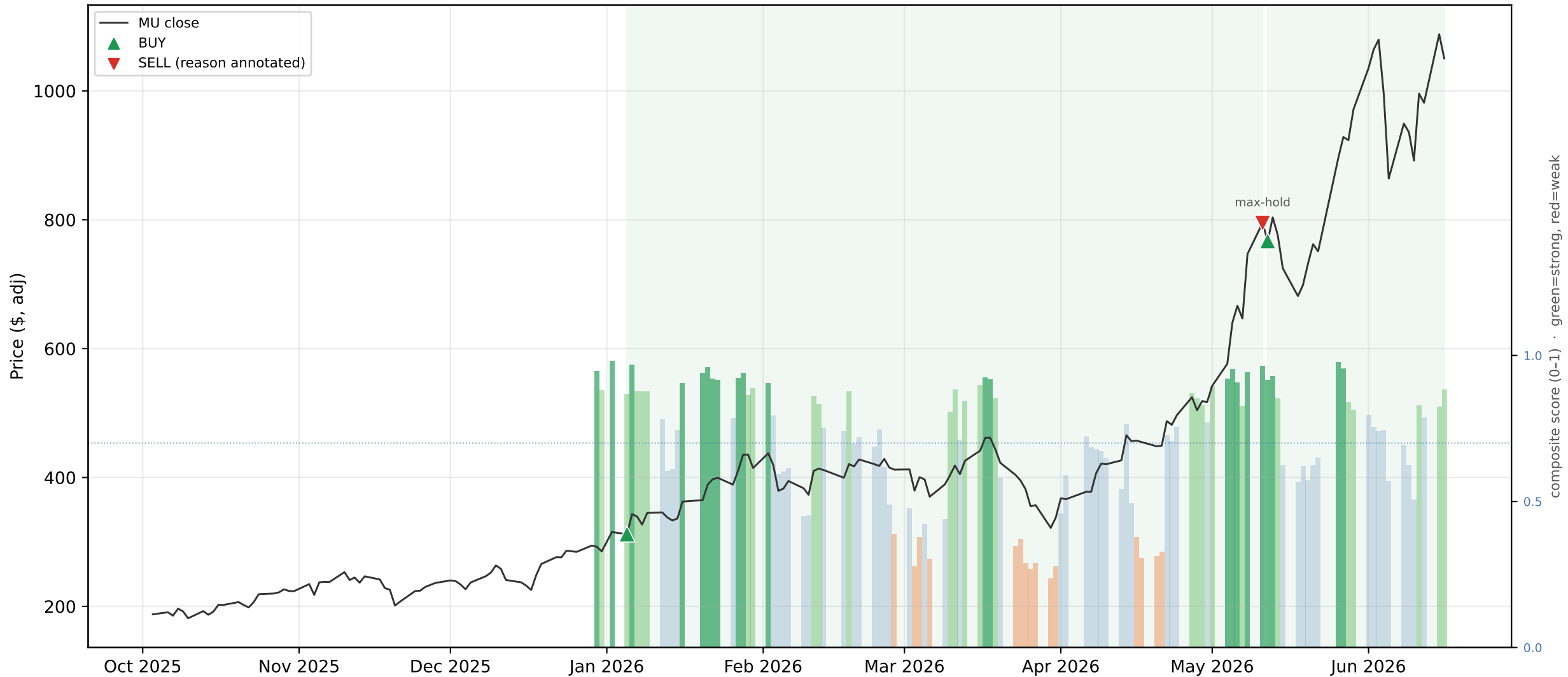
MU — active +248.2% vs buy & hold +459.7% (active TRAILED hold; 1 round trips)
