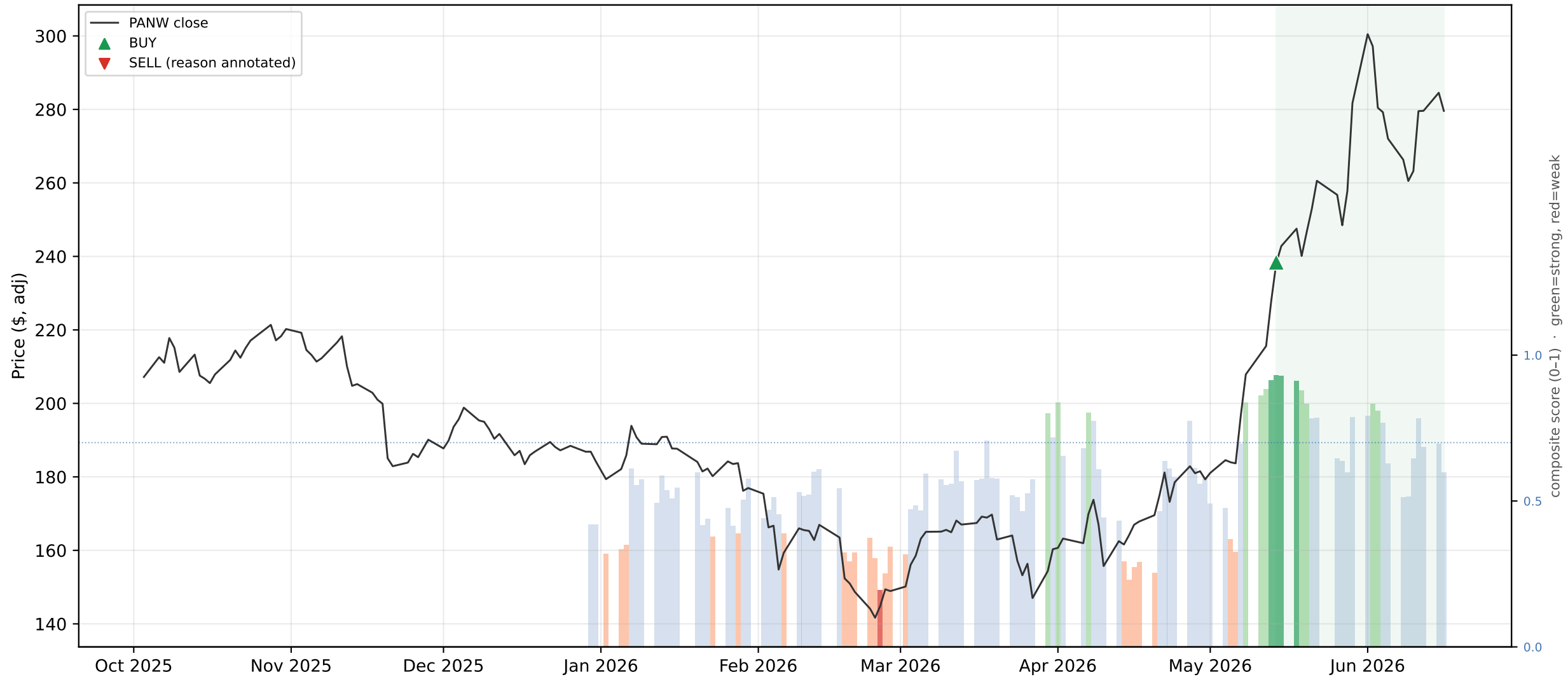
PANW — active +17.3% vs buy & hold +34.9% (active TRAILED hold; 0 round trips)
