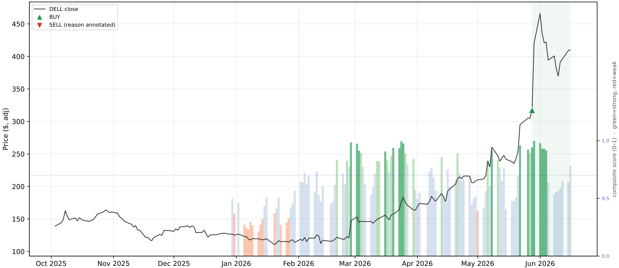
DELL — active +29.2% vs buy & hold +194.6% (active TRAILED hold; 0 round trips)
