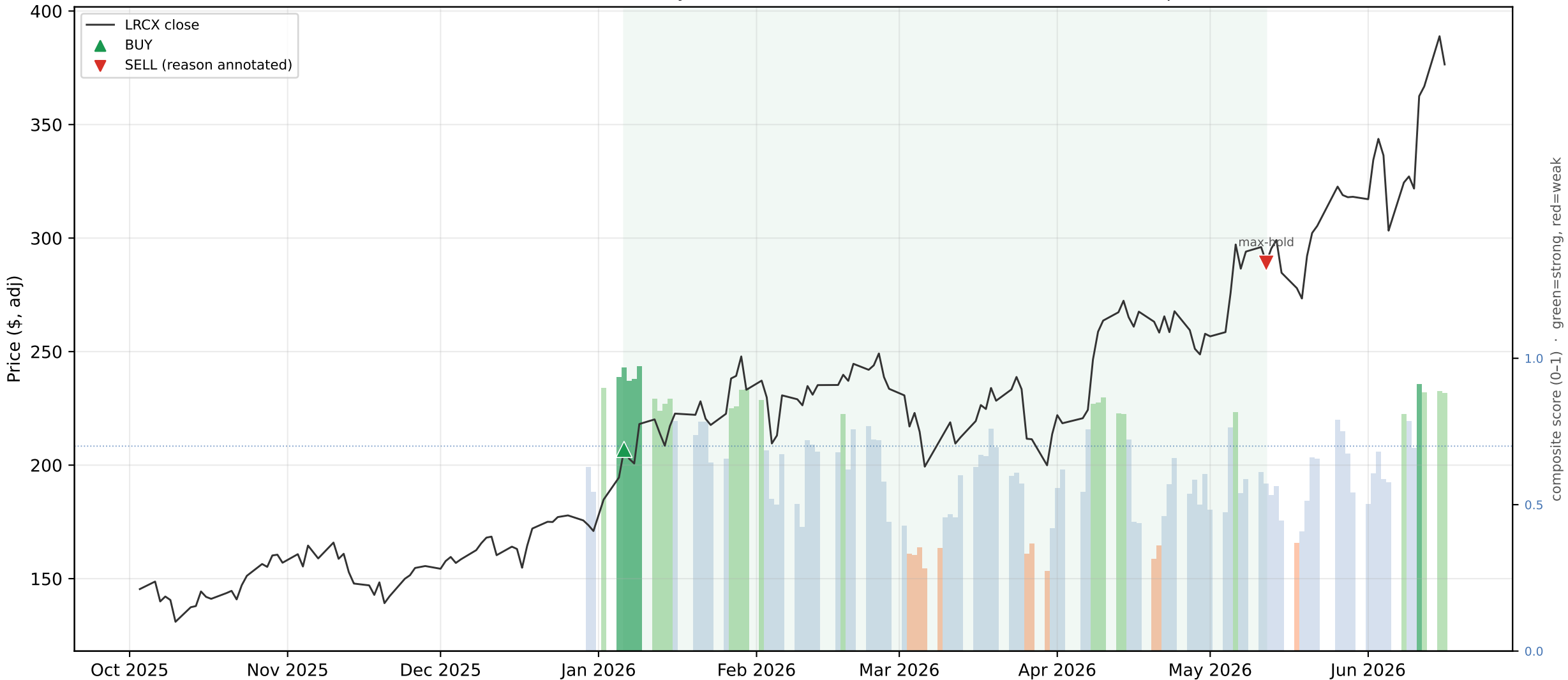
LRCX — active +39.6% vs buy & hold +158.9% (active TRAILED hold; 1 round trips)
