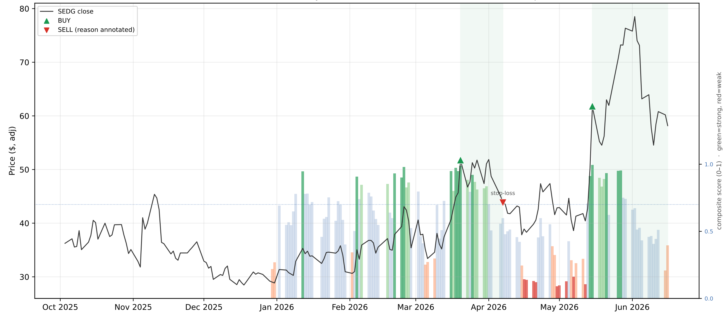
SEDG — active -20.4% vs buy & hold +60.5% (active TRAILED hold; 1 round trips)
