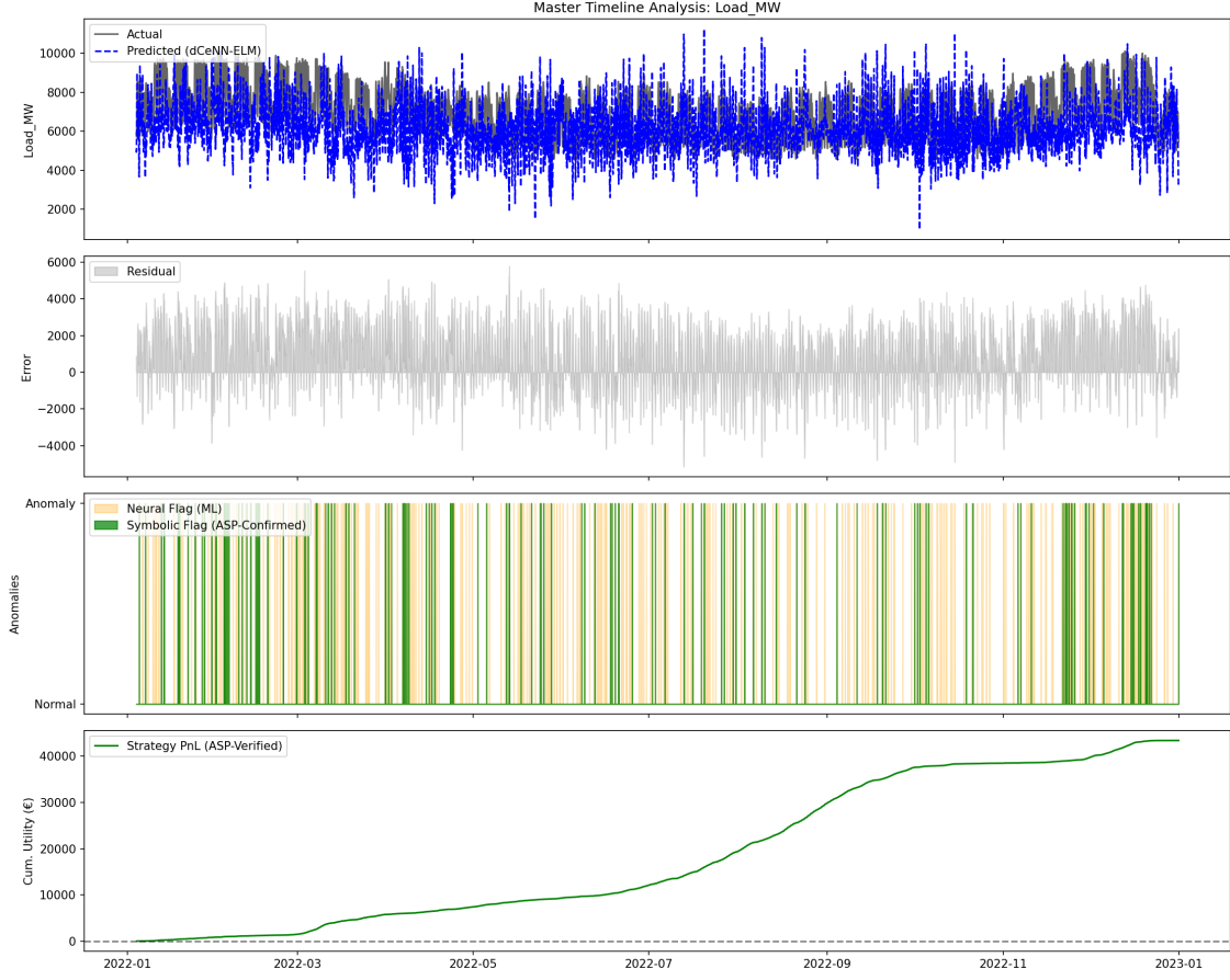
Figure 7.2: Master timeline for the Load_MW target over the 2022 test period, illustrating the temporal evolution of actual and predicted load, residual behaviour, and the corresponding anomaly-flag structure used in the downstream neuro-symbolic analysis.
