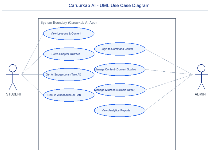
Figure: UML Use Case Diagram
