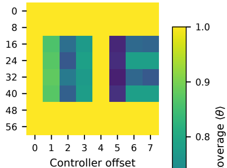
L=32, k=8, periodic
