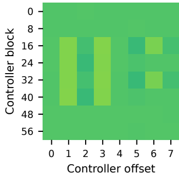
L=32, k=2, periodic
