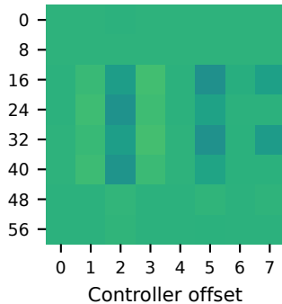
L=32, k=3, periodic
