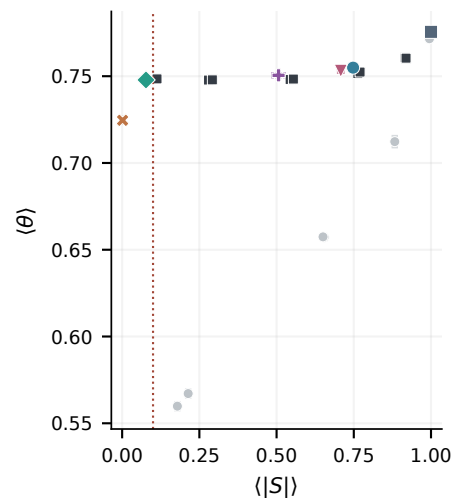
L=64, k=8, periodic
