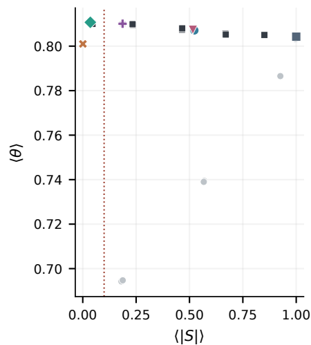
L=64, k=4, periodic
