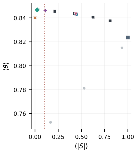
L=64, k=3, periodic
