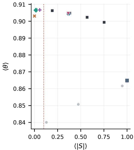
L=64, k=2, periodic
