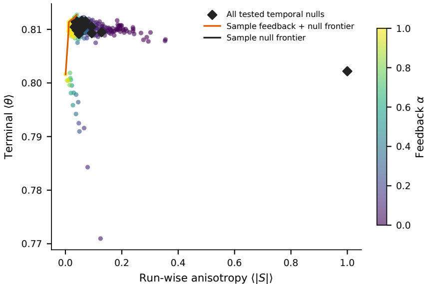
exploration-combined: L=64, k=4, periodic
