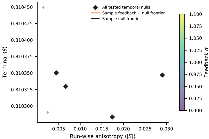
confirmation_stability: L=512, k=4, periodic
