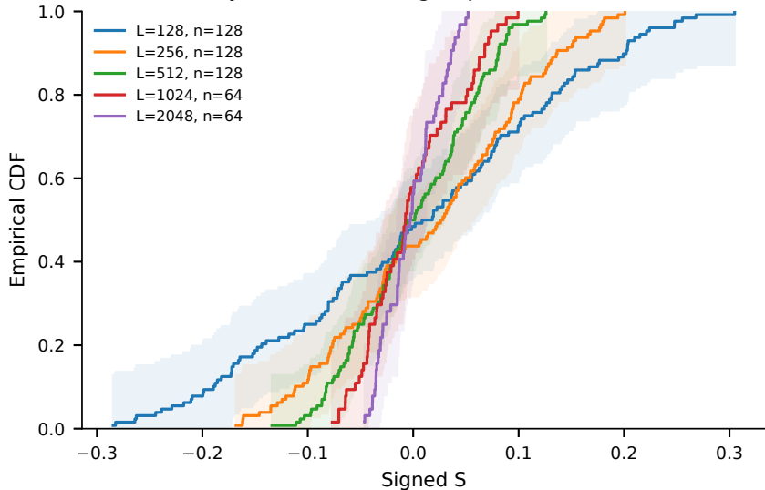
Policy41: k=4; within-group 95% DKW bands
