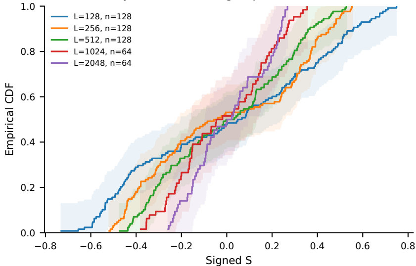
Policy41: k=8; within-group 95% DKW bands
