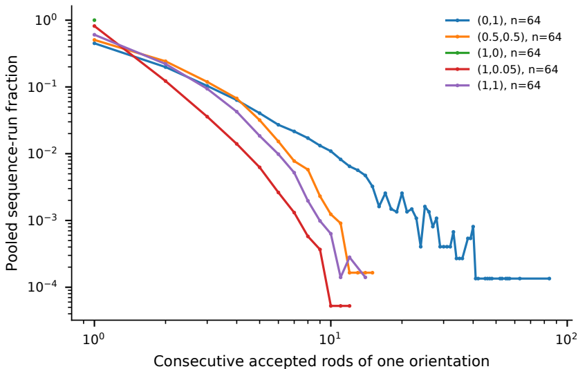
landscape: L=64 , k=8 , periodic
