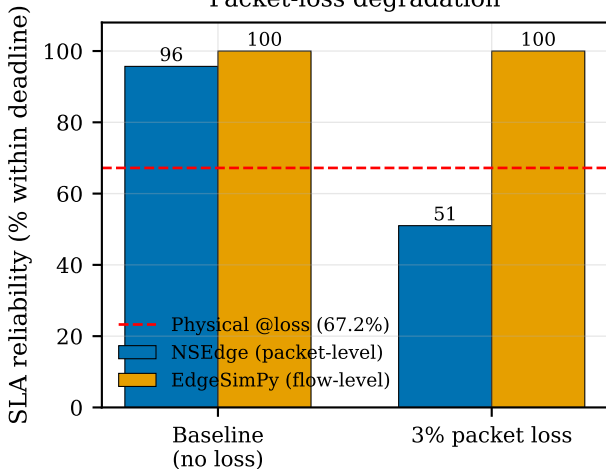
Packet-loss degradation
